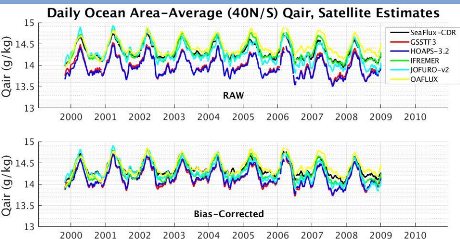
Area-average time series of Qair are shown for 6 different satellite-derived estimates for both raw (top) and bias-corrected fields over the common observing period 1999-2008. Note how the state-dependent bias correction results in more consistent — and presumably more accurate with reference to VOS — surface estimates across the products.
