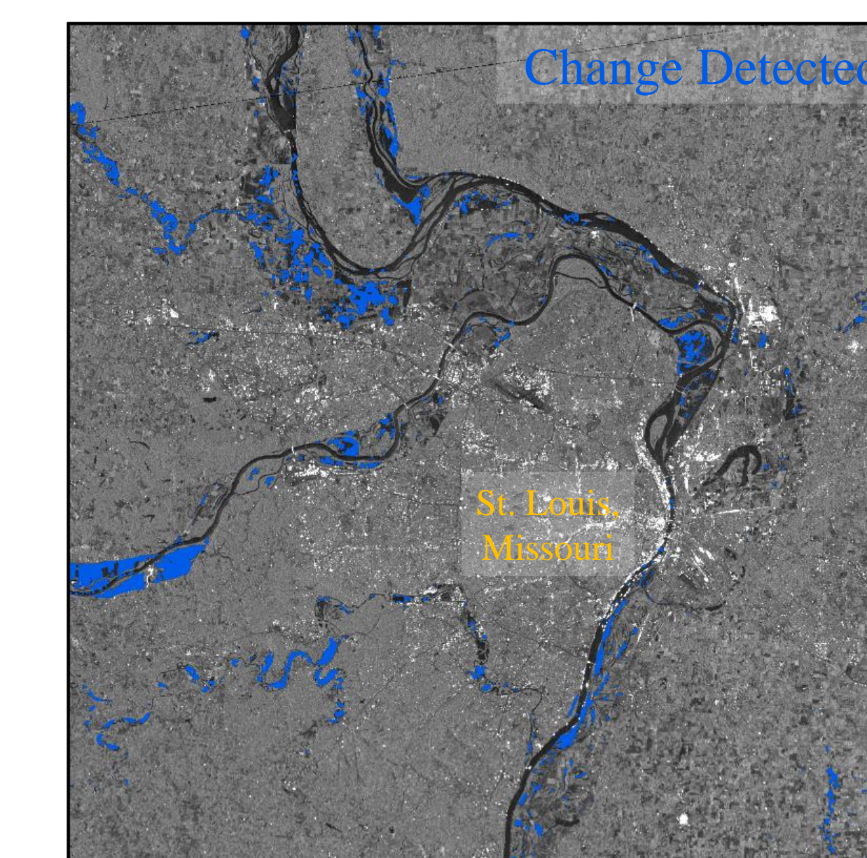
Figure 7. Using data from a before (Fig. 5) and after (Fig. 6), ASF has developed a change detection tool for HyP3 which identifies areas of significant change (flooding) between the two scenes.
