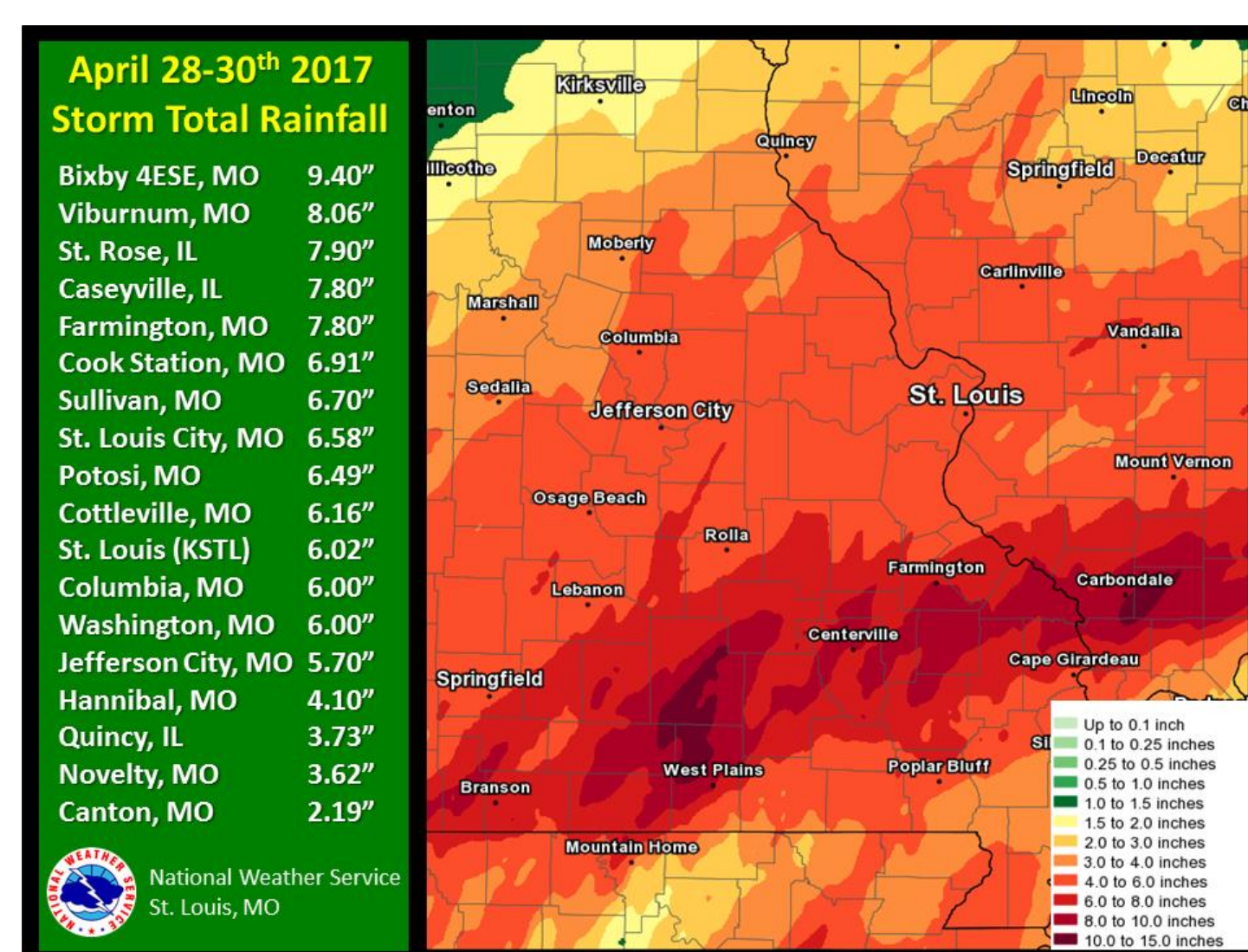
Figure 2. Three day rainfall totals across portions of Missouri that caused widespread flooding. Image is courtesy of the NOAA/National Weather Service-St. Louis.
