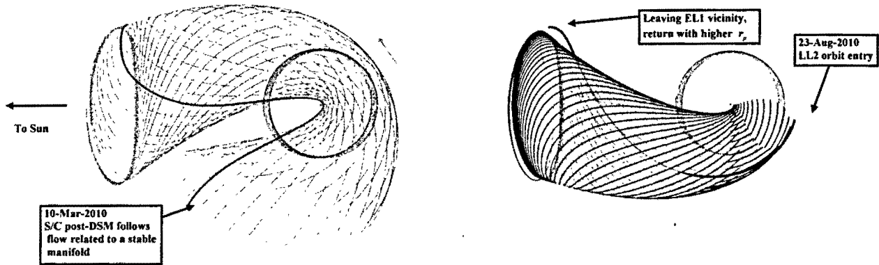
Figure 4. Baseline P1 Out-Bound to Max Radius on Stable Manifold and In-Bound to Lissajous Orbit on Unstable Manifold
