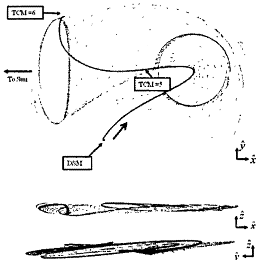
Figure 9. P1 Planned Stable Sun-Earth Manifold
