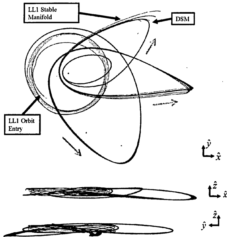
Figure 13. P2 Manifold
