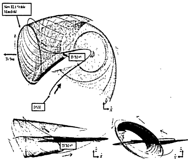
Figure 10. P1 Pre and Post TCM5 Stable Sun-Earth Manifold
