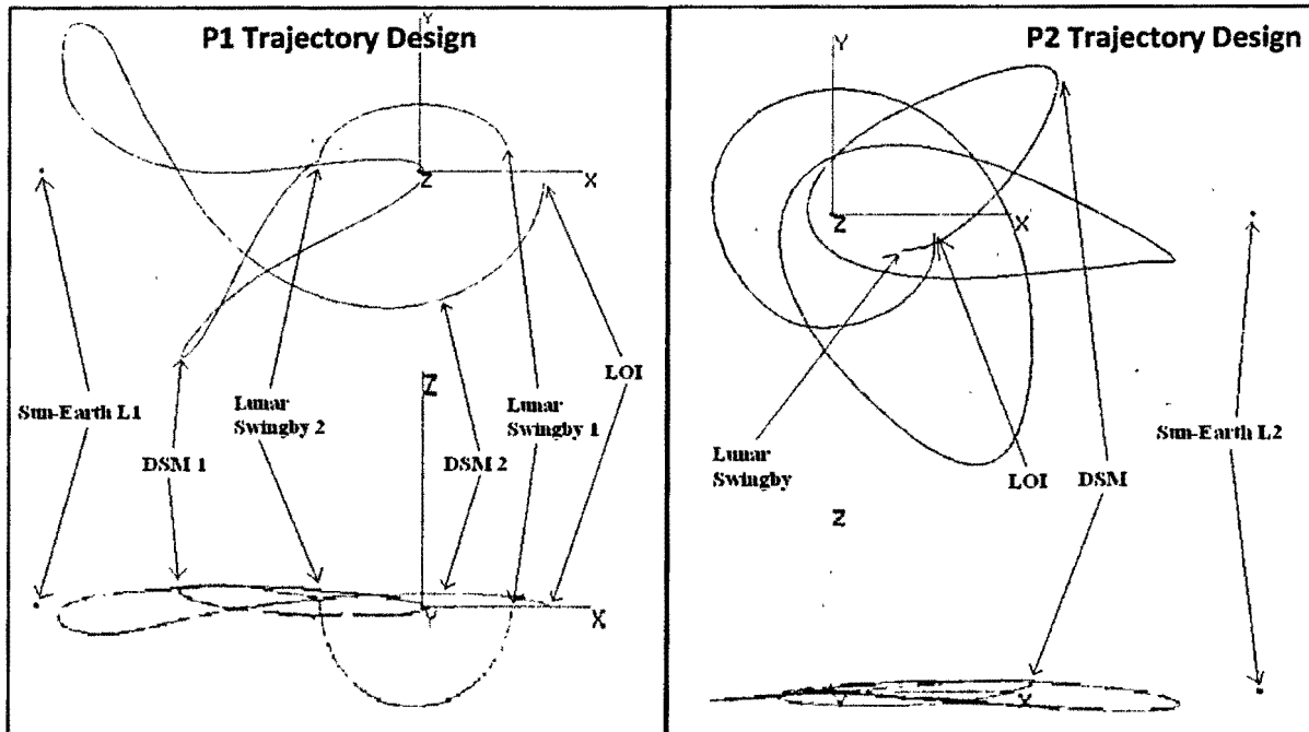
Figure 2. ARTEMIS P1 Trajectory Design
