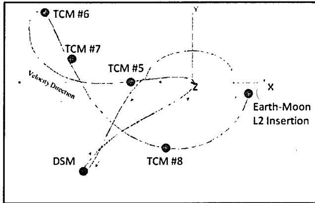
Figure 5. P1 Maneuver Locations
