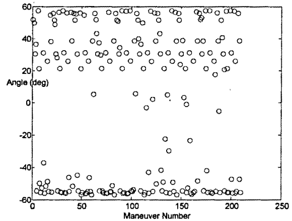
Figure 9. Angle Between X-axis and DV Vector for Maneuvers at Each X-axis Crossing.
