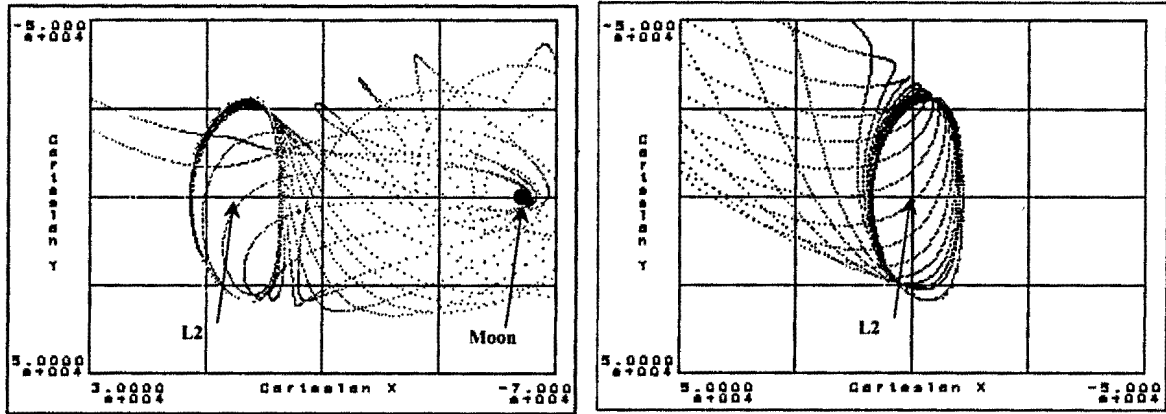
Figure 5. L_2 Trajectories and Arcs along the Unstable Modes.
