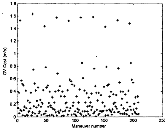
Figure 8. DVs for Maneuvers at Each X-axis Crossing.
