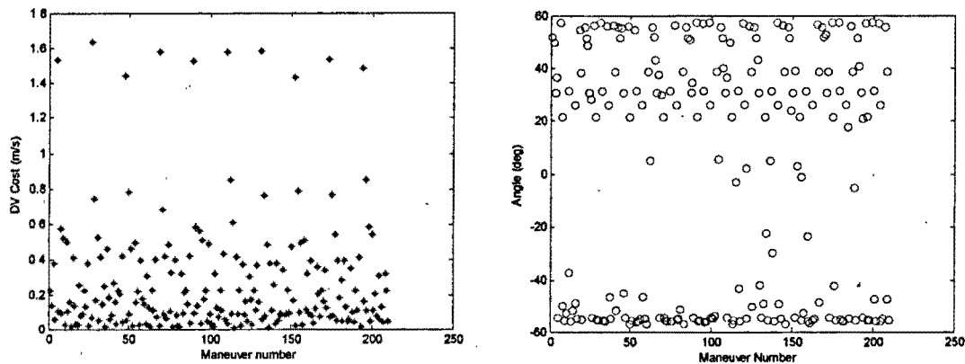
Figure 10. DVs of Maneuvers at 3.8-day intervals. Figure 11. Angles between X-axis and DV Vector.
