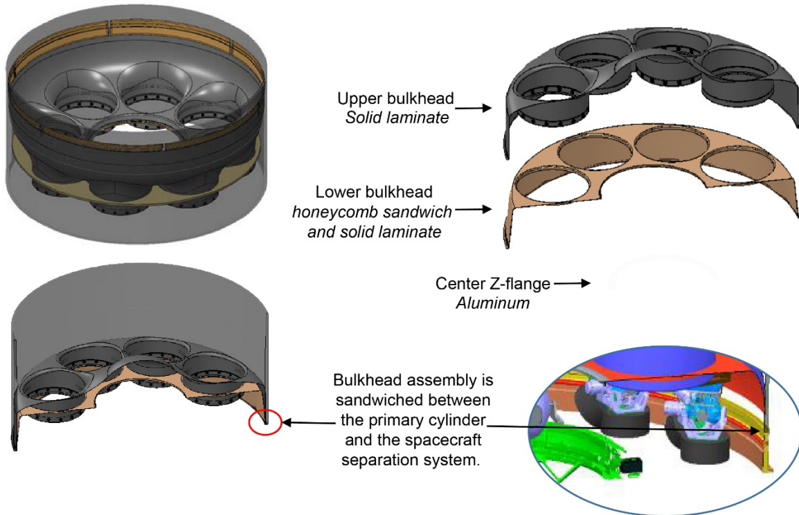
Figure 9.—Sombbrero bulkhead.
