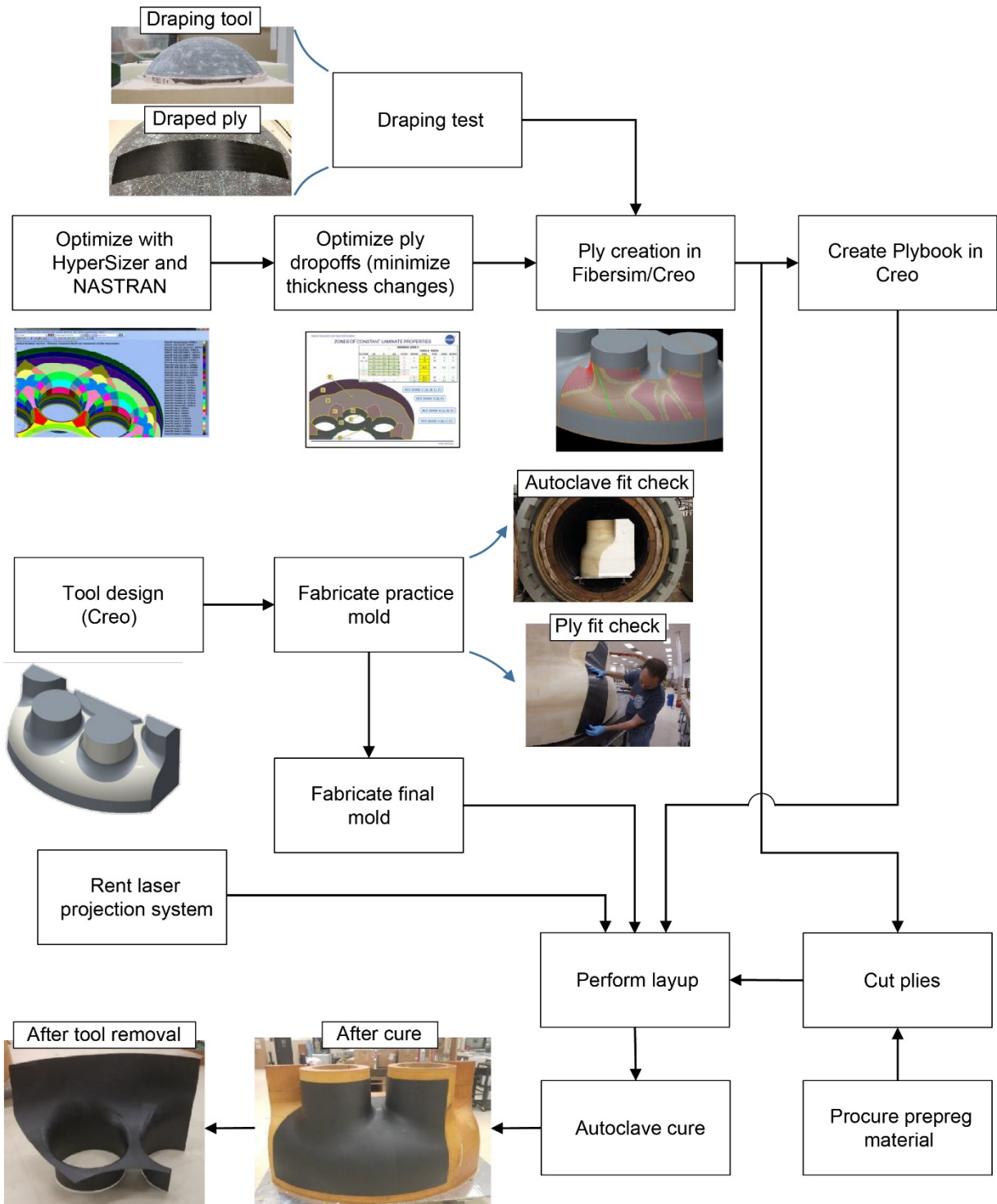
Figure 19.—Engineering demonstration unit (EDU) NASA Structural Analysis (NASTRAN).
