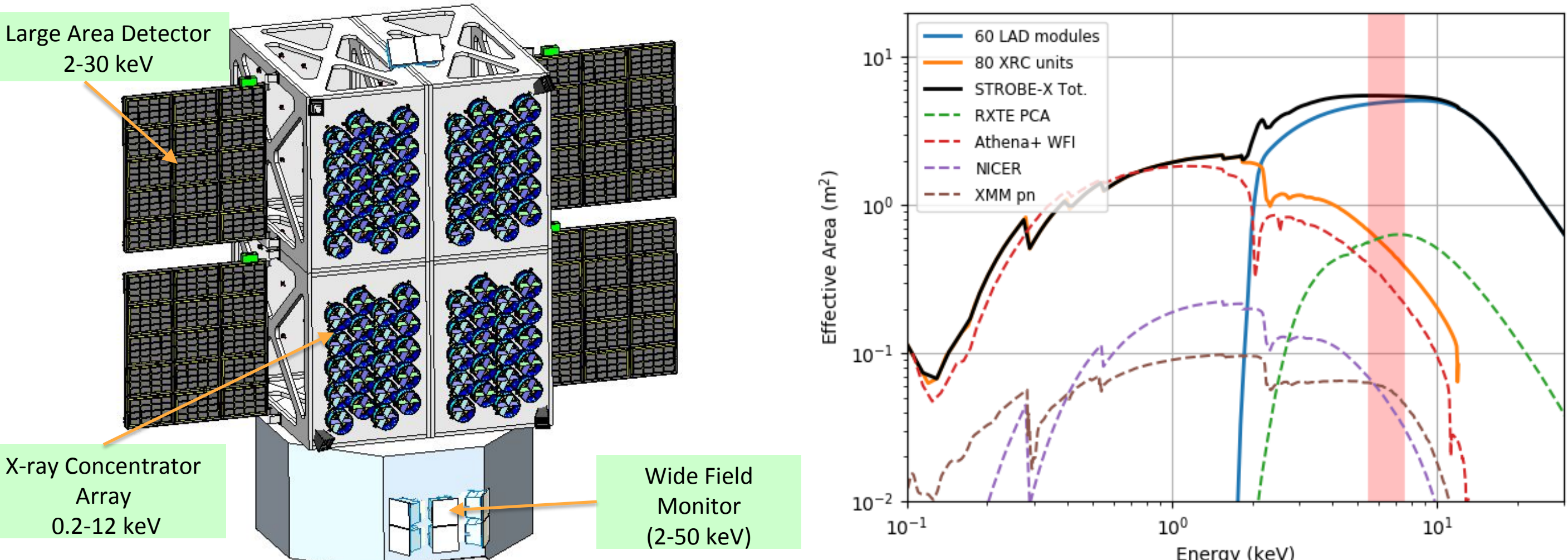
Figure 1: (Left) Notional deployed configuration of the STROBE-X spacecraft. (Right) Effective area for the current baseline configuration of 60 Large Area Detector (LAD) modules and 80 X-ray Concentrator (XRC) units. This configuration has ~5.5m² of effective area in the critical iron line region.
