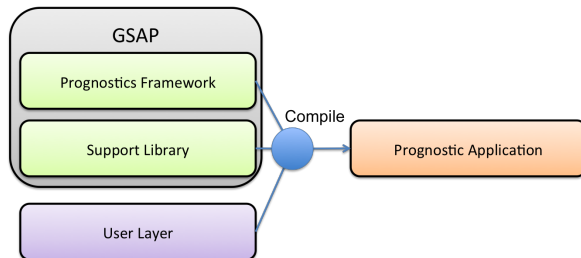
Figure 2. Using GSAP
