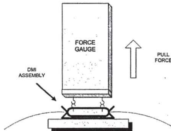
Figure 13; Pull test set up for measuring the pull force necessary to disengage the cylinder from the retention clip in the standard and rugged DMI (Mini AVIM).
