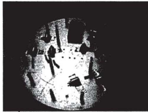
Figure 10 a) Cryogenic testing equipment set up for evaluation of optical terminations and processes, b) Top view inside of cyro chamber, optical assemblies on thermal control heat plate sitting on top of the chamber cold plate.
