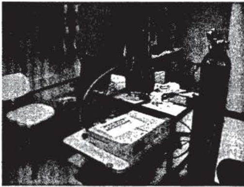
Figure 10 a) Cryogenic testing equipment set up for evaluation of optical terminations and processes, b) Top view inside of cyro chamber, optical assemblies on thermal control heat plate sitting on top of the chamber cold plate.
