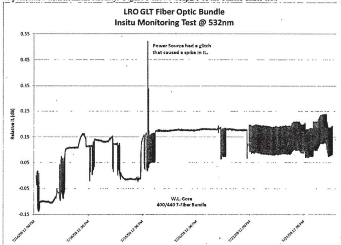
Figure 3; Graph 1 of the In-situ Insertion Loss for the Laser Ranging Bundle During the LRO Gimbal Lifetest.
