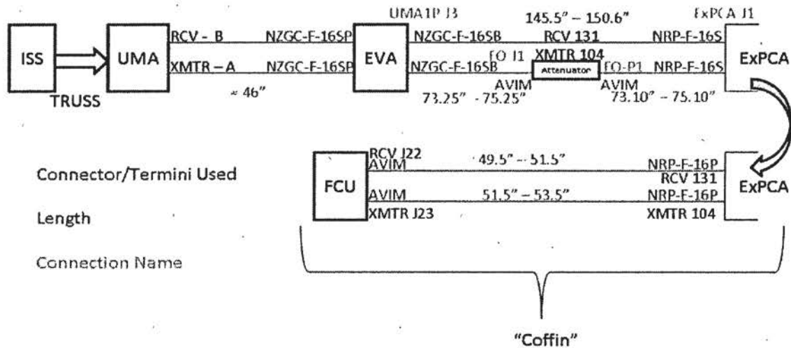
Figure 7: Express Logistics Carrier Harness Flow Map
