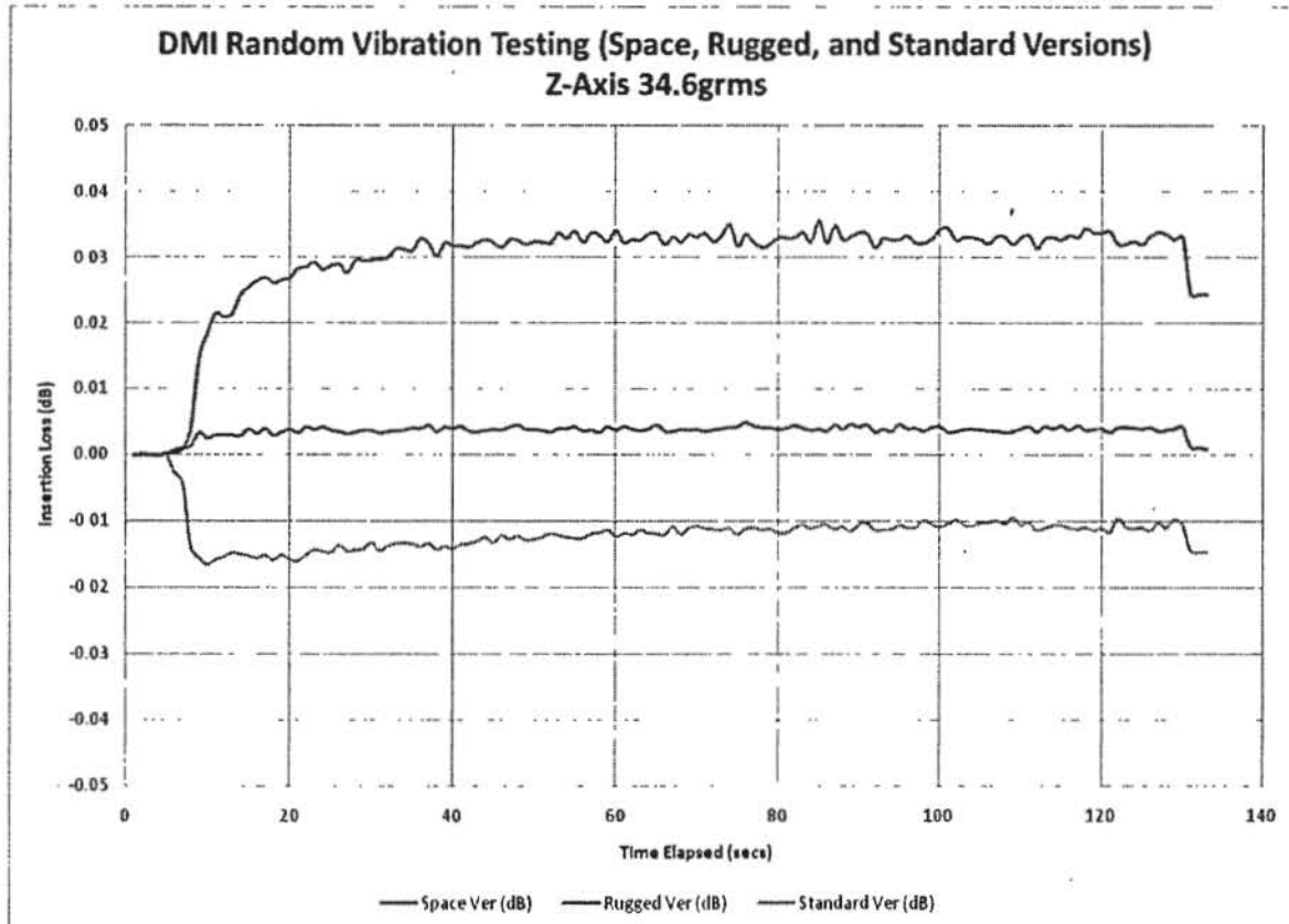
Figure 18: Example of the Mini AVIM/DMI Random Vibration Test Data.
