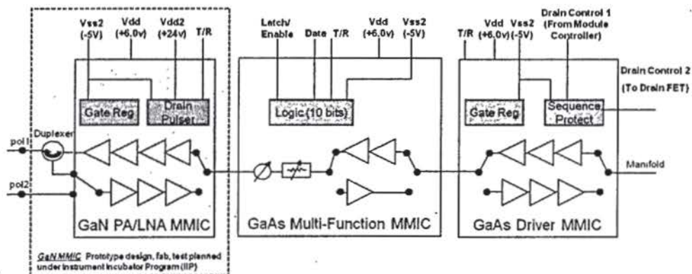
Fig. 3. Ka-band T/R module has switchable polarization on Rx and efficient GaN PA/LNA MMICs.
