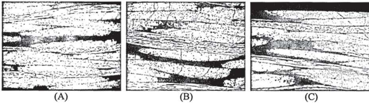
Figure 14. Photomicrographs of (A) the Baseline PMC and 0.5 wt % MWCNT-PETI-330 PMCs made from (B) two and (C) four day ball-milled blend.
