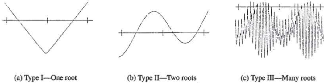
Figure 2: Types of event function behavior between ephemeris steps
