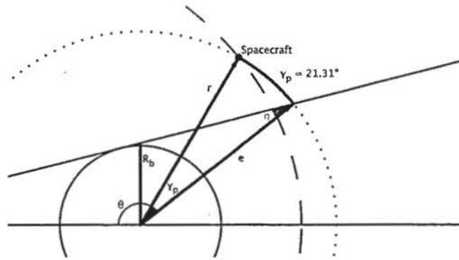
Figure 5: Penumbra event function
