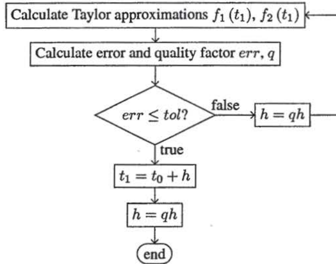
Figure 9: Adaptive stepping algorithm
