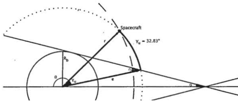
Figure 4: Umbra event function
