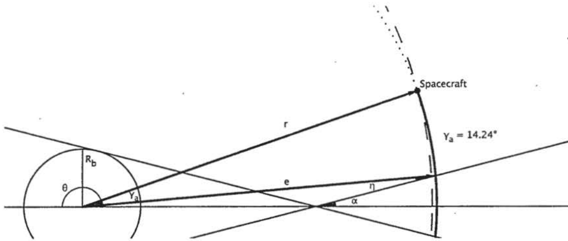
Figure 6: Antumbra event function
