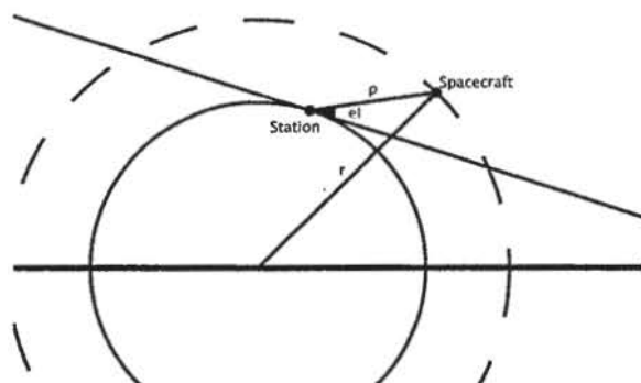
Figure 7: Elevation event function
