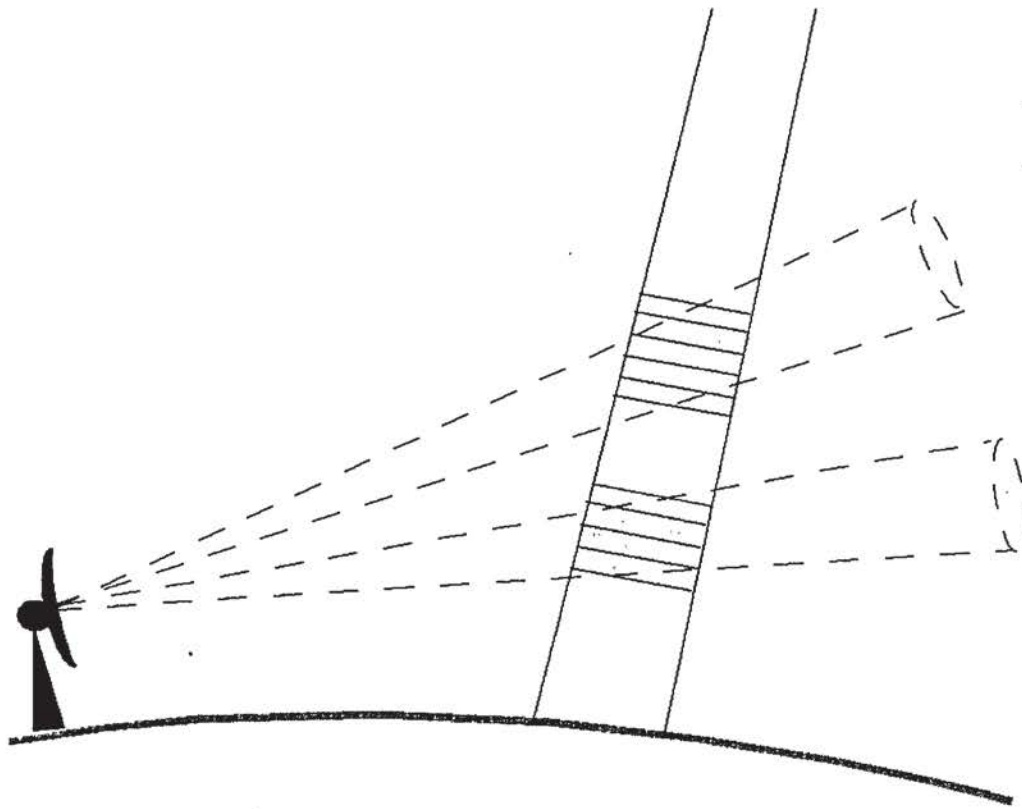
Figure 2. Schematic of PR gate averaging at GR sweep intersections. Shaded areas are PR gates intersecting two GR sweeps (dashed) at different elevation angles. Only one PR ray is shown.
