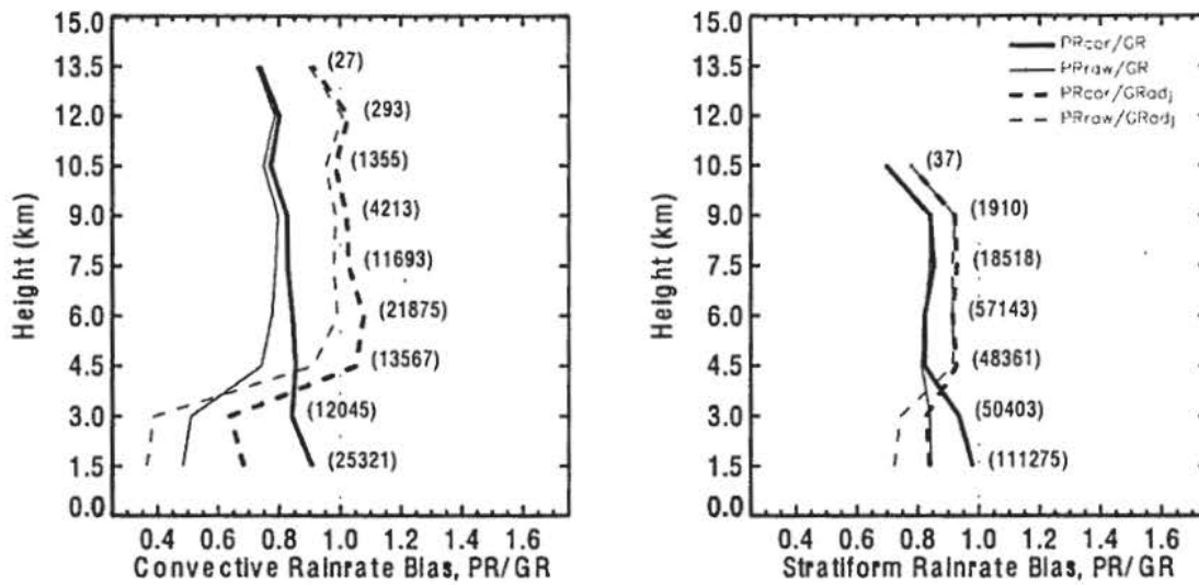
Figure 10. Vertical profiles of convective (left panel) and stratiform (right panel) mean rain rate bias (PR/GR) from volume-matched reflectivity data grouped by height, using Z=372R^{1.52} , and excluding samples affected by bright band. Heavy (narrow) lines use attenuation-corrected 2A-25 (raw 1C-21) PR reflectivity. Solid (dashed) lines use original (frequency-adjusted) GR reflectivity. Number of samples in each height layer are shown next to the profiles. No-bias (=1.0) line is shown as the light dotted line. Data for VN match-up samples measured over the NOAA WSR-88D radars identified in Figure 1 (with the exception of KGRK, see text), over the VN period of record until March 25, 2009
