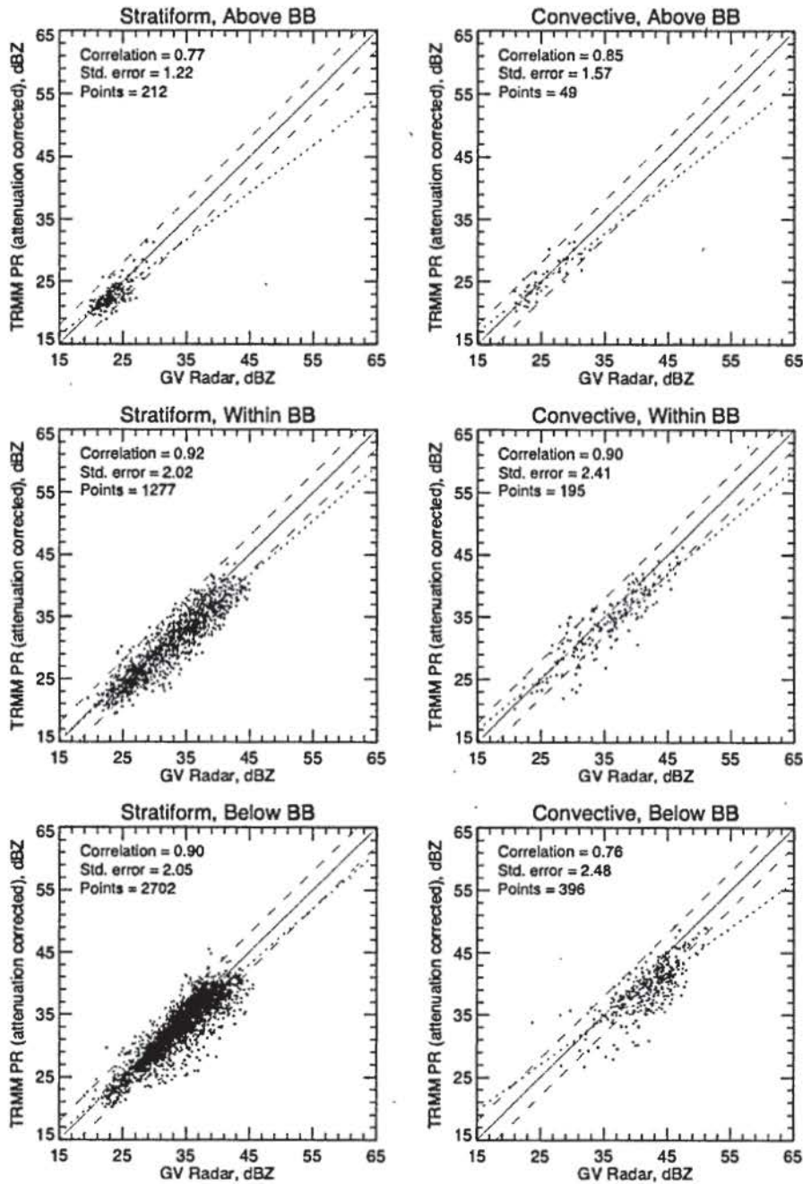
Figure 6. Scatter plots of PR vs. GR reflectivity for the same case and data constraints shown in Figures 4 and 5. Solid lines indicate the 1:1 match, dashed lines indicate \pm 3 dBZ bounds, and dotted lines are the linear fit to the data.
