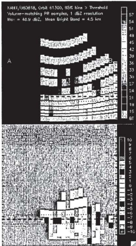
Figure 7. Vertical cross section, from 0-20 km height, of PR reflectivity (top) and PR-GR reflectivity difference (bottom) from geometrically-matched PR and GR data along the PR scan line labeled A-B in Figure 4. GR data have had S-to-Ku band adjustments applied. PR data shown in gray show sample points rejected based on the threshold criteria of Figure 4. Vertical extent of samples in the lower elevation sweeps has been adjusted to eliminate overlaps in the plots. The heavy dashed line indicates the mean bright band height, and dotted lines plotted 750 m above and below this height indicate the area of influence of the bright band (see text).
