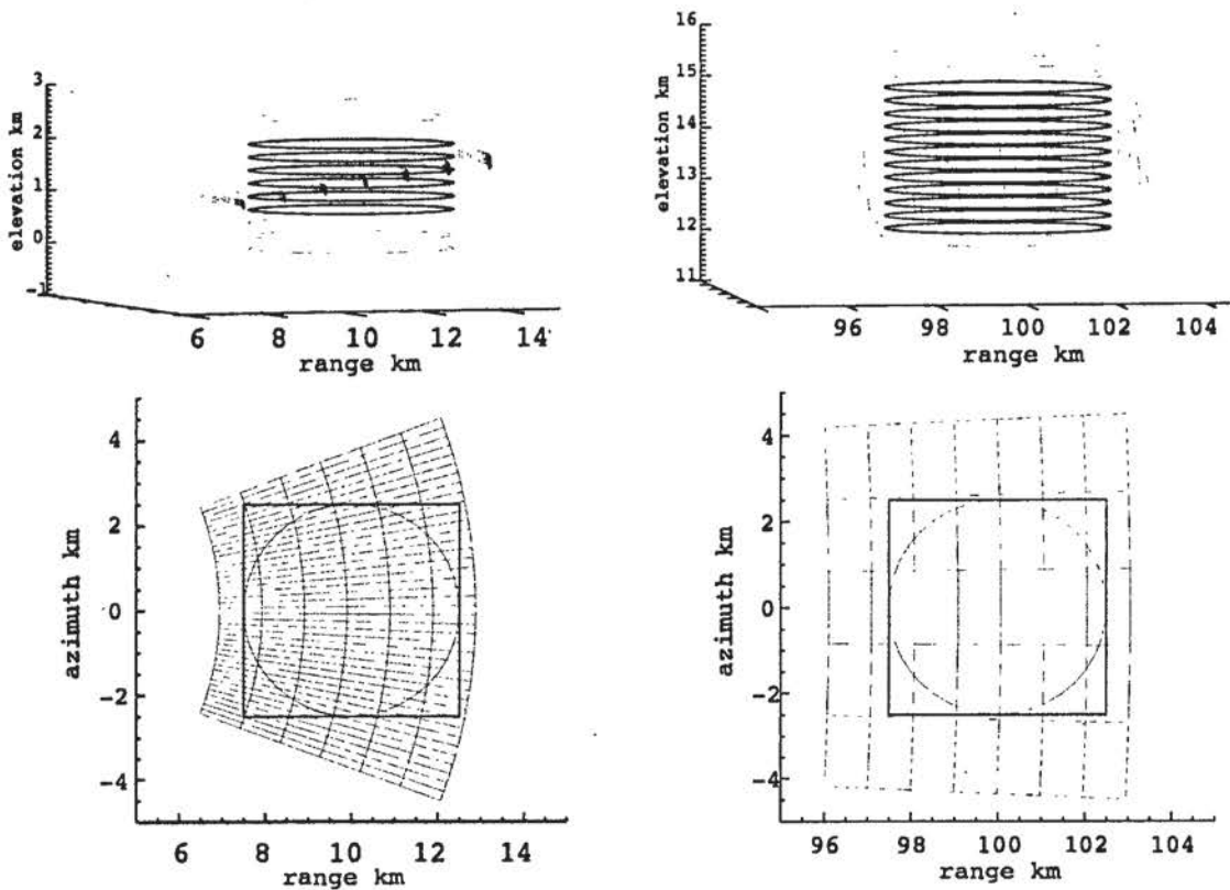
Figure 3. Illustration of the intersection of TRMM Precipitation Radar (PR) and WSR-88D Ground Radar (GR) sample volumes in the near range (left) and far range (right). The upper illustrations provide a three-dimensions representation of GR radar volumes propagating horizontally at a 7.76^\circ elevation angle as they intersect with nadir-pointing PR radar volumes propagating vertically. The projection of these intersections to the ground along a PR ray is illustrated below, again for the near and far ranges (left and right sides, respectively). The number of GR echoes included in the match-ups is much larger in the near range (left) than in the far range (right).
