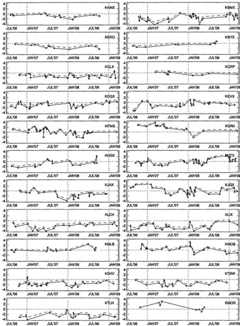
Figure 8. Time series of PR-GR mean reflectivity differences, in dBZ, for stratiform rain above the bright band. Individual rain event dates are shown by the asterisks. The solid (dashed) line shows differences based on unadjusted (S-to-Ku frequency-adjusted) GR. Only GR-unadjusted difference values are plotted for RMOR, a C-band radar.
