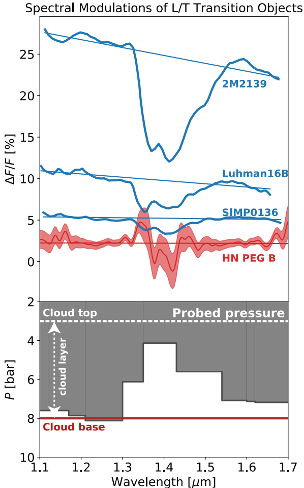
Figure 6. Comparison of HN Peg B with L/T transition brown dwarfs that have WFC3 G141 time-resolved observations. Upper: Spectral modulations defined in equation 1 are plotted. Lines are best-fit linear trends for spectral modulations out of 1.4\ \mu\text{m} water absorption band. Lower: Vertical spans of the atmosphere that are probed by different wavelength light curves are indicated in gray. (Pressure levels are calculated specifically for SIMP0136. Wavelength ranges that were not listed in Yang et al. (2016) are interpolated with adjacent bands. Red solid and dashed line show cloud base and top, respectively.)
