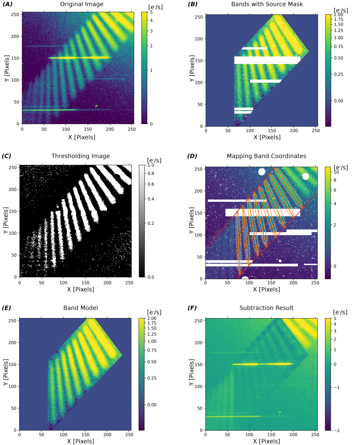
Figure 1. An example for original FIT frame, intermediate product, and the result after band subtraction. The order of the images corresponds to the sequence of reduction steps. The Images are: A) image before band subtraction; B) high S/N bands with astrophysical signal masked out; C) thresholding results, foreground pixels are plotted in white; D) coordinate regularization and re-mapping; E) empirically interpolated surface; F) image after band subtraction.
