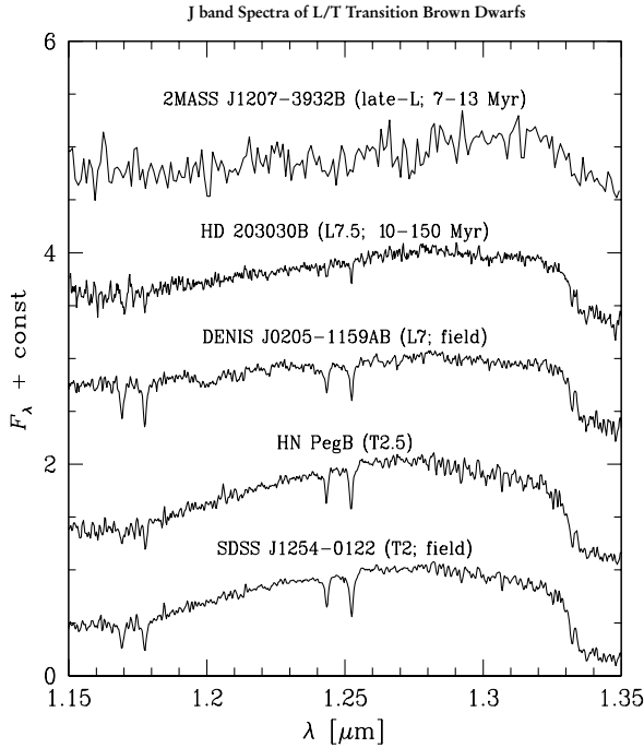
Figure 3. The Keck/NIRSPEC J -band spectrum of HN Peg B compared to the spectra of young and field-aged L/T transition dwarfs: the 10 \pm 3 Myr-old late-L TWA member 2MASS J1207–3932B (Chauvin et al. 2004), the Myr-old L7.5 dwarf HD 203030B (Metchev & Hillenbrand 2006; Miles-Páez et al. 2017), and the field-age ( >500 Myr old) L7 and T2 dwarfs DENIS J02051159AB and SDSS J12540122 (spectra from McLean et al. 2003). J band spectra for L/T transition brown dwarfs. HN Peg B resembles high surface gravity field brown dwarfs.
