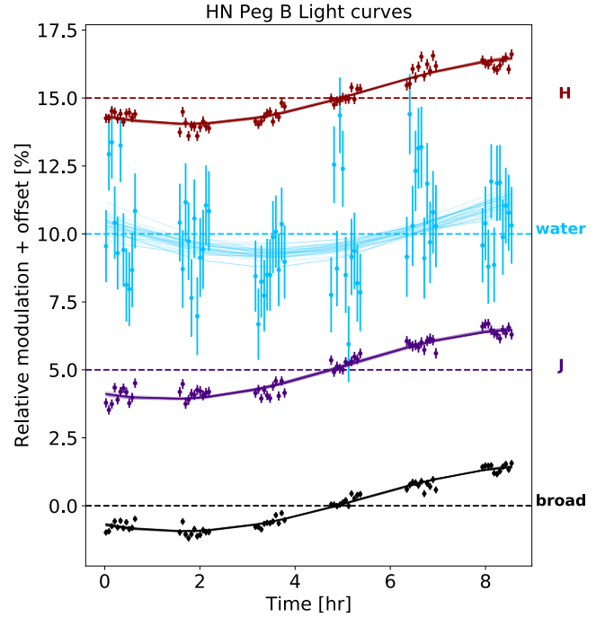
Figure 4. HN Peg b’s light curves in WFC3 G141 band pass. Observed 1.1–1.7 \mu\text{m} broad, J , water, and H bands light curves are plotted in dots with errorbars. For each bands, we also plot 30 sinusoids that are randomly selected from the posterior distributions of the sinusoidal fits (§4.1).
