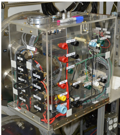
Figure 12.—A photograph of VF-6 Break-Out-Box.
