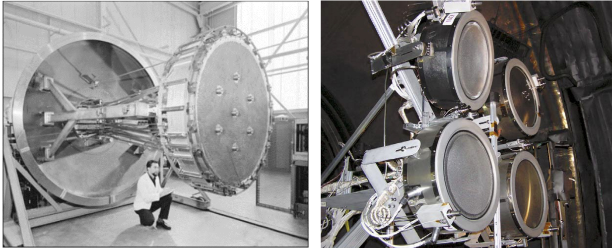
Figure 3.—The 1.5-m diameter mercury ion thruster (circa 1968) and a NEXT multi-thruster array testing (circa 2006) in VF-6.
