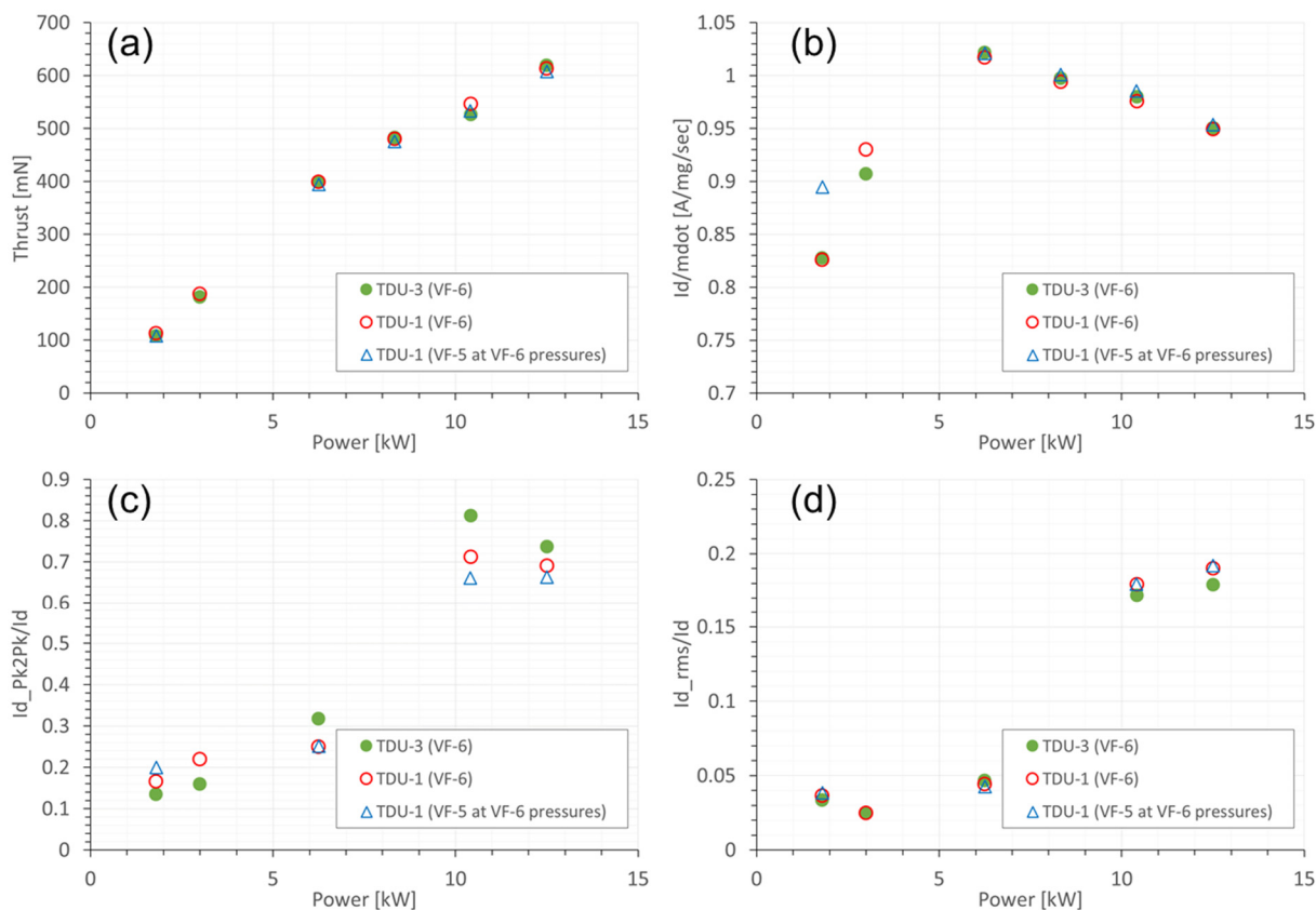
Figure 13.—Performance (a, b) and stability results (c, d) of TDU-1 and TDU-3 in VF-6 compared to TDU-1 results from VF-5 at an elevated facility pressure.
