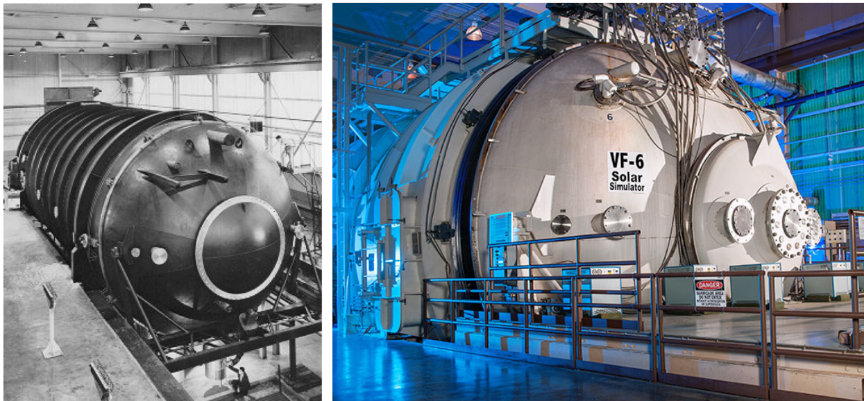
Figure 2.—NASA Vacuum Facility 6 during construction circa 1961 (left) (Ref. 6) and a recent photograph (right).
