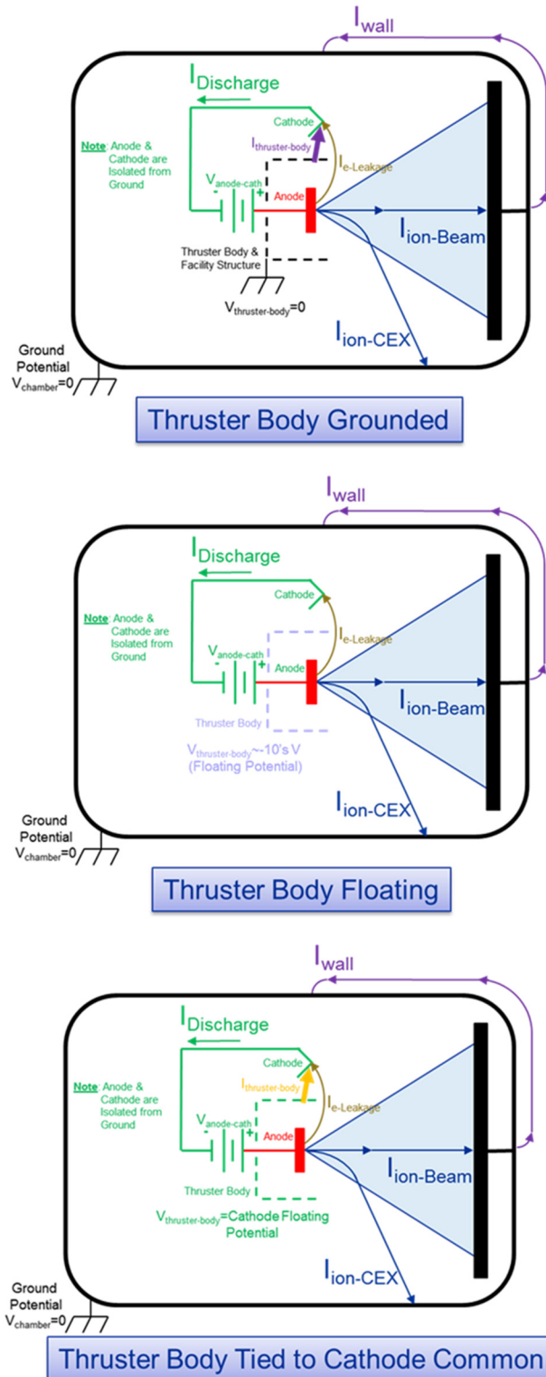
Figure 11.—Illustration of a Hall thruster body grounded, body floating, and thruster body tied to cathode common electrical configurations for ground based Hall thruster testing (Ref. 11).
