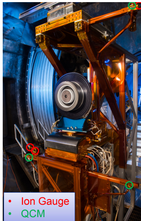
Figure 10.—QCM and ion gauge location on the VF-6 test setup.
