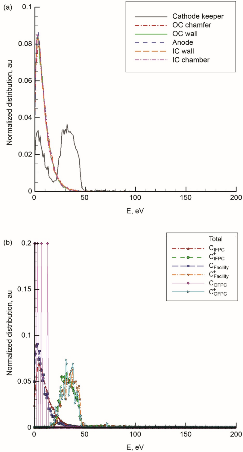
Figure 12.—(a) Energy distributions of backspattered carbon redepositing on all surfaces. (b) Energy distributions of individual carbon species redepositing on cathode keeper surface. IC, inner channel; IFPC, inner front pole cover; OC, outer channel; OFPC, outer front pole cover.
