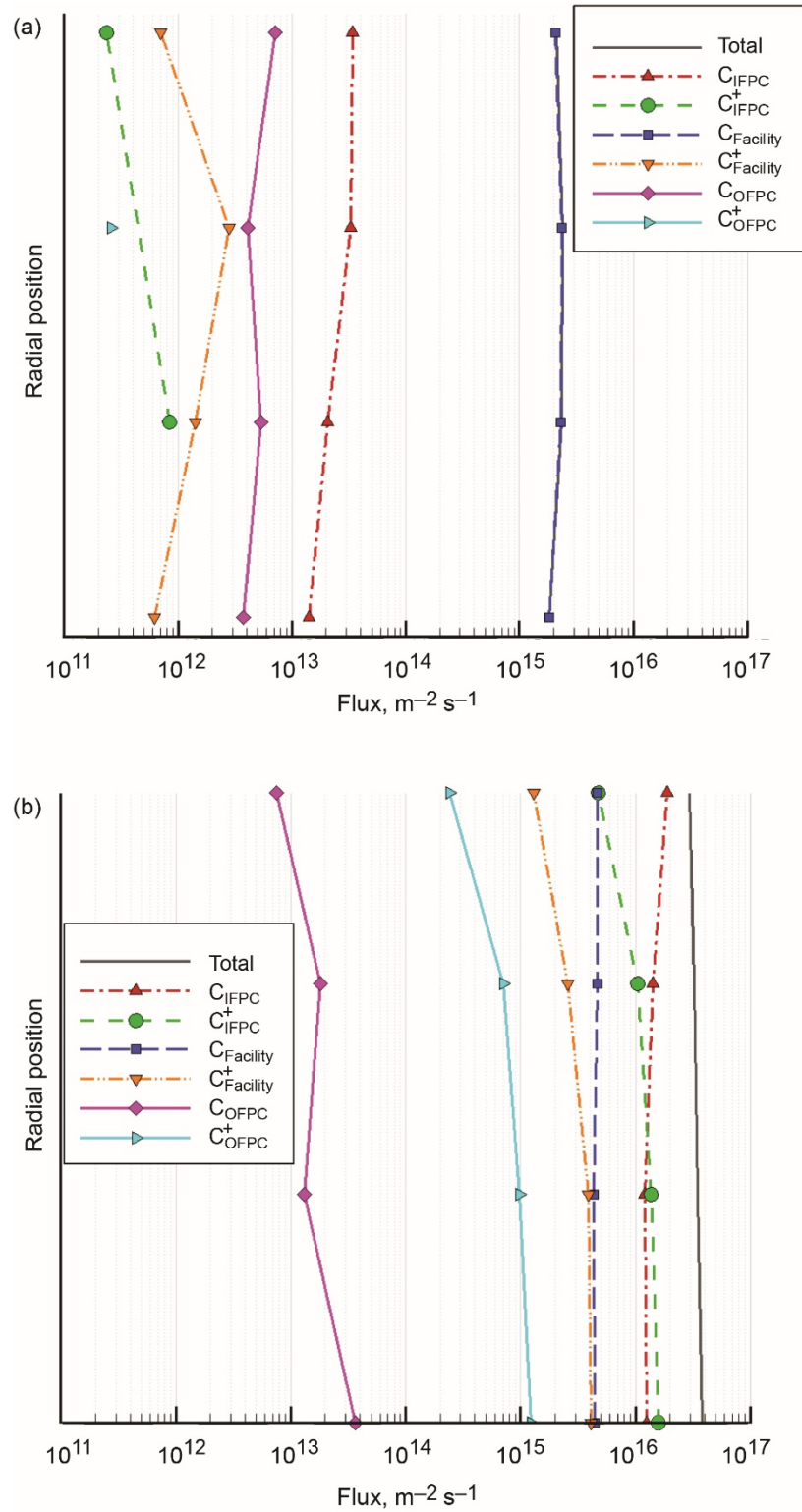
Figure 11.—Fluxes of backspattered carbon redepositing. (a) On anode surface. (b) On the cathode surface. IFPC, inner front pole cover; OFPC, outer front pole cover.
