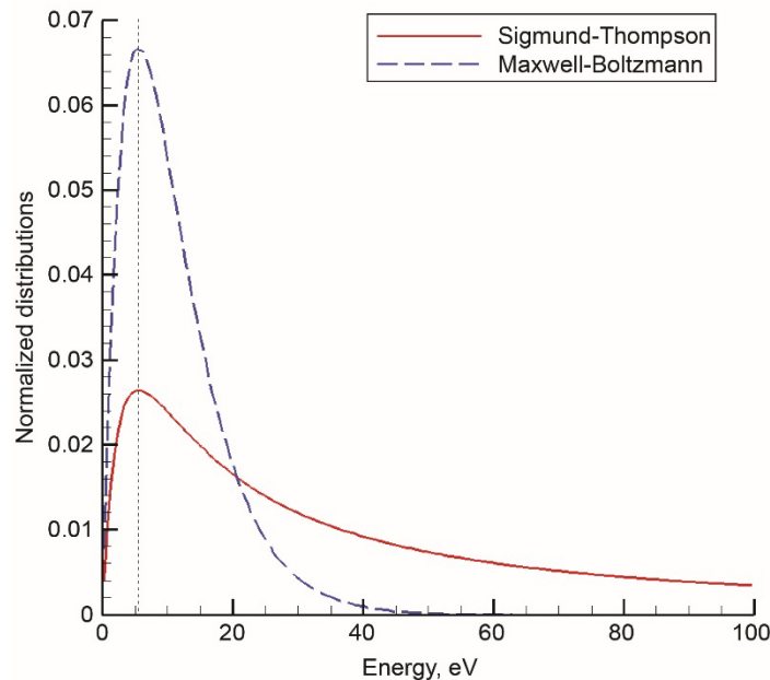
Figure 5.—Comparison of Sigmund-Thompson distribution (red) and sampled energy distribution for backscattered carbon, assuming Maxwellian velocity distribution function (VDF) (blue). By matching most probable energy of 5.6 eV, carbon with higher and lower energies is underestimated and overestimated, respectively.
