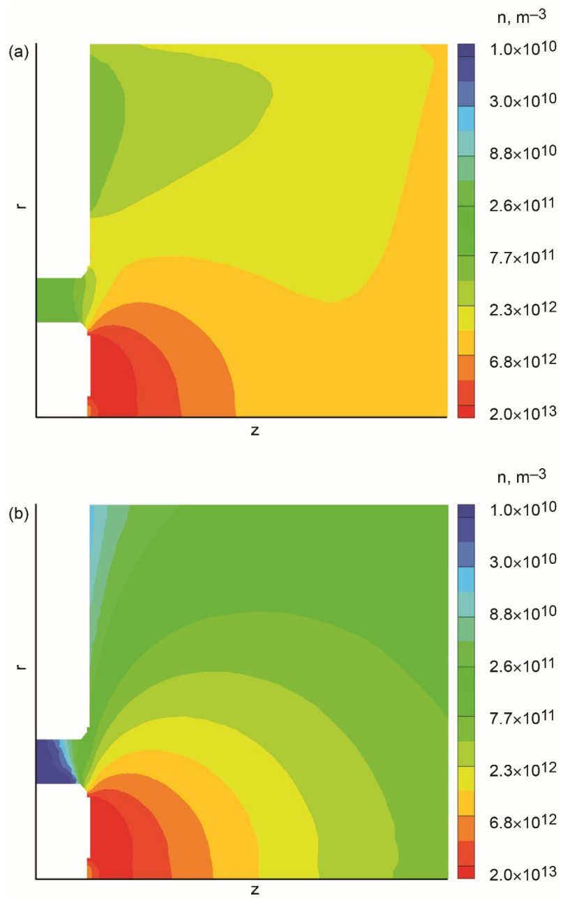
Figure 8.—Number densities. (a) Total carbon atoms. (b) Inner front pole cover (IFPC) carbon atoms. (c) Outer front pole cover (OFPC) carbon atoms. (d) Facility backscatter carbon atoms.
