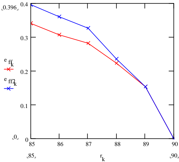
Fig. 51 Measured efficiency TM wave
