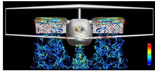
Fig. 7. Elytron 4S UAV, a box-wing configuration, during VTOL out of ground effect, viewed from the front. Q-criterion vorticity iso-surfaces colored by the vorticity magnitude.
