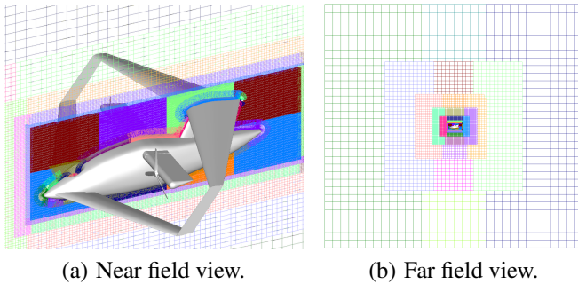
Fig. 6. Elytron 4S UAV OB Cartesian grids for case IV. The surface geometry in grey-shaded, and a cut of all volume grids with plane y = 0 are shown.
