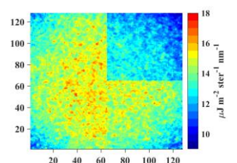
Fig. 1(d) Mean event energy detected in the LIS pixel array
