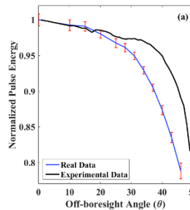
Fig. 3(a) Mean event energy density fall-off with off-boresight angle
