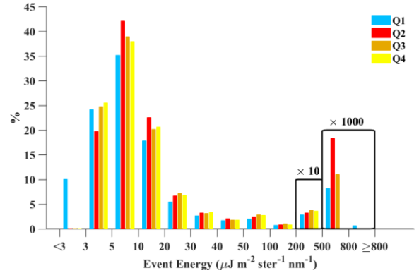
Fig. 2 Histogram of LIS event energy density
