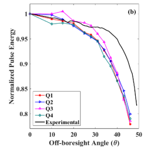
Fig. 3(b) Quadrant mean event energy density fall-off with off-boresight angle
