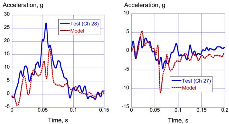
(a) Vertical acceleration responses.
