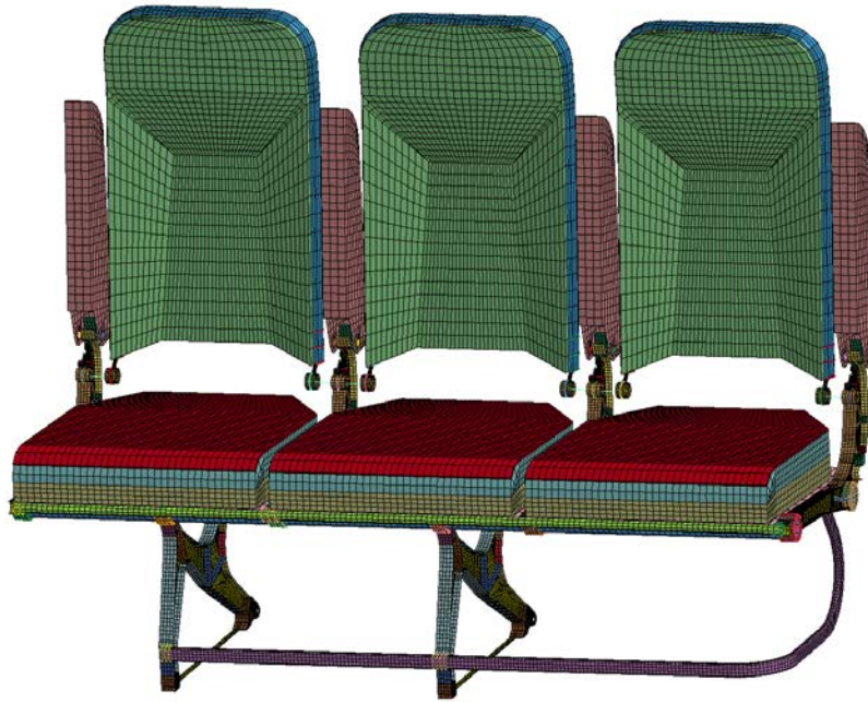
Figure 20. Seat finite element model.
