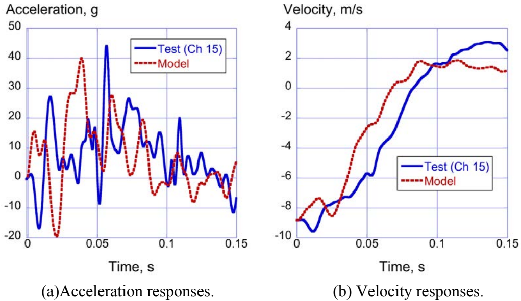
Figure 32. Vertical acceleration and velocity comparisons at the port aisle at FS 6805.
