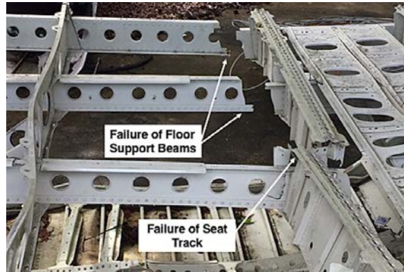
(b) Floor failures.
