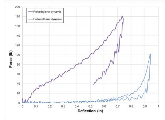
(b) Force/deflection response.
