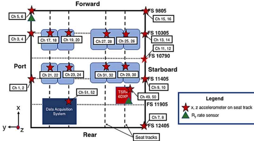
Figure 8. Floor-level instrumentation of the wing-box fuselage section.
