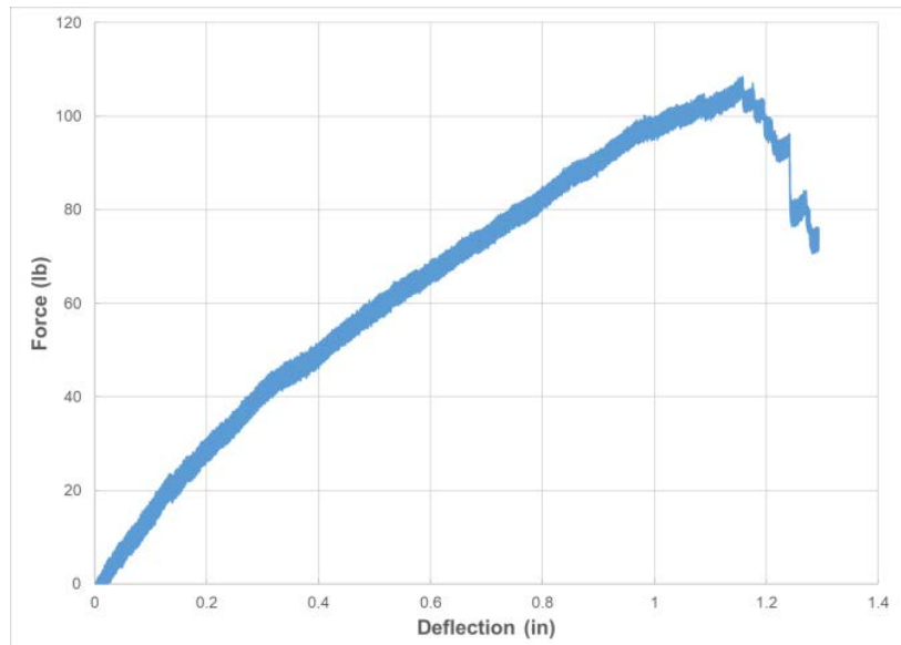
(b) Tensile test data of the seat pan fabric.
