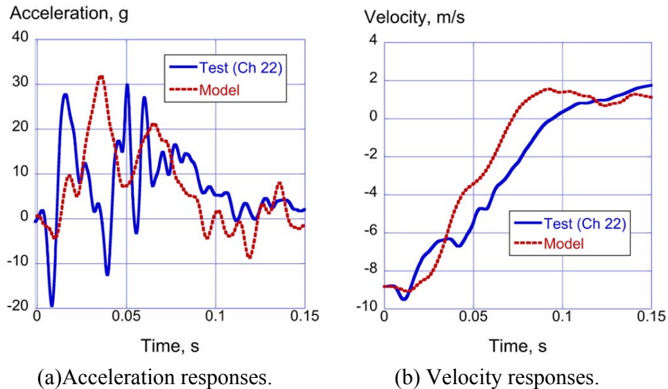
Figure 33. Vertical acceleration and velocity comparisons at the starboard aisle at FS 6805.
