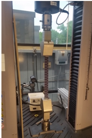
(a) Tensile test of a seat cushion cover.
