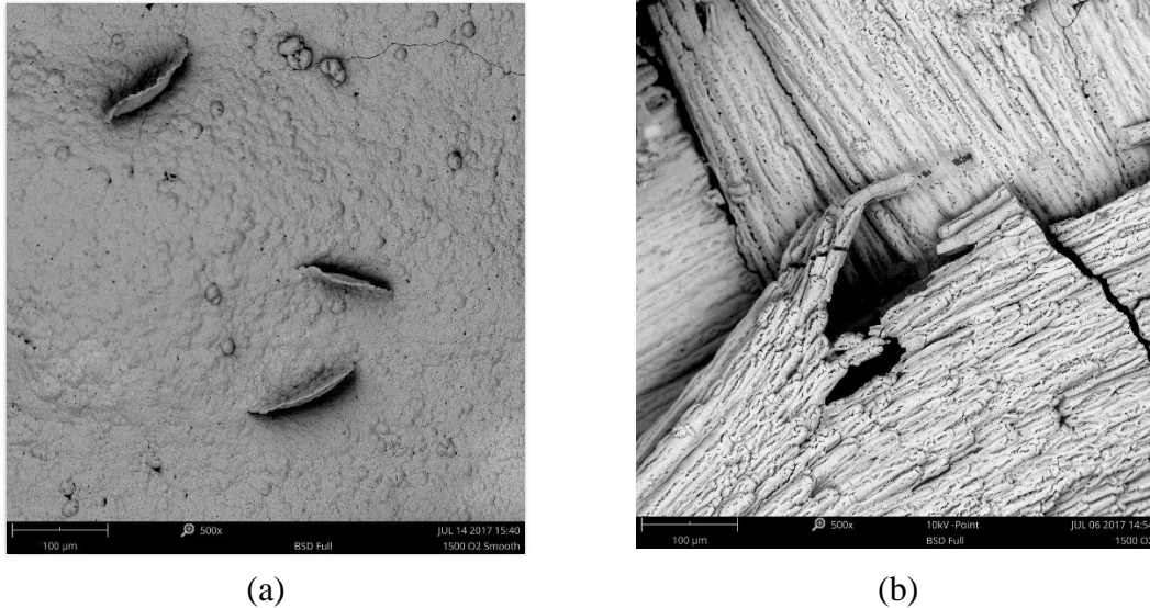
(a) (b) Figure 5. Scanning Electron Microscope (SEM) images of a 1500°C oxidation tested specimen. Image (a) shows the ‘smooth’ side of the sample tested at 1500°C for 100 hours, while image (b) shows the ‘rough’ side of the same sample. One can note the difference in grain texture, as well as the beginnings of spallation on the ‘smooth’ side.
