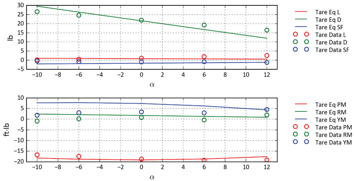
Figure D-4: Airplane Mode—R508 \alpha = 0 , Q = 80 .
