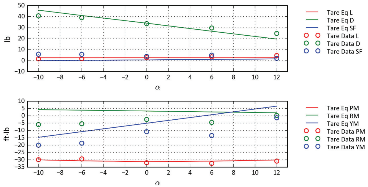
Figure D-12: Airplane Mode—R517 \alpha = 5 , Q = 120 .
