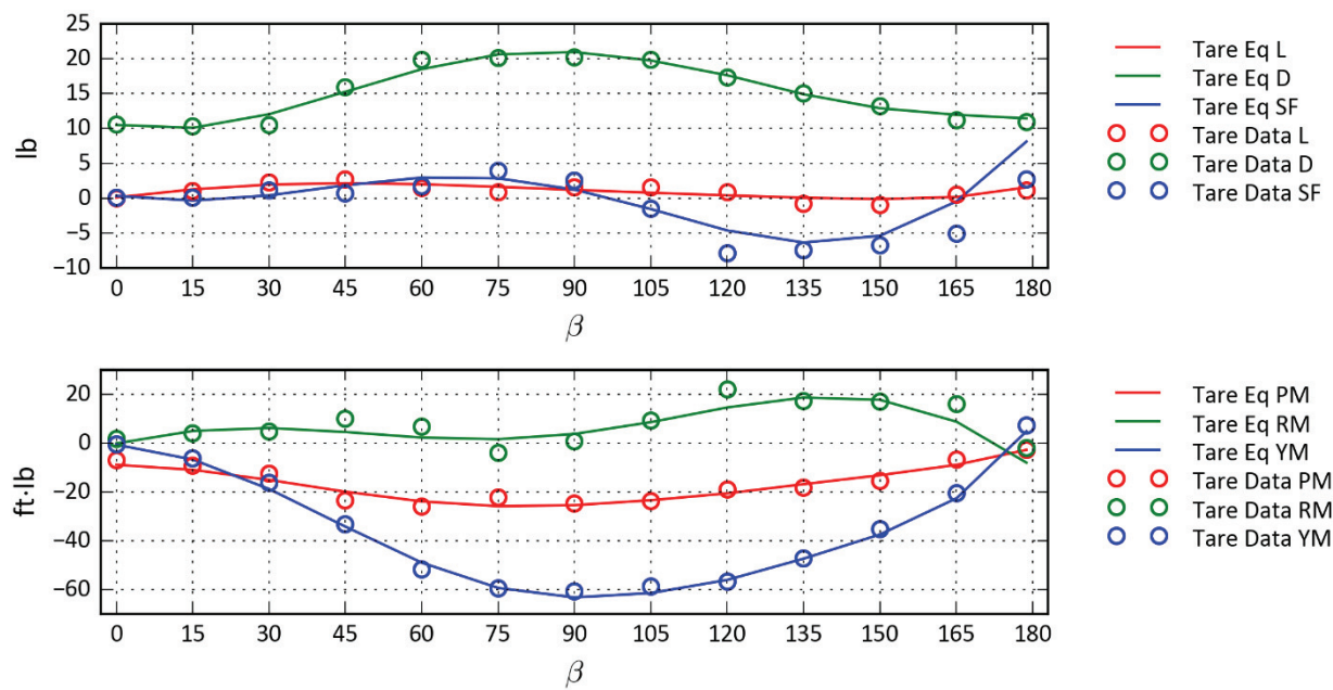
Figure D-31: Helicopter Mode—R544B \alpha = 5 , Re = 0.6 .
