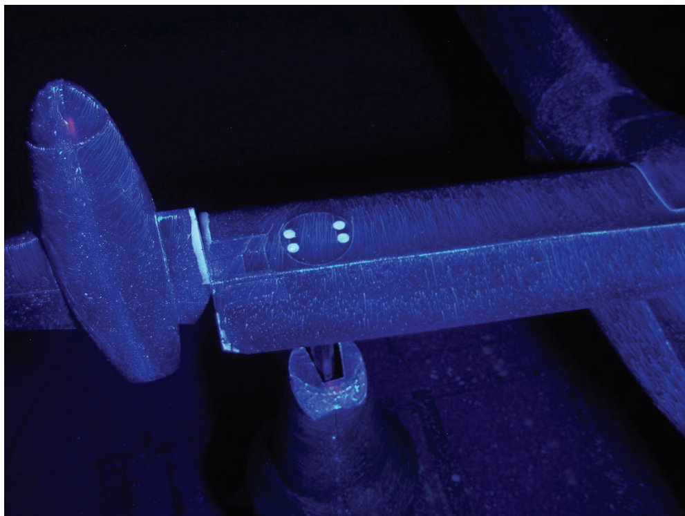
Figure B-85: LS8 flow visualization over nacelle (port-aft).
