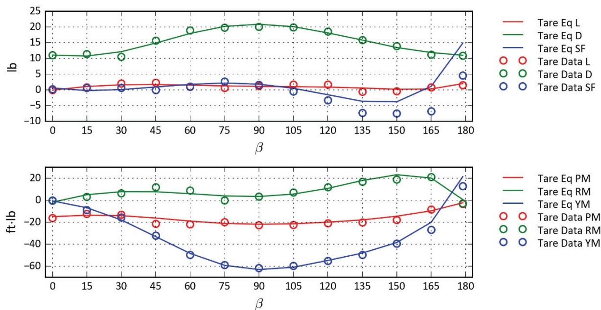
Figure D-30: Helicopter Mode—R540B \alpha = -5 , Re = 0.6 .
