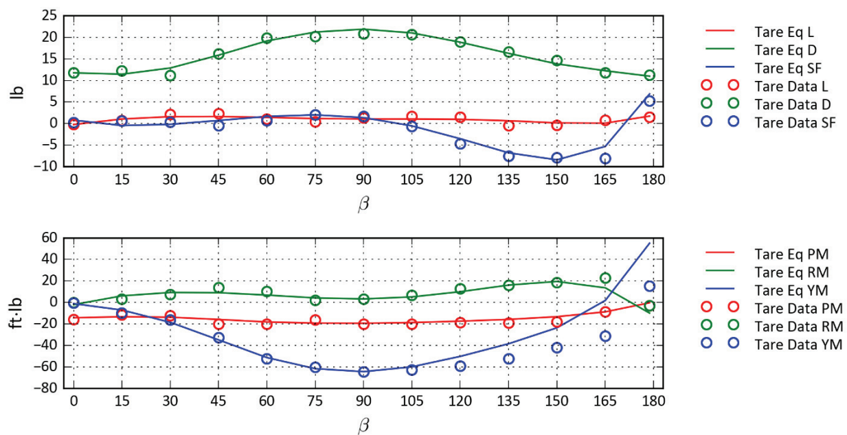
Figure D-28: Helicopter Mode—R540C \alpha = -10 , Re = 0.6 .
