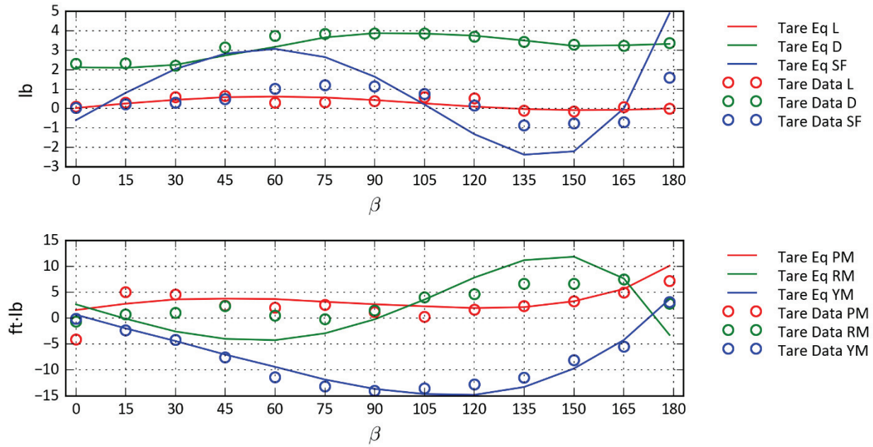
Figure D-25: Helicopter Mode—R535 \alpha = 0 , Re = 0.3 .
