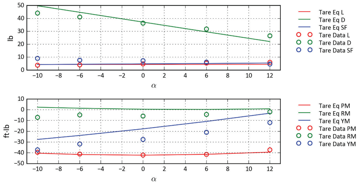
Figure D-18: Airplane Mode—R520 \alpha = 10 , Q = 130 .
