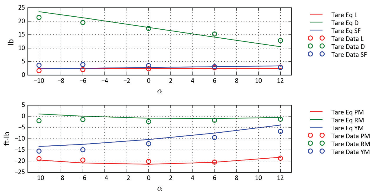
Figure D-14: Airplane Mode—R520 \alpha = 10 , Q = 60 .
