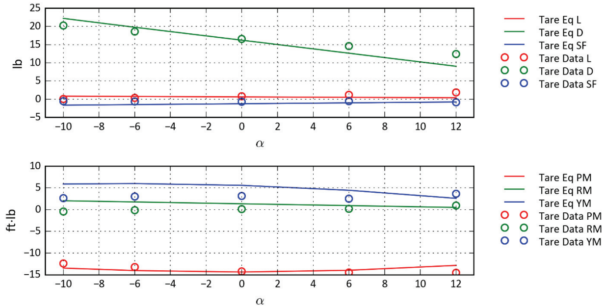
Figure D-3: Airplane Mode—R508 \alpha = 0 , Q = 60 .
