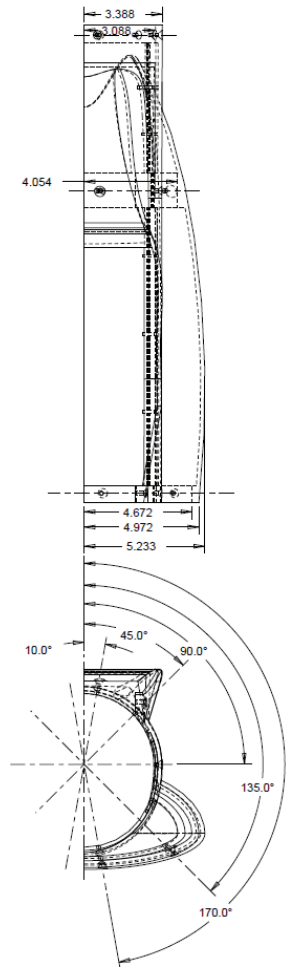
Figure A-5: Technical drawing of the LCTR2 model fuselage (mid-port).
