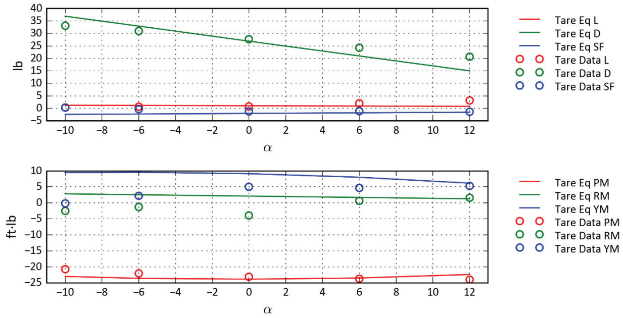
Figure D-5: Airplane Mode—R508 \alpha = 0 , Q = 100 .
