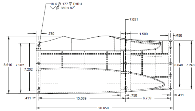
Figure A-5: Technical drawing of the LCTR2 model fuselage (mid-port).
