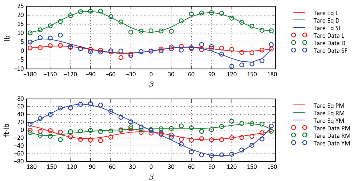
Figure D-27: Helicopter Mode—R544A \alpha = 0 , Re = 0.6 .
