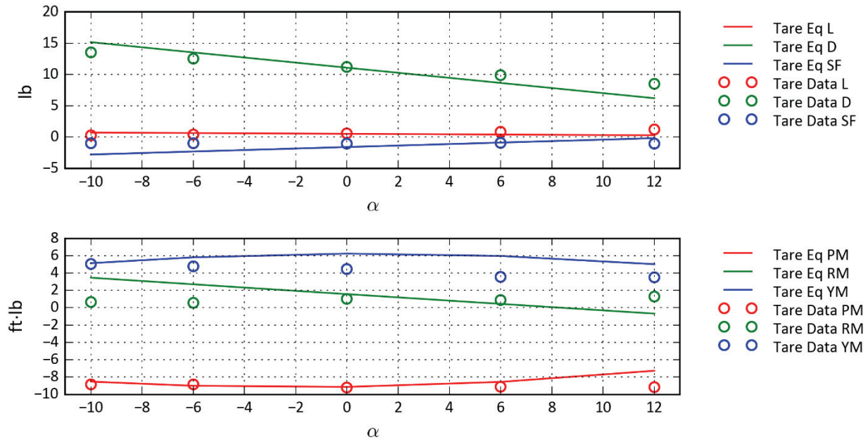
Figure D-19: Airplane Mode—R529 \alpha = -5 , Q = 40 .
