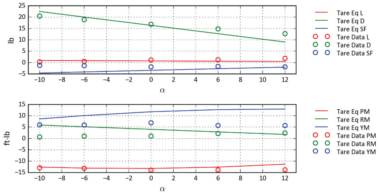
Figure D-20: Airplane Mode—R529 \alpha = -5 , Q = 60 .
