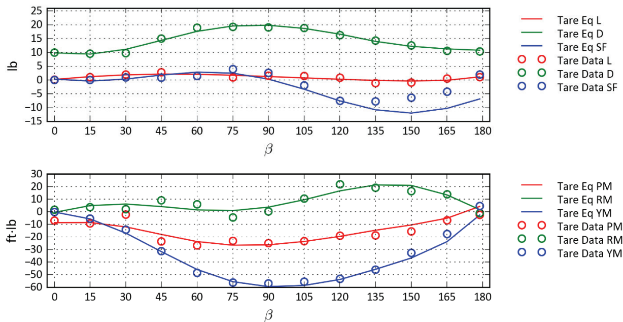
Figure D-29: Helicopter Mode—R544C \alpha = 10 , Re = 0.6 .
