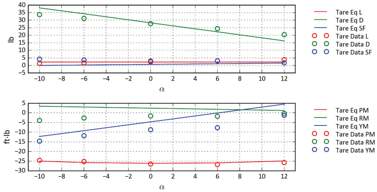
Figure D-11: Airplane Mode—R517 \alpha = 5 , Q = 100 .
