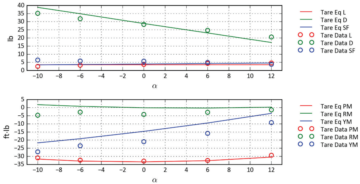
Figure D-16: Airplane Mode—R520 \alpha = 10 , Q = 100 .
