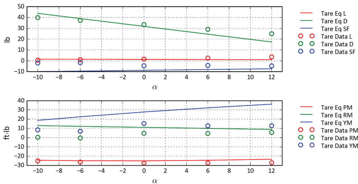
Figure D-23: Airplane Mode—R529 \alpha = -5 , Q = 120 .
