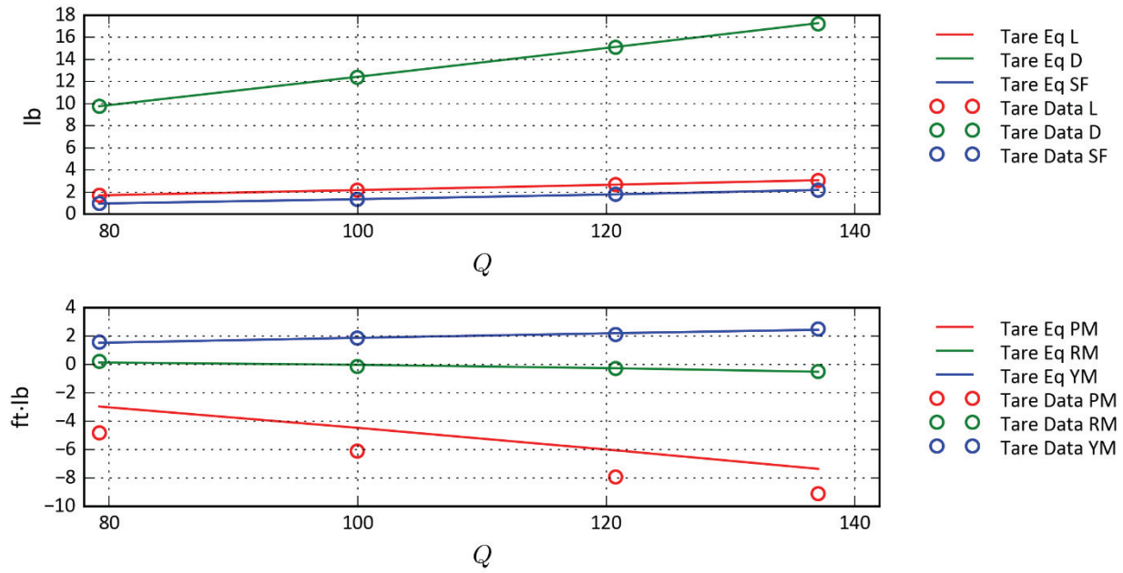
Figure D-33: Wing Only—R504 \alpha = 0 , \beta = 5 .
