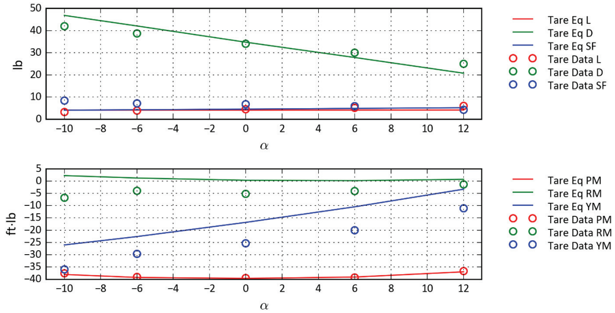
Figure D-17: Airplane Mode—R520 \alpha = 10 , Q = 120 .
