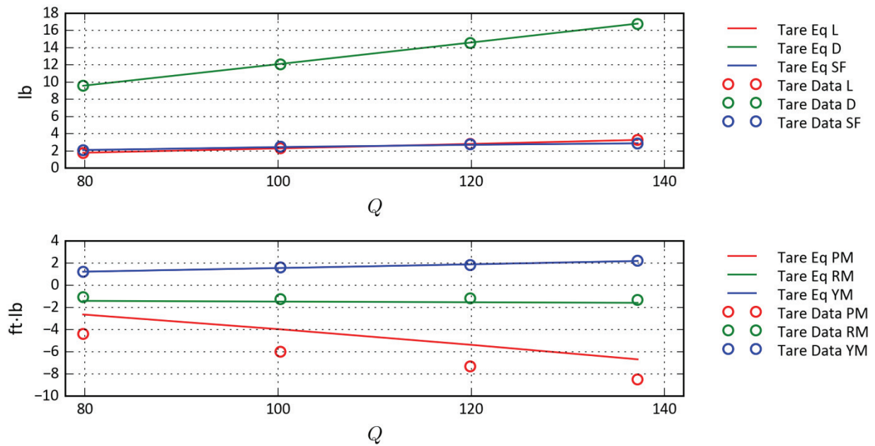
Figure D-34: Wing Only—R506 \alpha = 0 , \beta = 10 .
