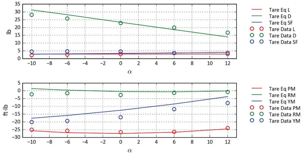
Figure D-15: Airplane Mode—R520 \alpha = 10 , Q = 80 .
