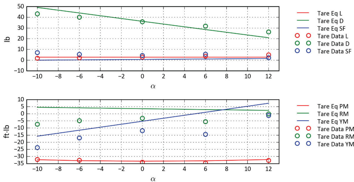
Figure D-13: Airplane Mode—R517 \alpha = 5 , Q = 130 .
