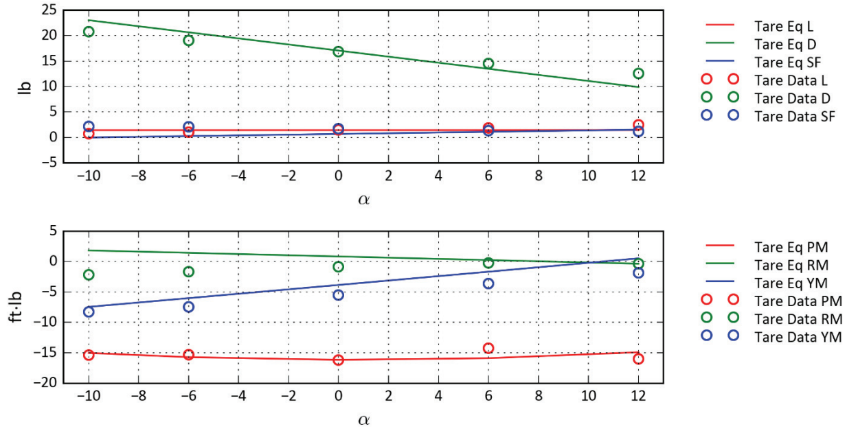
Figure D-9: Airplane Mode—R517 \alpha = 5 , Q = 60 .
