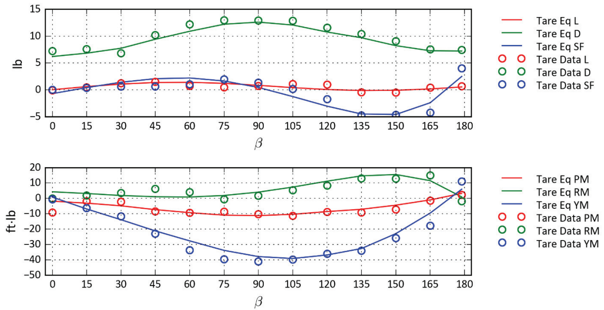
Figure D-26: Helicopter Mode—R535 \alpha = 0 , Re = 0.45 .
