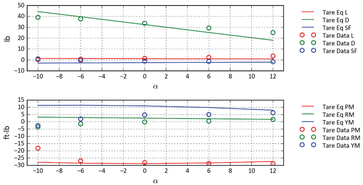
Figure D-6: Airplane Mode—R508 \alpha = 0 , Q = 120 .
