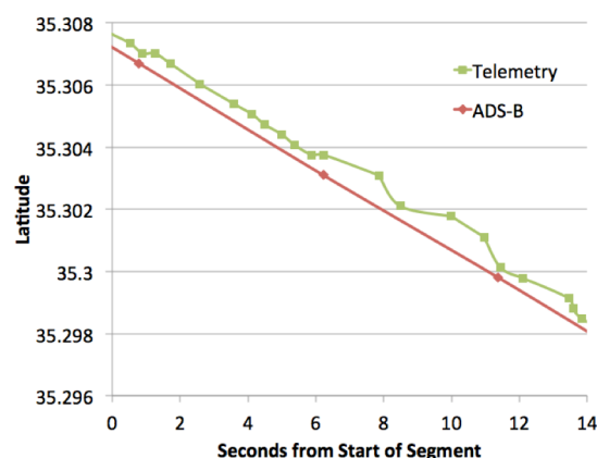
Figure 9. T-34C Track Latency. The T-34C telemetry has a 0.5-1.0 second time shift and increased variability differences compared to ADS-B.
