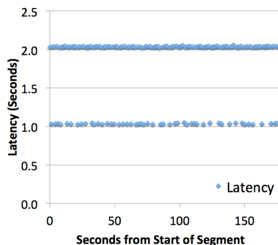
Figure 6. Aircraft to NextGen System Latency. The difference between the time the position report was received by NextGen and the position TOA.
