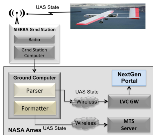
Figure 11. Connection of SIERRA. The system diagram showing the connection between the NASA SIERRA UAS and the NASA LVC infrastructure.
