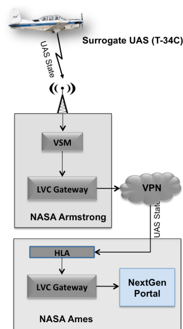
Figure 7. Connection of T-34C. The system diagram showing the connection between the NASA T-34C surrogate aircraft and the NASA LVC infrastructure.
