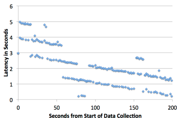
Figure 12. SIERRA to NextGen System Latency. The difference between the time the position report was received and the position TOA.
