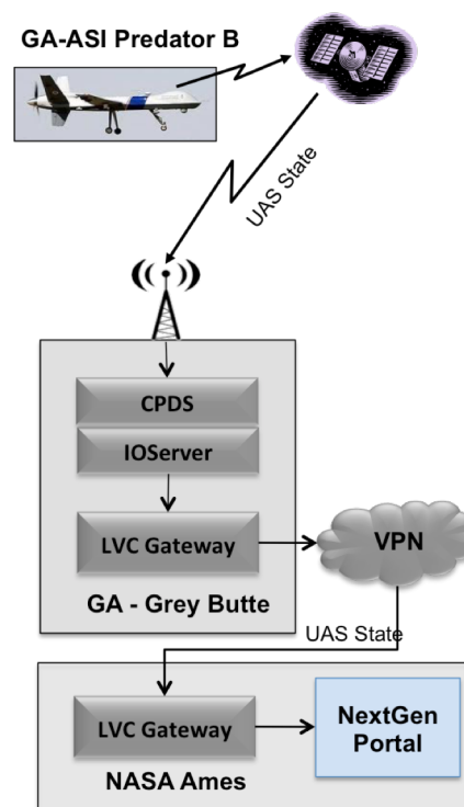
Figure 3. Connection to Predator B Class UAS. The system diagram showing the connection between the General Atomics' Predator B capital asset and the NASA LVC infrastructure.
