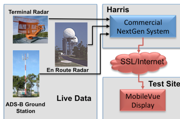
Figure 13. GCS Display Connection. High level system architecture showing the connection between the NextGen system and the Harris MobileVue application.
