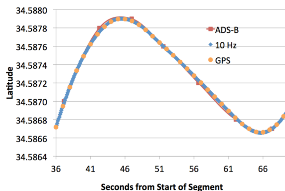
Figure 5. Predator B Position Data Smoothness. The self-reported positions of the Predator B data shows good conformance with the ADS-B and GPS data.
