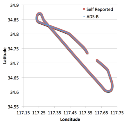
Figure 4. Predator B Track History. Aircraft self-reported positions overlaid with the recorded ADS-B position of the aircraft.
