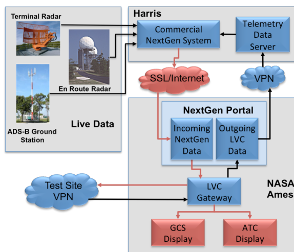
Figure 1. NextGen Portal Connection. High level system architecture showing the main system components and the data flow between the Harris NextGen data and the NASA LVC.
