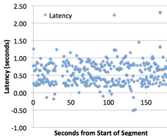
Figure 10. T-34C to NextGen System Latency. The difference between the time the position report was received and the position TOA.
