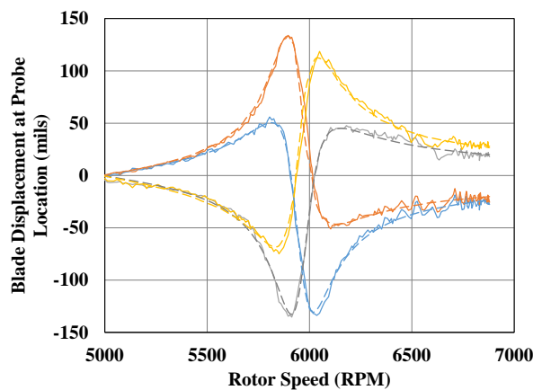
b. Wind tunnel (four probes, one blade)
