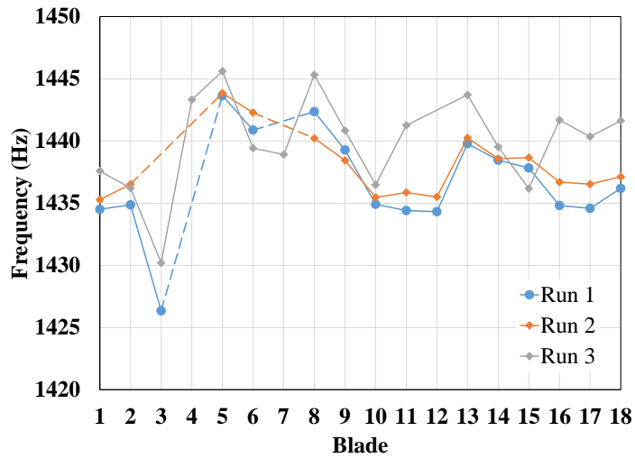
Fig. 22 Blade resonance frequency for three sweeps of 8EO/M4 in the wind tunnel
