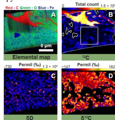
Figure 1. (A) STXM elemental map of Carancas 1. (B) NanoSIMS 12 C elemental map, and isotopic images of (C) \delta D and (D) \delta^{13} C.
