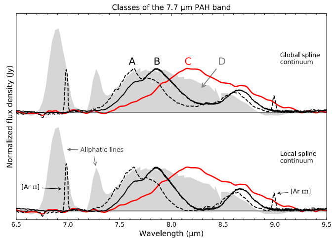
Figure 1. The four classes of the 7.7 \mu\text{m} PAH emission complex, which are linked to object type. The physical/chemical changes in PAH populations needed to explain these variations are currently largely unknown.
