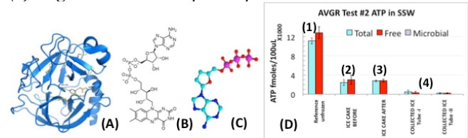
Figure 3: (A) Trypsin, (B) Flavin Adenine Dinucleotide (FAD) & (C) Adenosin Triphosphate (ATP), (D) Table of: Total, Free & Microbial ATP concentrations in synthetic sea water (1), Ice before (2) and after (3) shoot & at collection (4).
