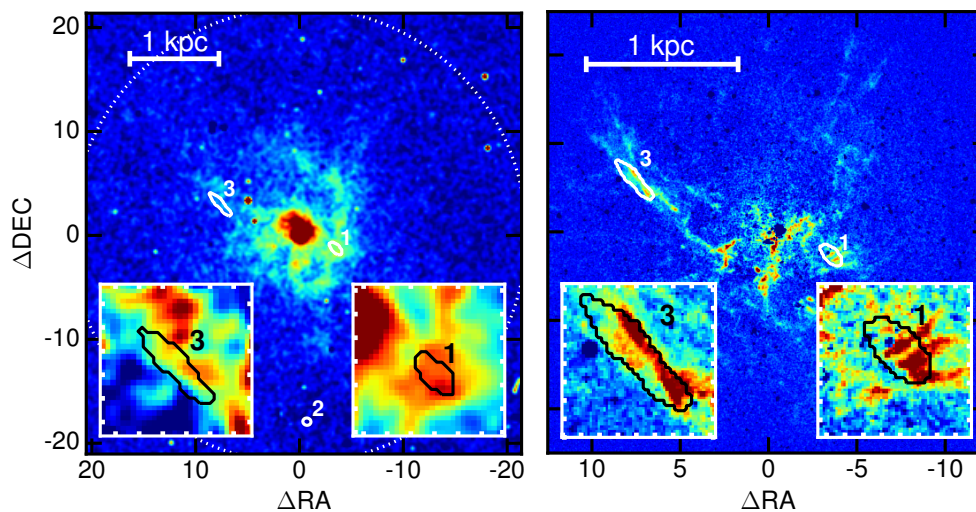
Images of NGC 5846 showing detected CO(2-1) clouds projected against an optical H\alpha+N[II] emission (left) and a dust starlight extinction image (right). Color sequence (blue \rightarrow green \rightarrow yellow \rightarrow red) indicates increasing H\alpha+[NII] and dust. CO clouds, indicated with black (in the insert) and white contours, are defined as the area where the emission line signal-to-noise is greater than 4. Clouds #1 and #3 are somewhat resolved and extend about 1.2'' and 2.9'' . Note that cloud #3 (see enlarged insert) is aligned almost exactly along a dust filament, and coincides with knots and filamentary structures in the H\alpha+[NII] emission. Cloud #1 also coincides with H\alpha+[NII] emission and dust extinction, but other similar dusty regions were not detected in CO(2-1). Cloud #2 is not associated with detectable optical emission and out of dust extinction map FOV. The white dashed circle in the H\alpha+N[II] emission map identifies the field of view of the ALMA primary beam.
