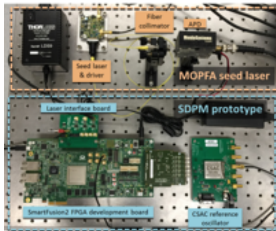
Prototype Miniature Optical Communications Transceiver Software-defined Pulsed Modulator and Seed
