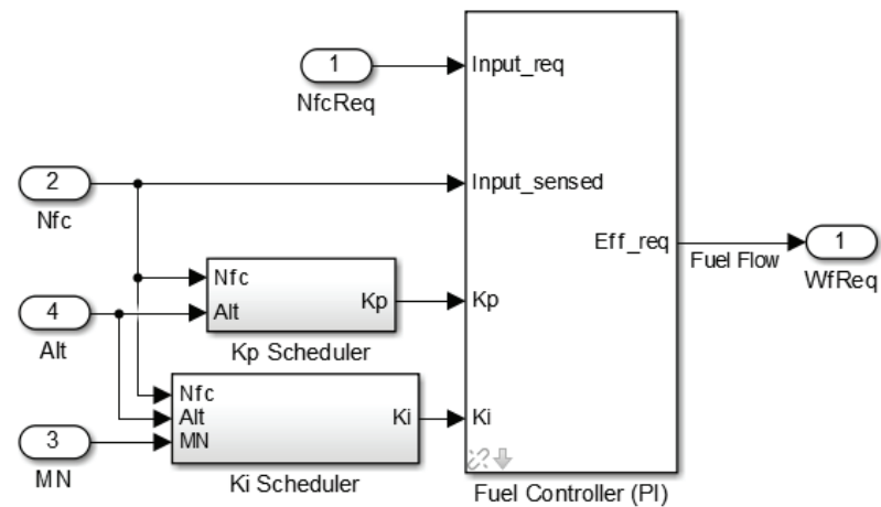
Speed Controller
