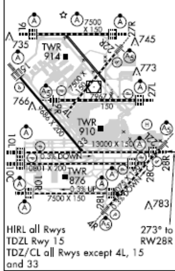
Figure 128. RNAV (GPS) RWY 28R approach plate (KORD).
