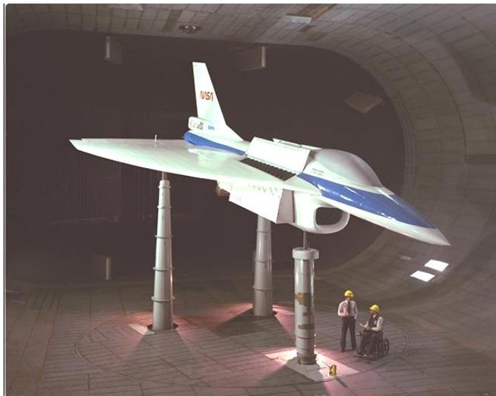
The E-7 Ejector Concept in the Tunnel
