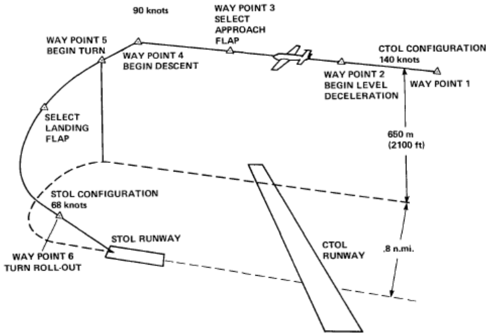
The Curved-Decelerating Descending Approach
