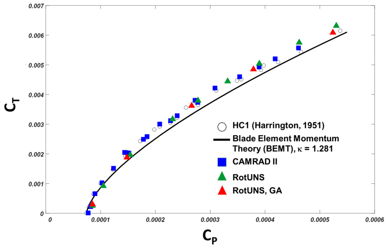
Figure 43. Performance of HC1[13] in hover compared with momentum theory, BEMT and RotUNS rotor disk model calculations.
