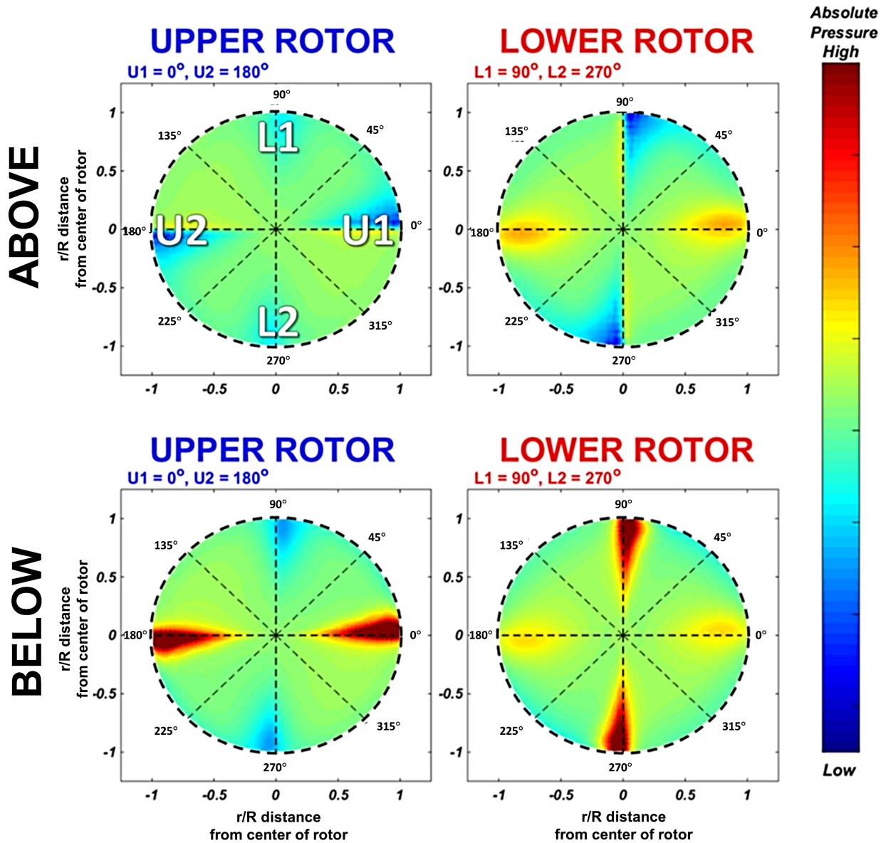
Figure 47. HC1 comparison of upper and lower rotor of absolute pressure below and above rotor, respectively, at non-overlap. RotUNS lifting-line (discrete-blade) rotor model calculations are presented for hover.
