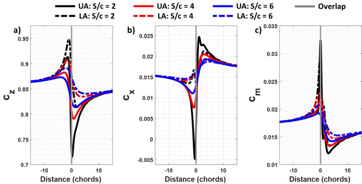
Figure 19. Two NACA 0012 airfoils crossing for a) c_z , b) c_x , and c) c_m versus distance to overlap ( M = 0.5 ( V_{tip} = 560 ft/s), \alpha = 7^\circ , and S/c = 2.0, 4.0 , and 6.0 ( c = 0.5 ft)).
