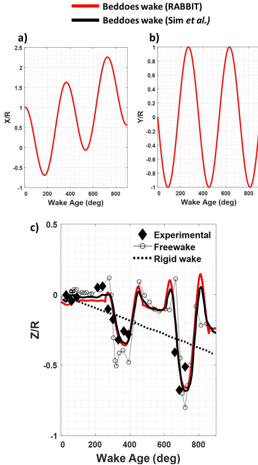
Figure 57. Rotor tip vortex wake displacement for a) X/R , b) Y/R , and c) Z/R .
