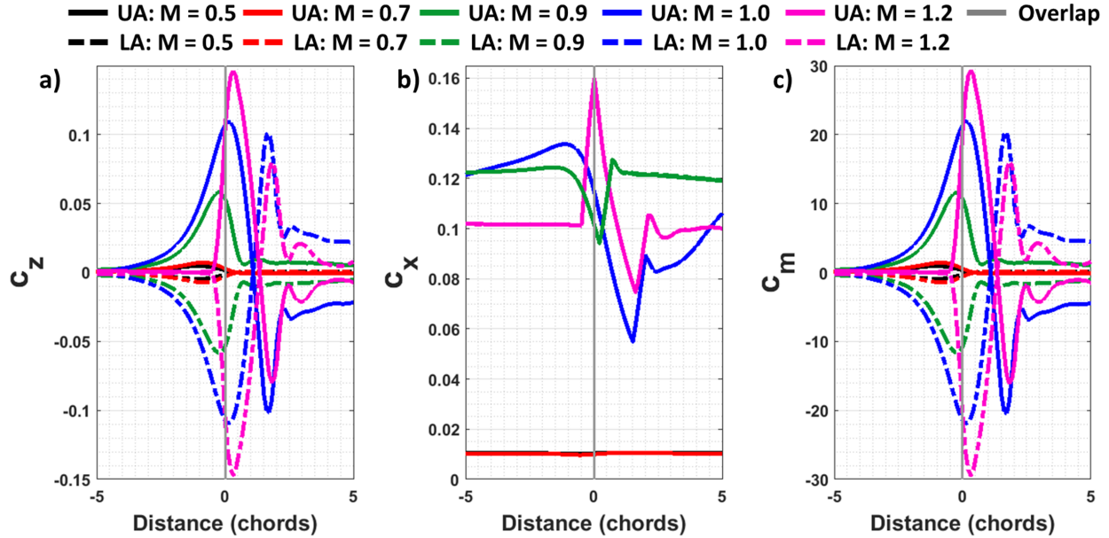
Figure 21. Two NACA 0012 airfoils crossing for a) c_z , b) c_x , and c) c_m versus distance to overlap ( M = 0.5, 0.7, 0.9, 1.0 , and 1.2 ( V_{tip} = 560, 780, 1005, 1116 , and 1340 ft/s), \alpha = 0^\circ , and S/c = 4.0 ( S = 2.0 ft, c = 0.5 ft)).
