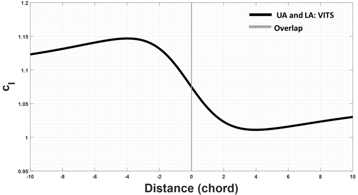
Figure 4. VITS simulation of two airfoils crossing, c_l versus distance to overlap in chords ( M = 0.25 , \alpha = 9.8^\circ , and S/c = 4.0 ( S = 2.0 ft, c = 0.5 ft)).
