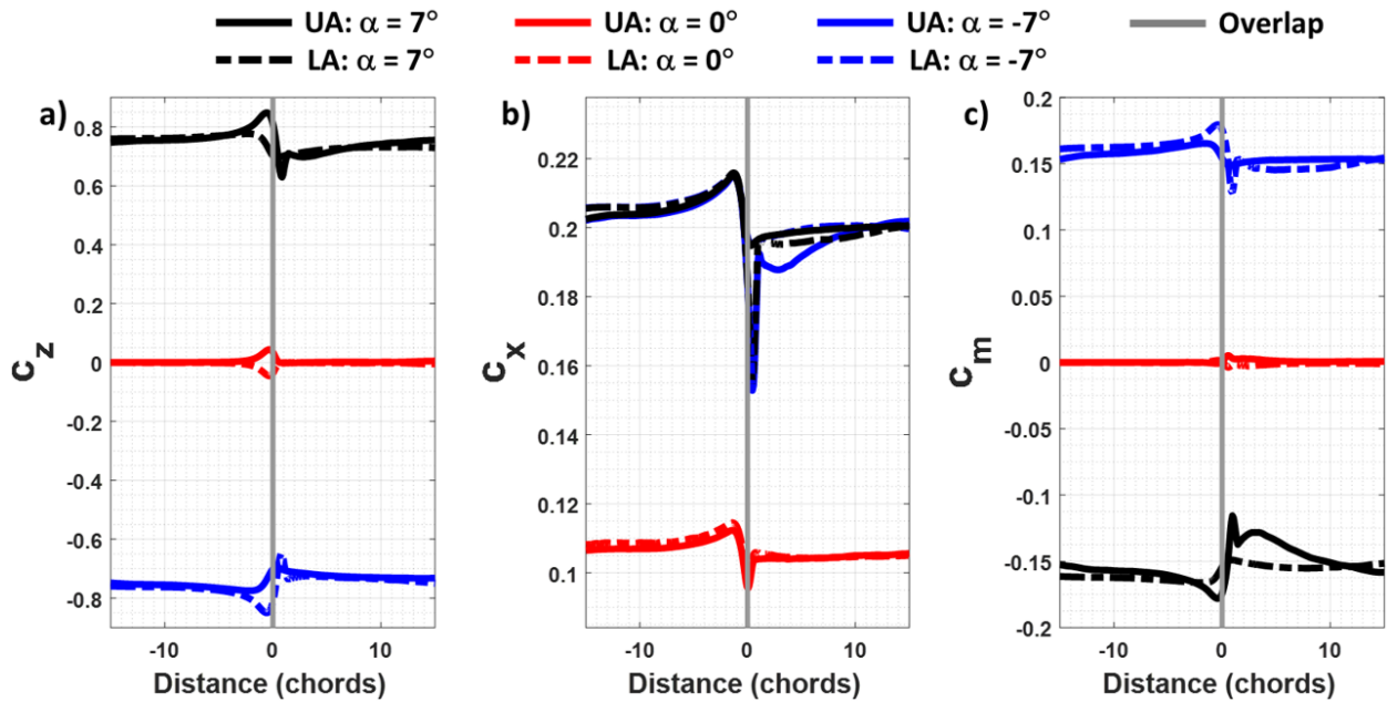
Figure 14. Two NACA 0012 airfoils crossing for a) c_z , b) c_x , and c) c_m versus distance to overlap ( M = 0.9 ( V_{tip} = 1,005 ft/s), \alpha = -7^\circ, 0^\circ , and 7^\circ , and S/c = 4.0 ( S = 2.0 ft, c = 0.5 ft)).
