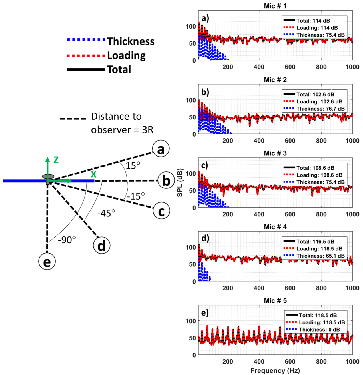
Figure 70. Elevation acoustic directivity in hover for single modern rotor frequency spectrum.
