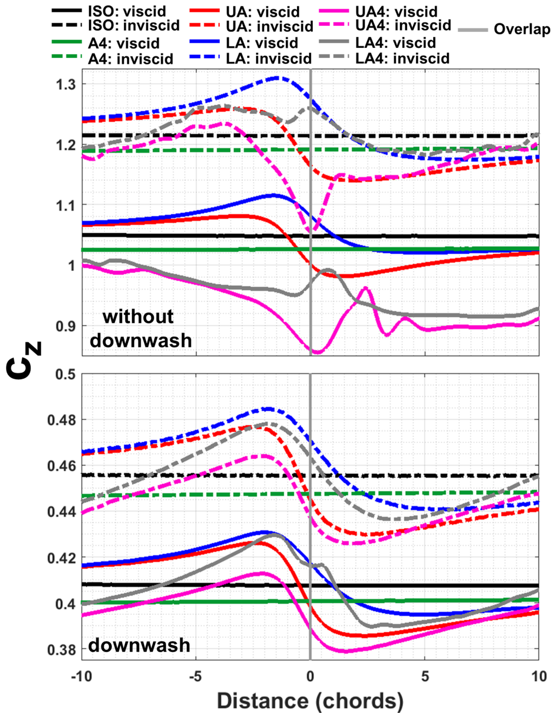
Figure 27. Viscid and inviscid isolated airfoil, two airfoils crossing at crossing ( UA/LA ), single train of eight airfoils ( A4 ), and two trains of eight airfoils at crossing ( UA4/LA4 ) with and without downwash c_z versus distance ( M = 0.25 , \alpha = 9.8^\circ , V_i = 31 ft/s, S/c = 4.0 ( S = 2.0 ft, c = 0.5 ft), and D/c = 33.51 ).
