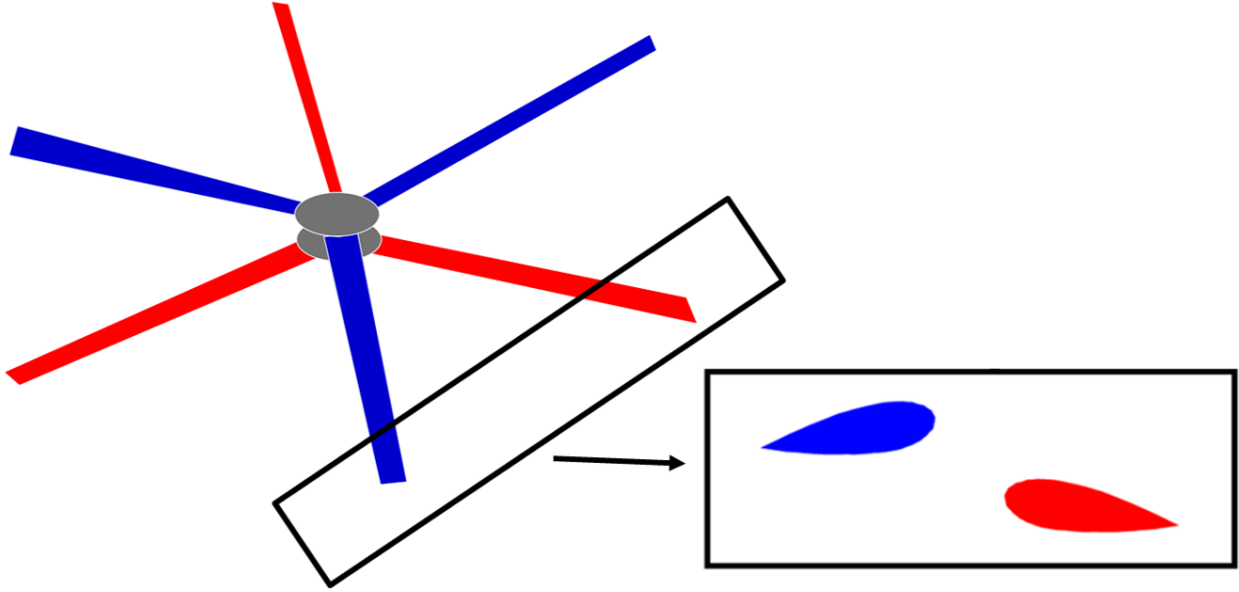
Figure 2. 3D representation of a coaxial rotor simulated in 2D as two airfoils moving past each other.
