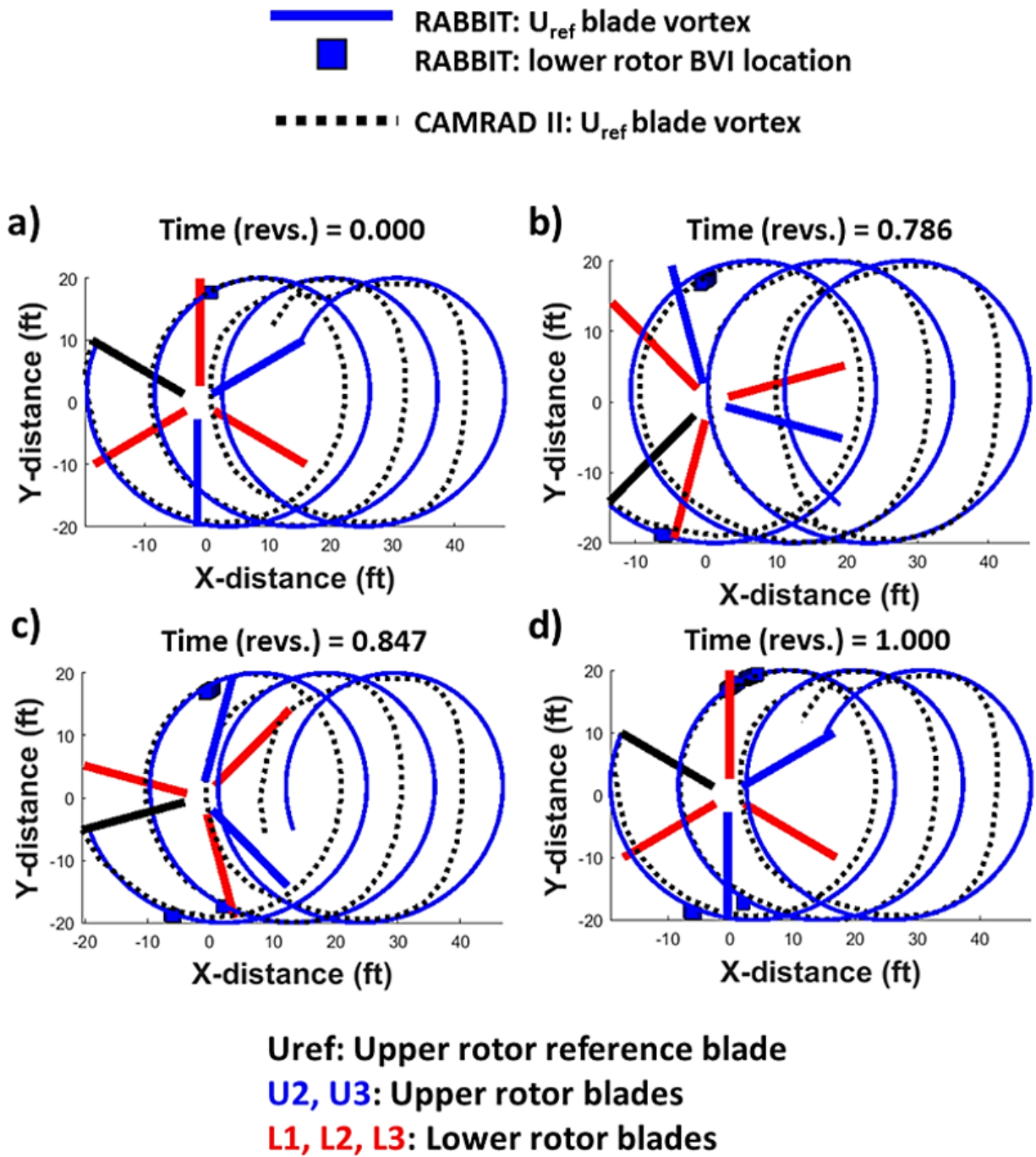
Figure 63. RABBIT versus CAMRAD II predictions for a six-bladed coaxial (three upper/ three lower) rotor blade crossing time and BVI lower rotor locations for U_{ref} at time of a) 0.000, b) 0.786, c) 0.847, and d) 1.000 revs. ( V_{tip} = 625 ft/s, \mu = 0.0867 , and S = 2.0 ft, \chi_{TPP} = 89.6^\circ , C_T = 0.0025 , \alpha_S = 10.00^\circ ).
