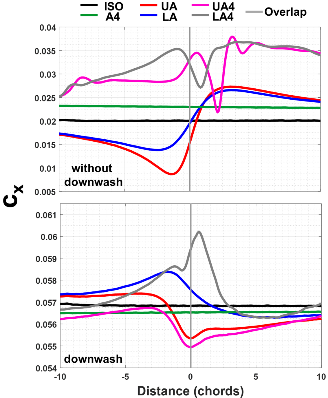
Figure 28. Viscid isolate airfoil, two airfoils crossing at crossing ( UA/LA ), single train of eight airfoils ( A4 ), and two trains of eight airfoils at crossing ( UA4/LA4 ) with and without downwash c_x versus distance ( M = 0.25 , \alpha = 9.8^\circ , V_i = 31 ft/s, S/c = 4.0 ( S = 2.0 ft, c = 0.5 ft), and D/c = 33.51 ).
