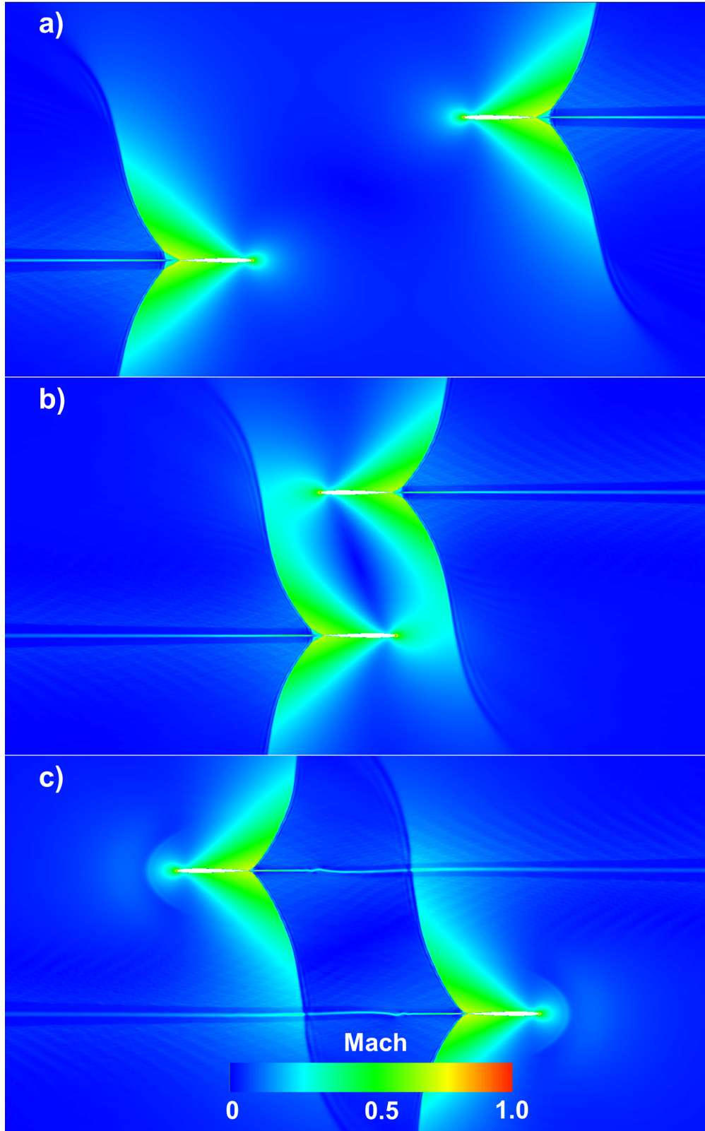
Figure 23. Mach contour of two airfoils crossing a) before, b) at, and c) after overlap ( M = 0.90 , \alpha = 0^\circ , and S/c = 4.0 ( S = 2.0 ft, c = 0.5 ft)).
