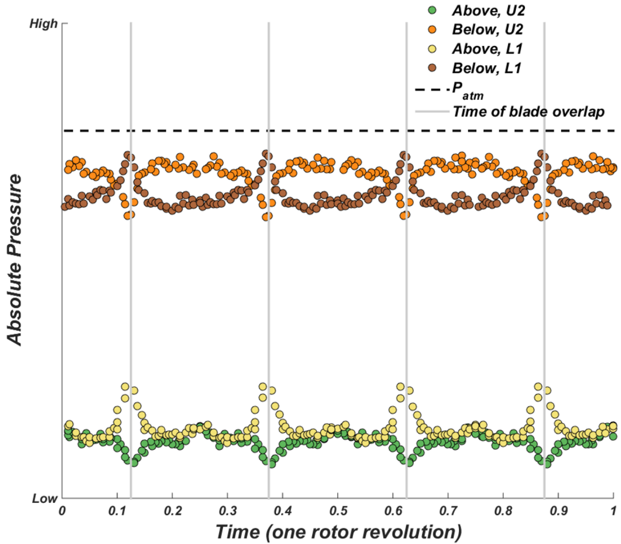
Figure 49. Time history (one revolution) at r/R = 0.85 for absolute pressure below and above U2 (upper rotor blade two) and L1 (lower rotor blade one) in hover.
