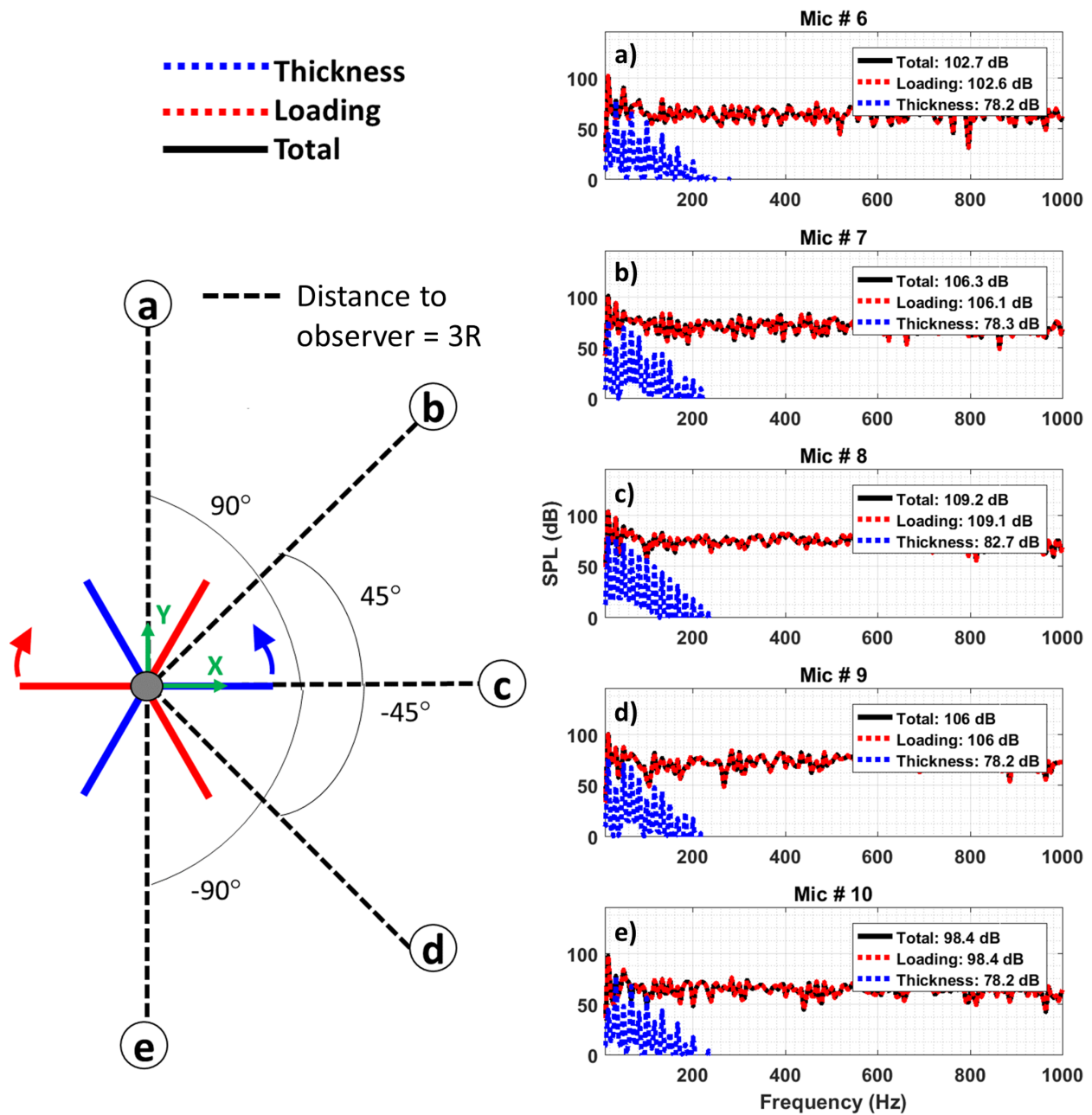
Figure 76. Azimuthal acoustic directivity in hover for coaxial modern rotor frequency spectrum.
