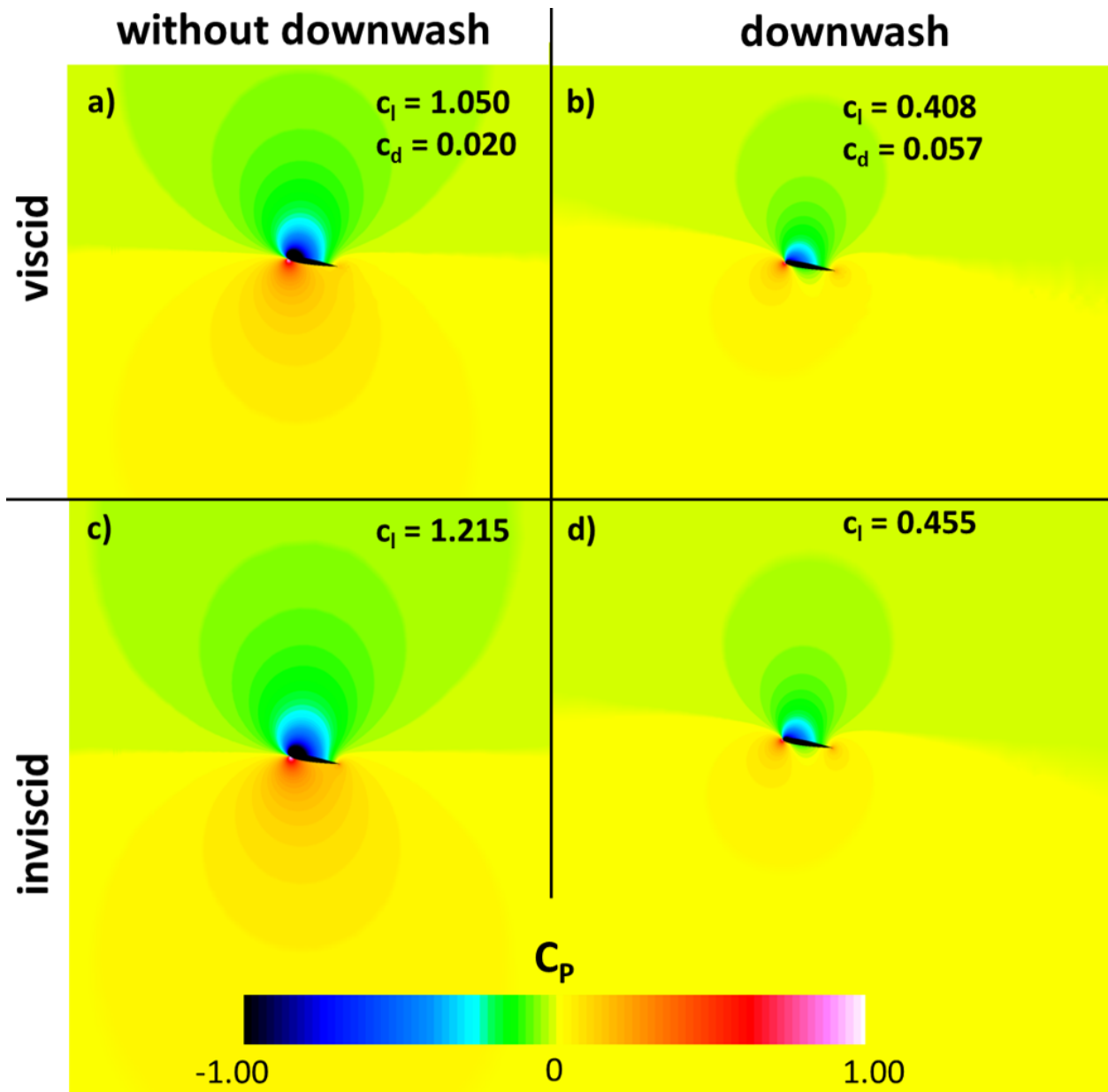
Figure 31. An isolated NACA 0012 airfoil C_p contour for a) viscid no downwash, b) viscid with downwash, c) inviscid, no downwash, and d) inviscid, downwash simulation ( M = 0.25 ( V_{tip} = 280 ft/s), \alpha = 9.8^\circ , V_i = 31 ft/s). Note: abrupt changes in contour levels is due to changing grid densities and numerical issues.
