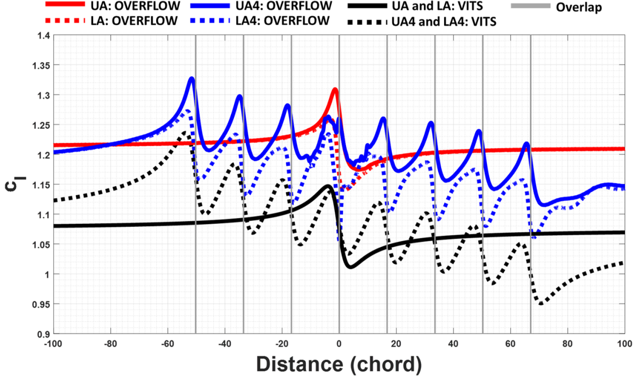
Figure 24. VITS (inviscid) and OVERFLOW (inviscid) calculations of two airfoils and two trains of eight airfoils crossing, c_l versus distance to overlap in chords ( M = 0.25 , \alpha = 9.8^\circ , and S/c = 4.0 ( S = 2.0 ft, c = 0.5 ft), and D/c = 33.51 ).
