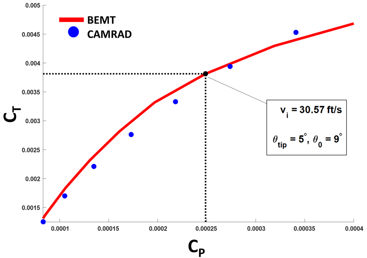
Figure 9. Coefficient of thrust versus coefficient of power for modern coaxial rotor in hover.
