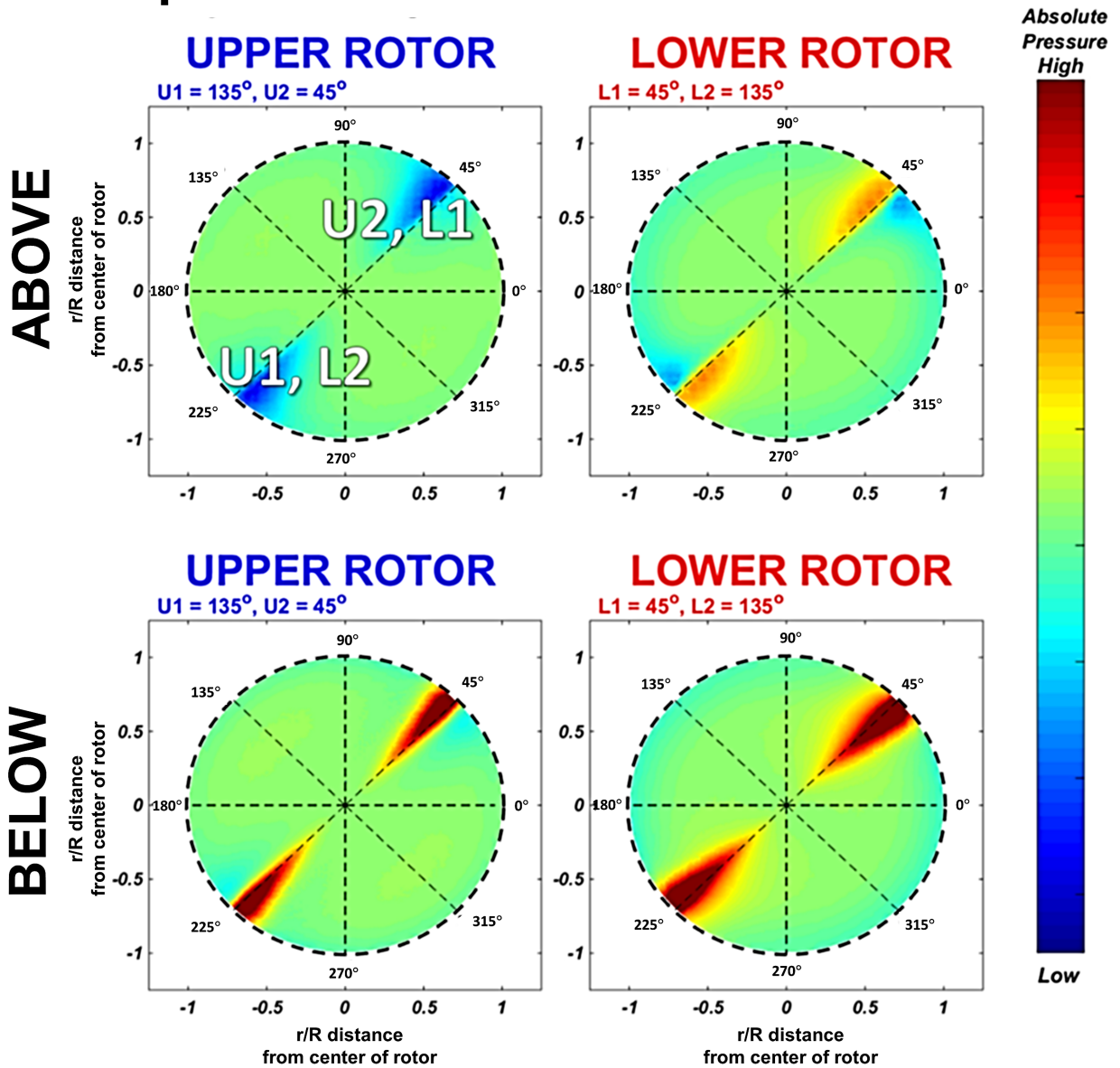
Figure 48. HC1 comparison of upper and lower rotor of absolute pressure below and above rotor, respectively, at overlap. RotUNS lifting-line (discrete-blade) rotor model calculations are presented for hover.
