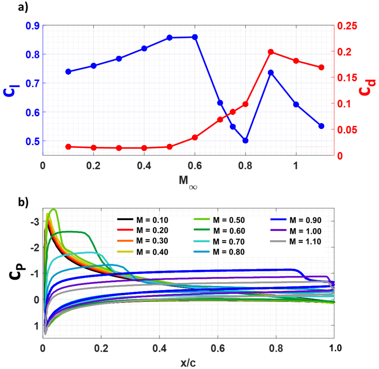
Figure 11. Viscid isolated NACA 0012 airfoil at \alpha = 7^\circ with a chord of 0.50 ft Mach number variation for a) c_l and c_d and b) C_P versus x/c .
