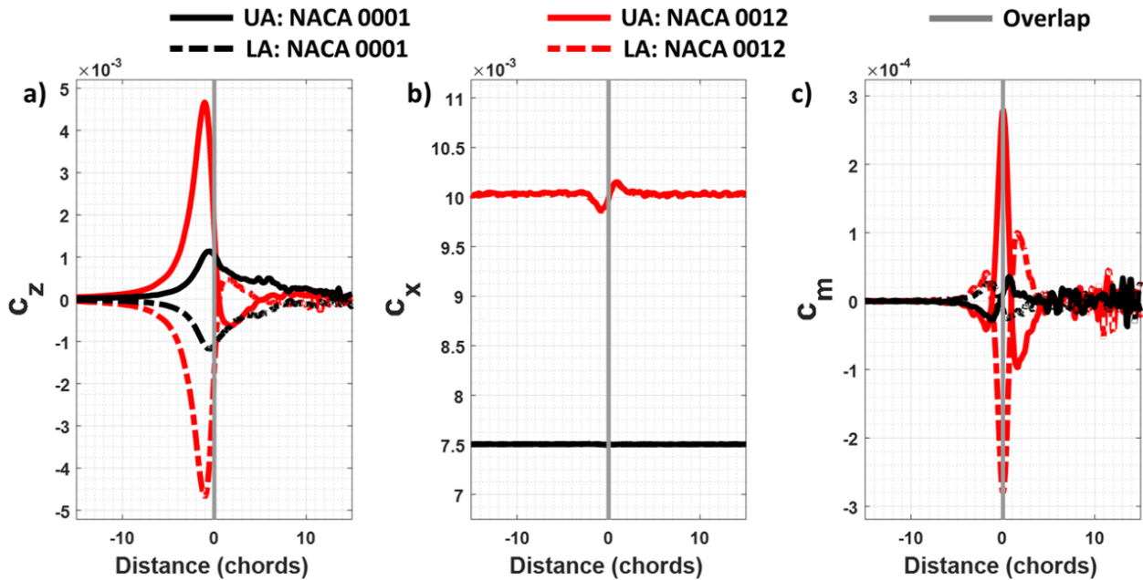
Figure 15. Comparison of two NACA 0001 and NACA 0012 airfoils crossing for a) c_z , b) c_x , and c) c_m versus distance to overlap ( M = 0.5 ( V_{tip} = 560 ft/s), \alpha = 0^\circ , and S/c = 4.0 ( S = 2.0 ft, c = 0.5 ft)).
