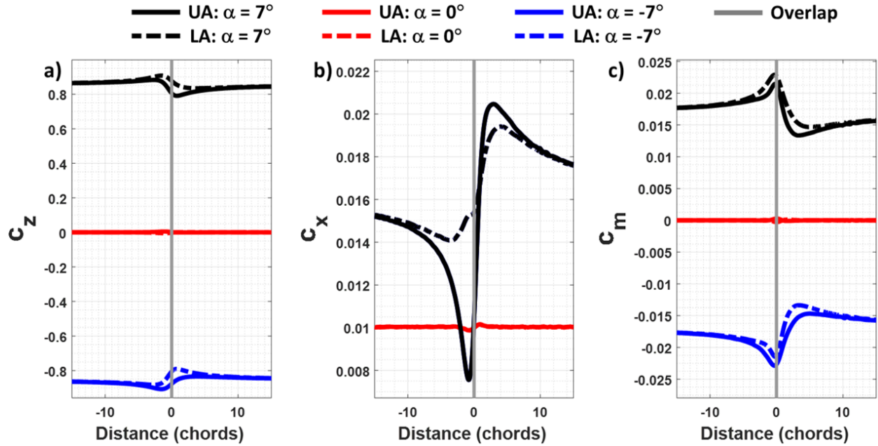
Figure 13. Two NACA 0012 airfoils crossing for a) c_z , b) c_x , and c) c_m versus distance to overlap ( M = 0.5 ( V_{tip} = 560 ft/s), \alpha = -7^\circ, 0^\circ , and 7^\circ , and S/c = 4.0 ( S = 2.0 ft, c = 0.5 ft)).
