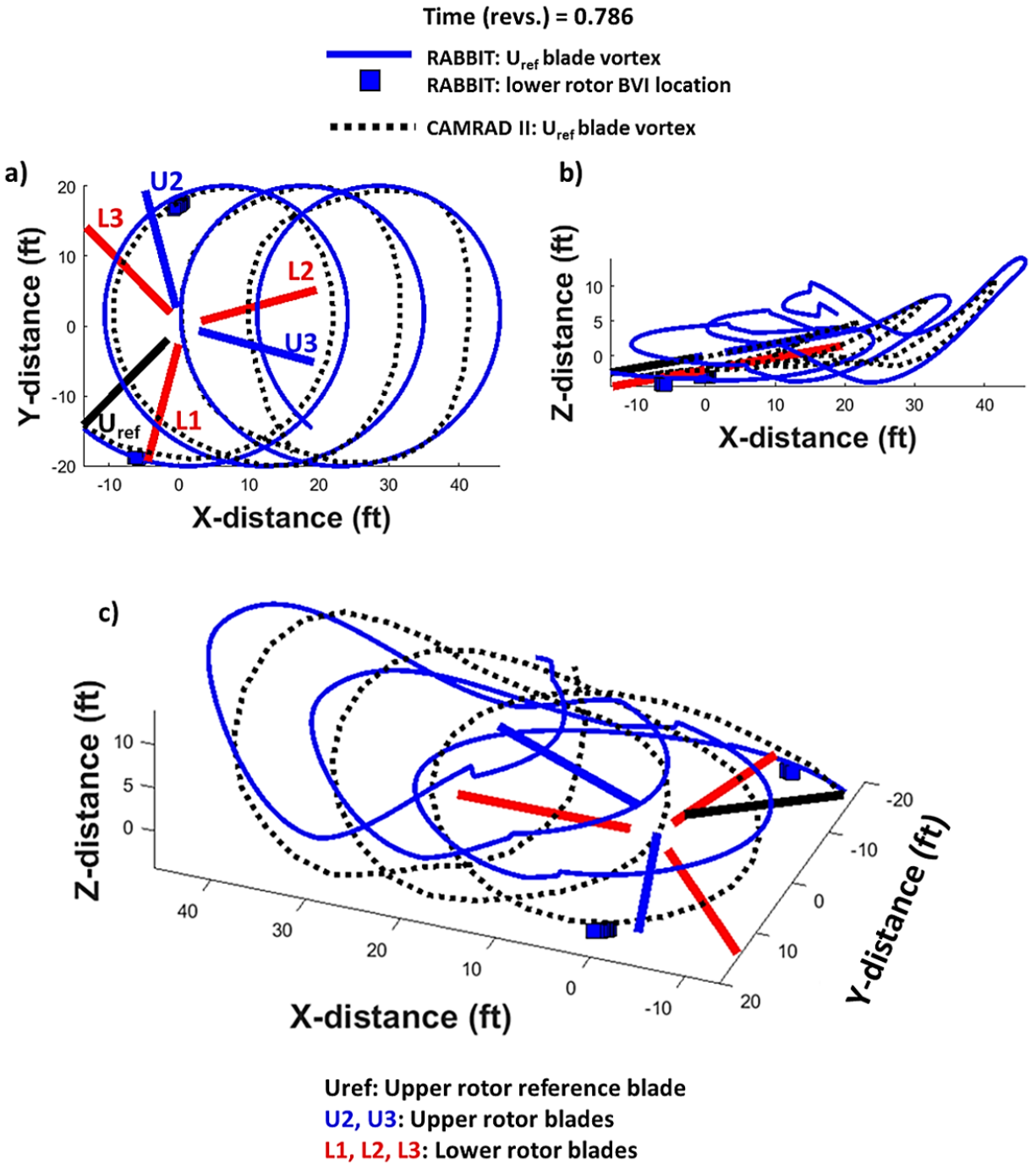
Figure 62. RABBIT versus CAMRAD II predictions for a six-bladed coaxial (three upper/ three lower) rotor wake comparison at time of 0.786 rev. ( U_{ref} ) ( V_{tip} = 625 ft/s, \mu = 0.0867 , and S = 2.0 ft, \chi_{TPP} = 89.6^\circ , C_T = 0.0025 , \alpha_S = 10.00^\circ ).
