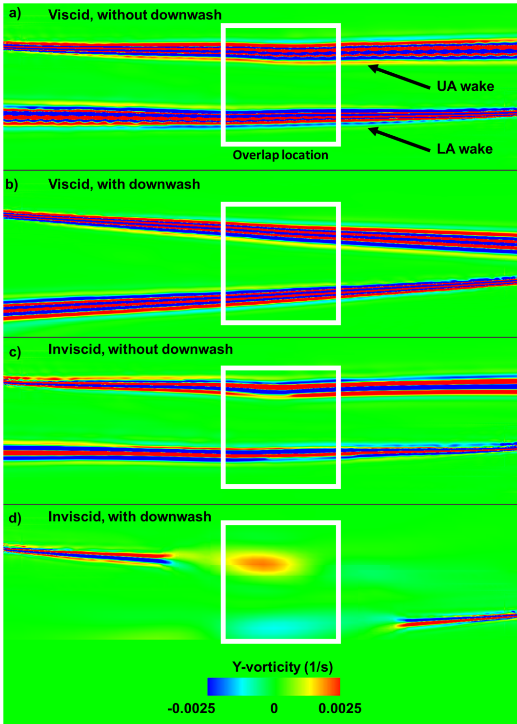
Figure 34. Two NACA 0012 airfoils y-vorticity contour after time of crossing for a) viscous no downwash, b) viscous with downwash, c) inviscid, no downwash, and d) inviscid, downwash simulation ( M = 0.25 ( V_{tip} = 280 ft/s), \alpha = 9.8^\circ , V_i = 31 ft/s, and S/c = 4.0 ( S = 2.0 ft, c = 0.50 )).
