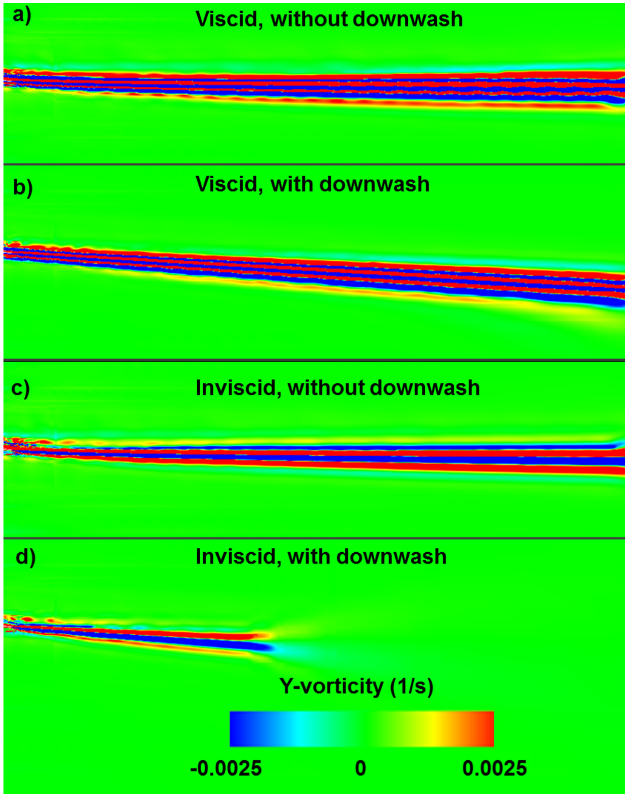
Figure 32. An isolated NACA 0012 airfoil wake y-vorticity contour for a) viscous no downwash, b) viscous with downwash, c) inviscid, no downwash, and d) inviscid, downwash simulation ( M = 0.25 ( V_{tip} = 280 ft/s), \alpha = 9.8^\circ , V_i = 31 ft/s).
