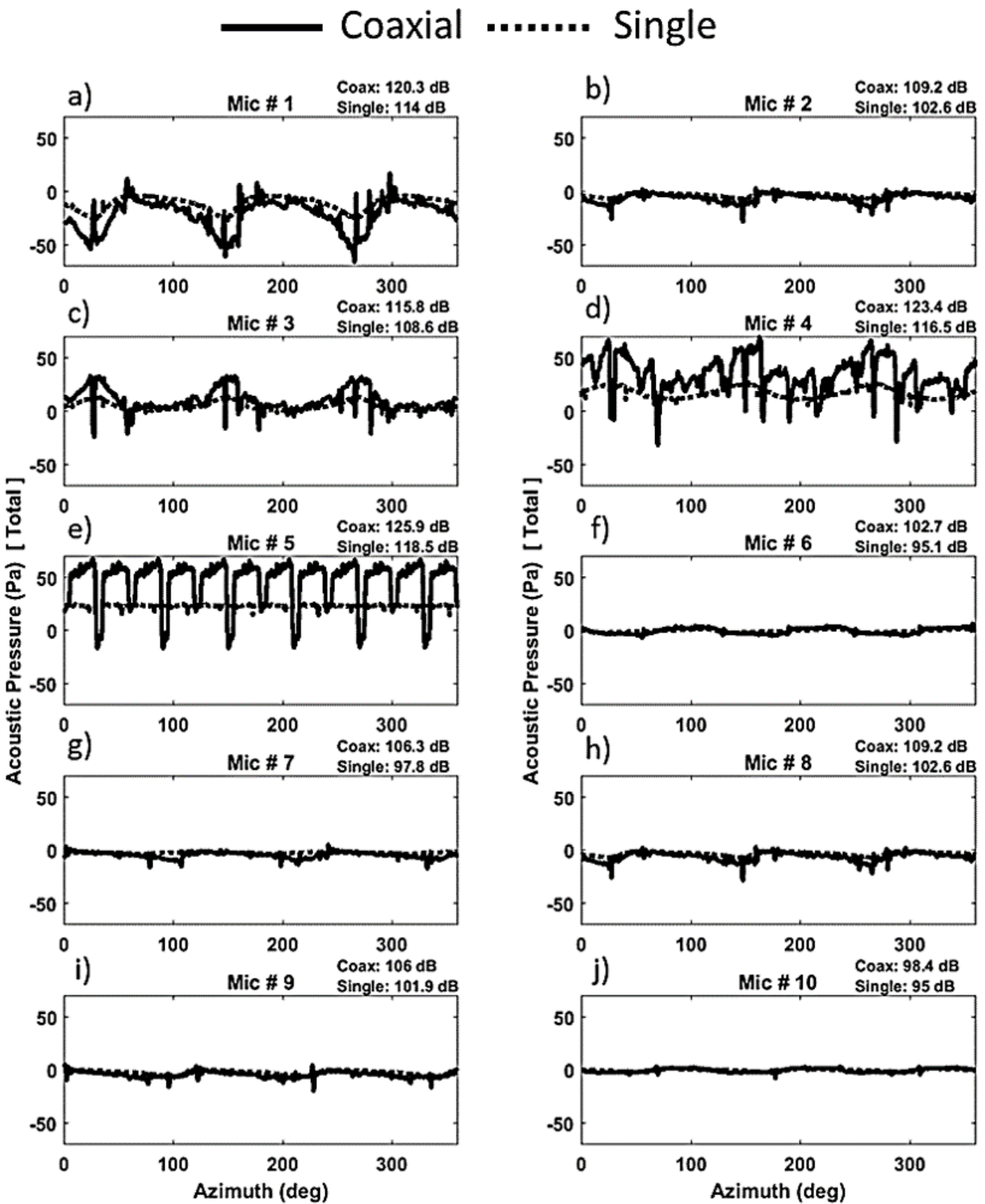
Figure 79. Single and coaxial modern rotor in hover. Total noise time history comparison for observers 1 through 10.
