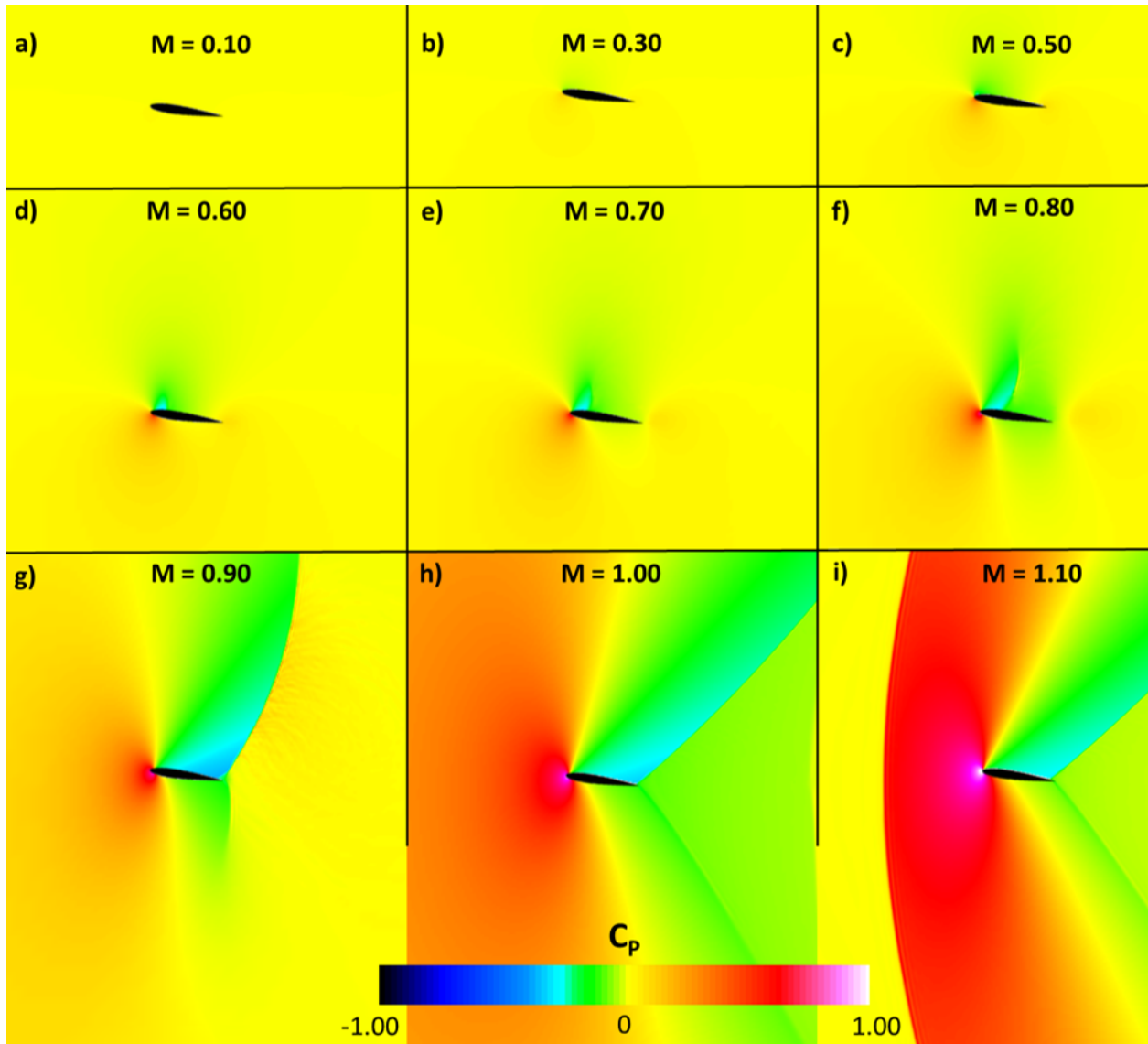
Figure 12. C_p flow field contours for Mach number variation for an isolated NACA 0012 airfoil at \alpha = 7^\circ M = a) 0.10, b) 0.30, c) 0.50, d) 0.60, e) 0.70, f) 0.80, g) 0.90, h) 1.0, and i) 1.1
