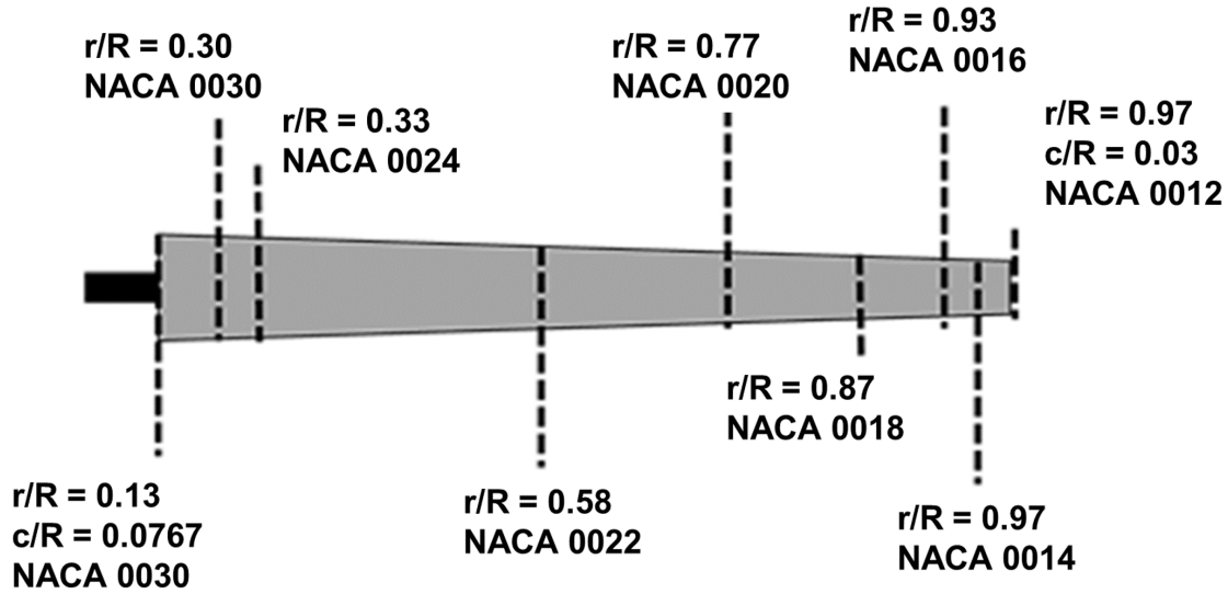
Figure 41. HS1/HC1 blade planform geometry as modeled in RotUNS.
