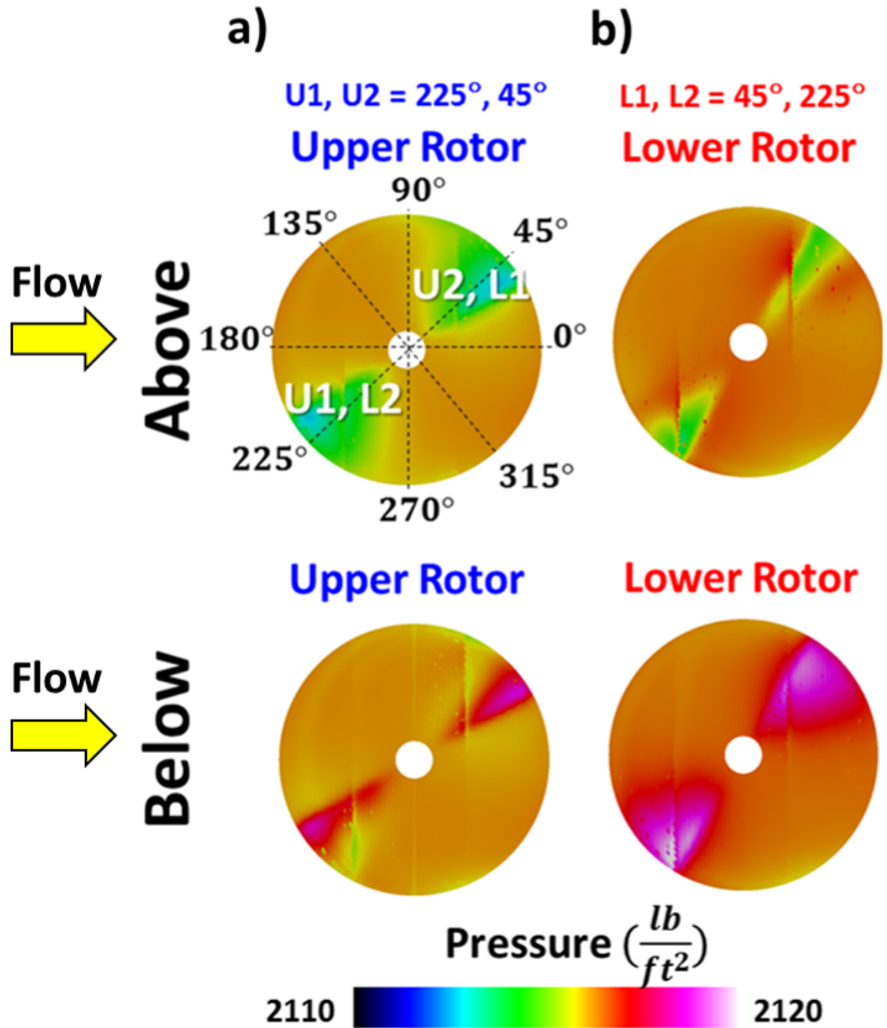
Figure 51. HC1 flow field absolute pressures below and above rotor at two instances in time when blades are overlapped for a) upper rotor where U1, U2 = 225^\circ, 45^\circ and b) lower rotor, where L1, L2 = 45^\circ, 225^\circ (RotUNS forward flight lifting-line (discrete blade) rotor model calculations) in forward flight ( \mu = 0.12 ).
