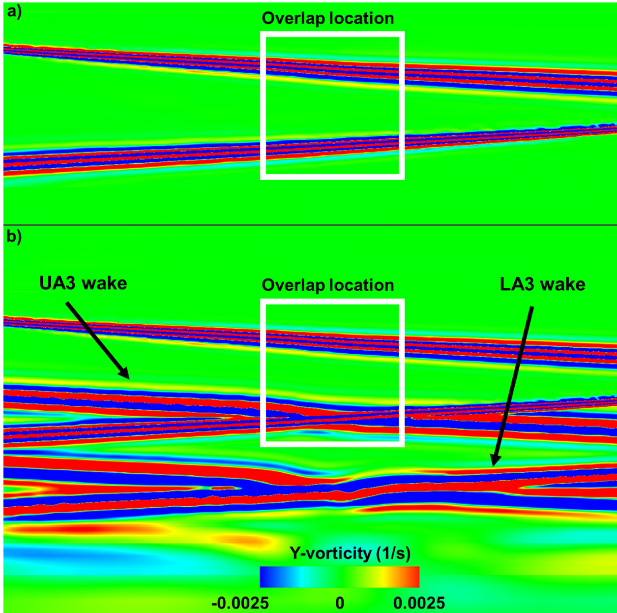
Figure 38. Vorticity contour with downwash viscous simulation of a) two airfoils ( UA/LA ) crossing and b) two trains of eight airfoils crossing after time of overlap of upper and lower airfoil four ( UA4/LA4 ) ( M = 0.25 , \alpha = 9.8^\circ , V_i = 31 ft/s, S/c = 4.0 ( S = 2.0 ft, c = 0.5 ft), and D/c = 33.51 ).
