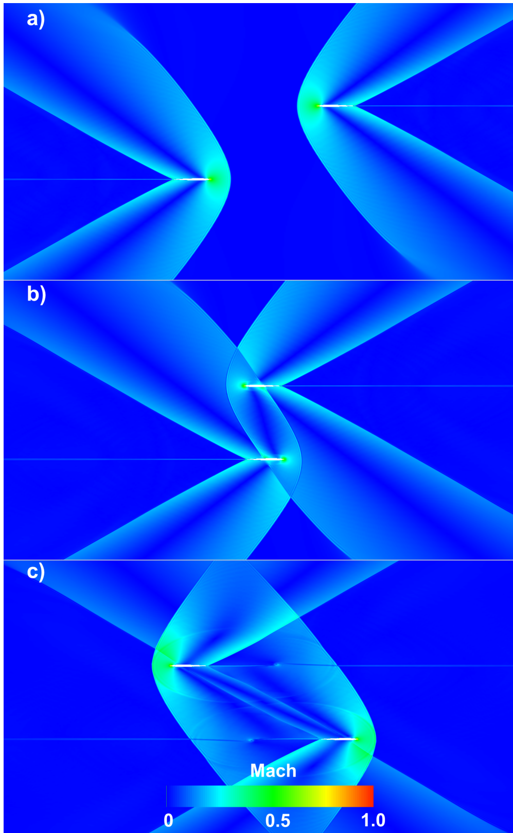
Figure 22. Mach contour of two airfoils crossing a) before, b) at, and c) after overlap ( M = 1.2 , \alpha = 0^\circ , and S/c = 4.0 ( S = 2.0 ft, c = 0.5 ft)).
