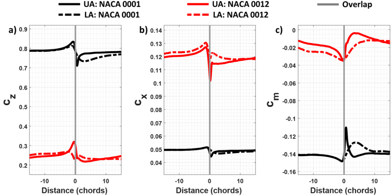
Figure 18. Comparison of two NACA 0001 and NACA 0012 airfoils crossing for a) c_z , b) c_x , and c) c_m versus distance to overlap ( M = 0.9 ( V_{tip} = 1,005 ft/s), \alpha = 3^\circ , and S/c = 4.0 ( S = 2.0 ft, c = 0.5 ft)).
