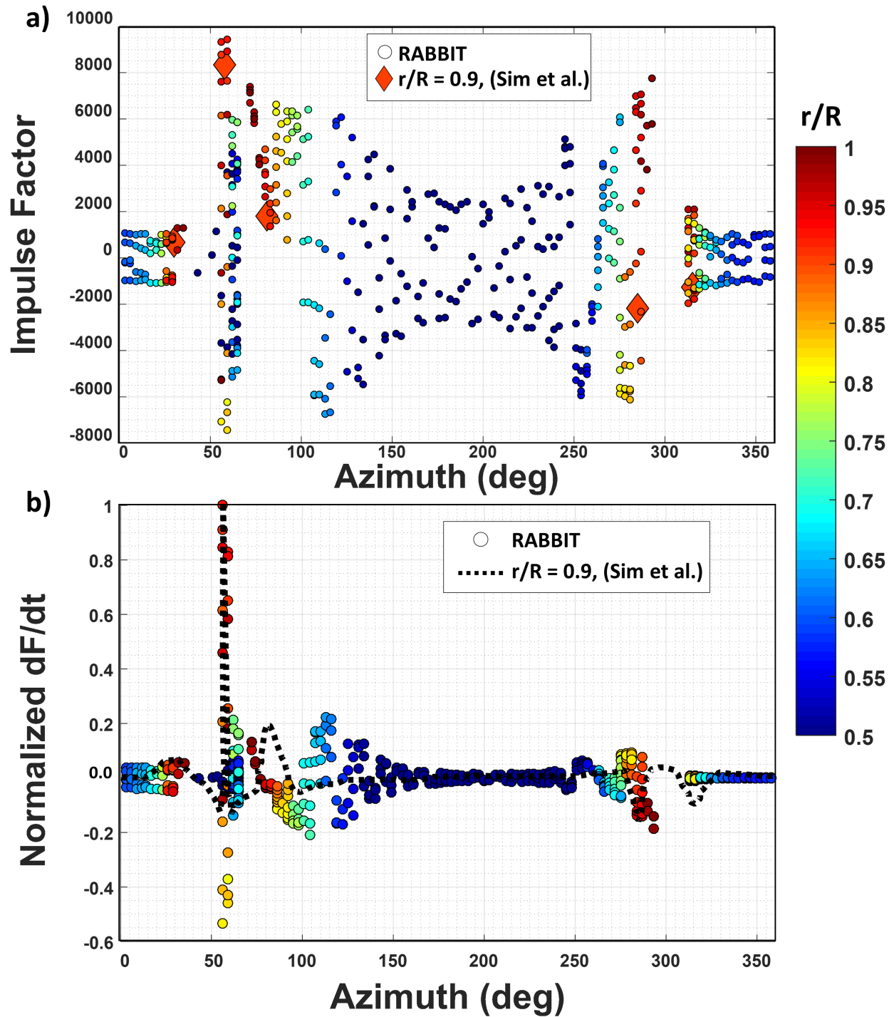
Figure 60. RABBIT and Sim et al., case study comparison of a) impulse factor versus azimuth angle and b) normalized \frac{\partial F}{\partial t} versus azimuth angle for r/R locations.
