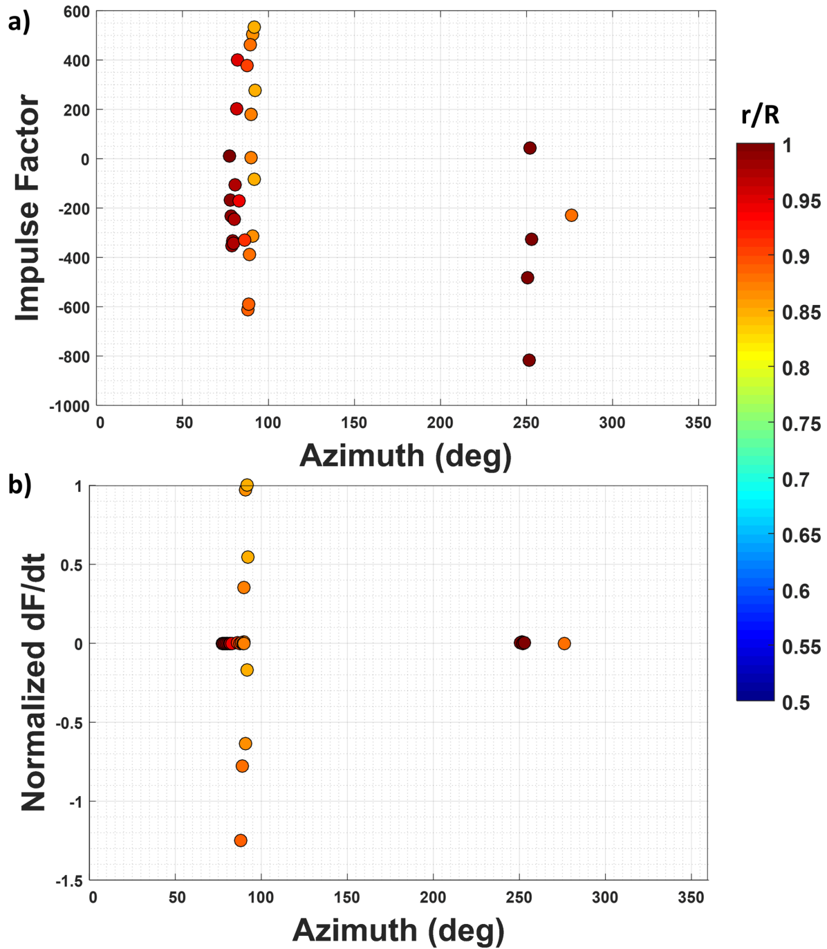
Figure 64. RABBIT modern coaxial lower rotor BVI predictions for U_{ref} for a) impulse factor and b) normalized \frac{\partial F}{\partial t} versus azimuth angle for r/R locations ( V_{tip} = 625 ft/s, \mu = 0.0867 , and S = 2.0 ft, \chi_{TPP} = 89.6^\circ , C_T = 0.0025 , \alpha_S = 10.00^\circ ).
