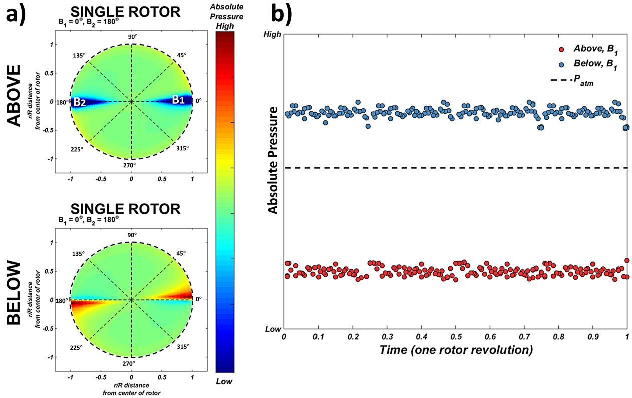
Figure 46. HS1 flow field absolute pressures a) below and above rotor and b) time history (one revolution) at r/R = 0.85 in hover (RotUNS lifting-line (discrete blade) rotor model calculations).
