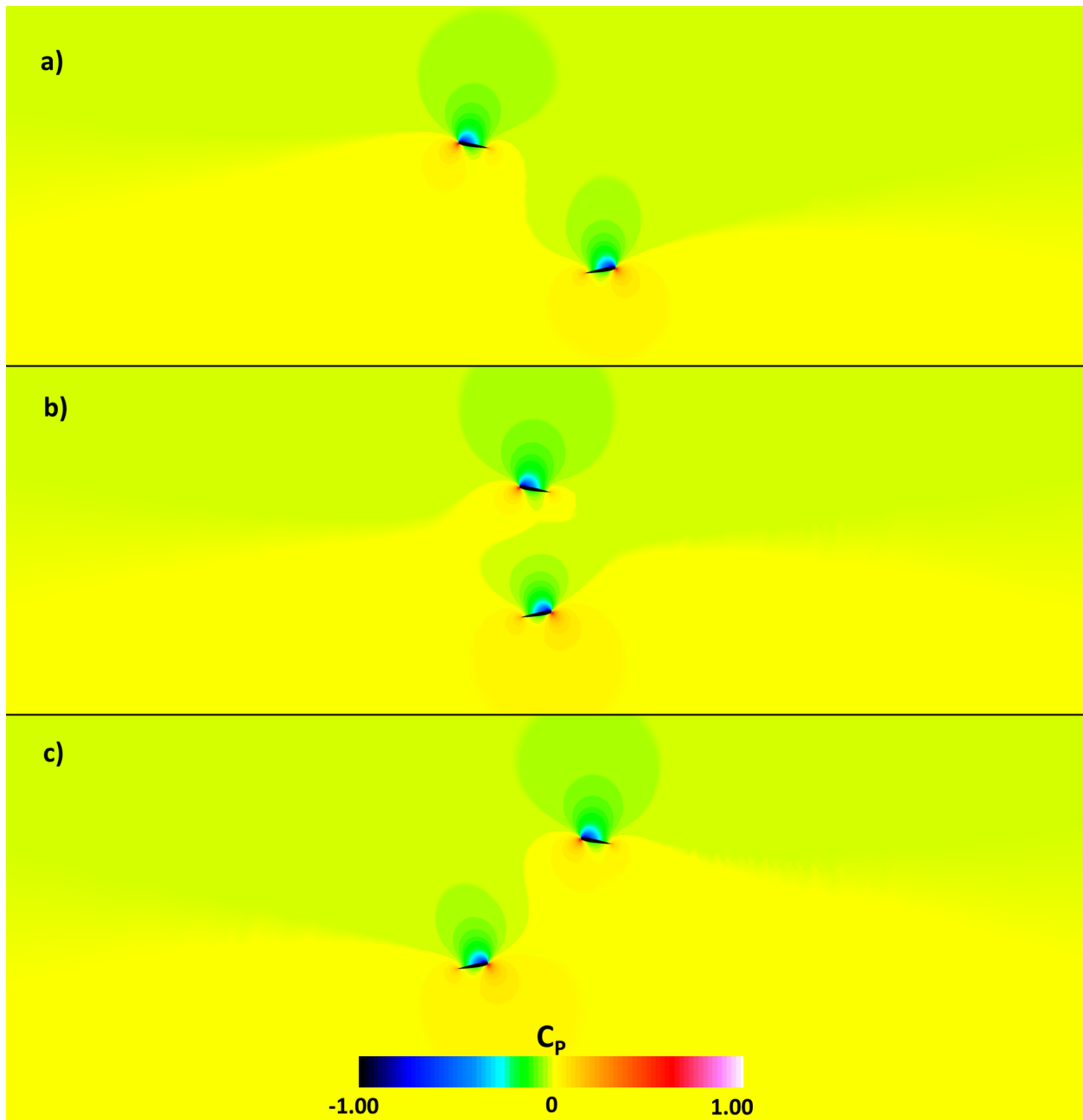
Figure 33. Viscid flow field C_p contour of two NACA 0012 airfoils crossing a) before, b) at, and c) after with downwash ( M = 0.25 ( V_{tip} = 280 ft/s), \alpha = 9.8^\circ , V_i = 31 ft/s, and S/c = 4.0 ( S = 2.0 ft, c = 0.5 ft)).
