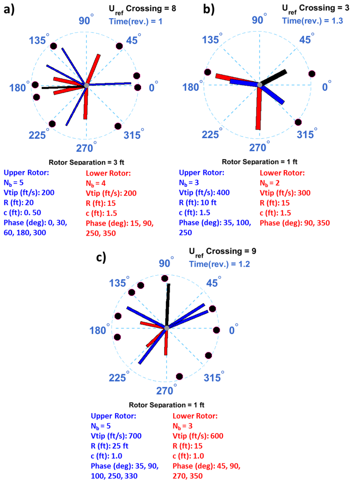
Figure 55. RABBIT's blade crossing predictions for three unconventional coaxial configurations.
