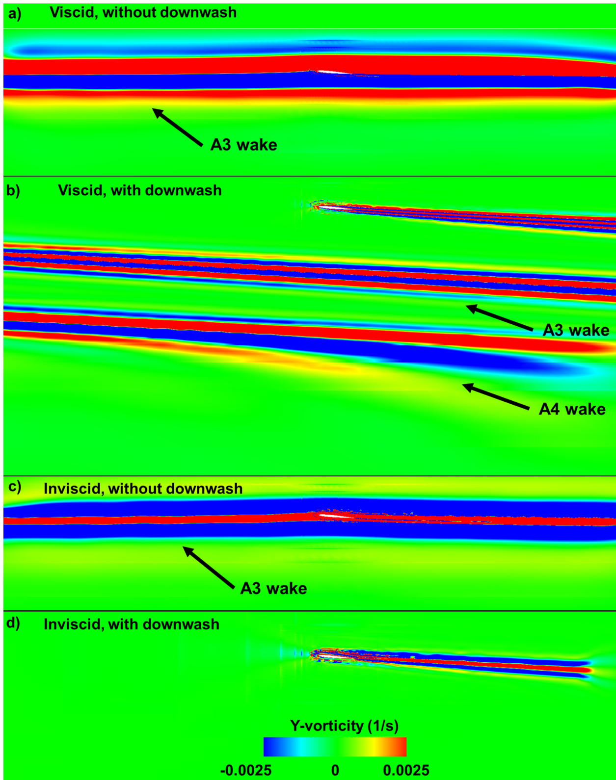
Figure 36. Vorticity contours for A4 (4th airfoil in a train of eight airfoils) for a) viscous no downwash, b) viscous with downwash, c) inviscid, no downwash, and d) inviscid, downwash simulation ( M = 0.25 , \alpha = 9.8^\circ , V_i = 31 ft/s, and D/c = 33.51 ).
