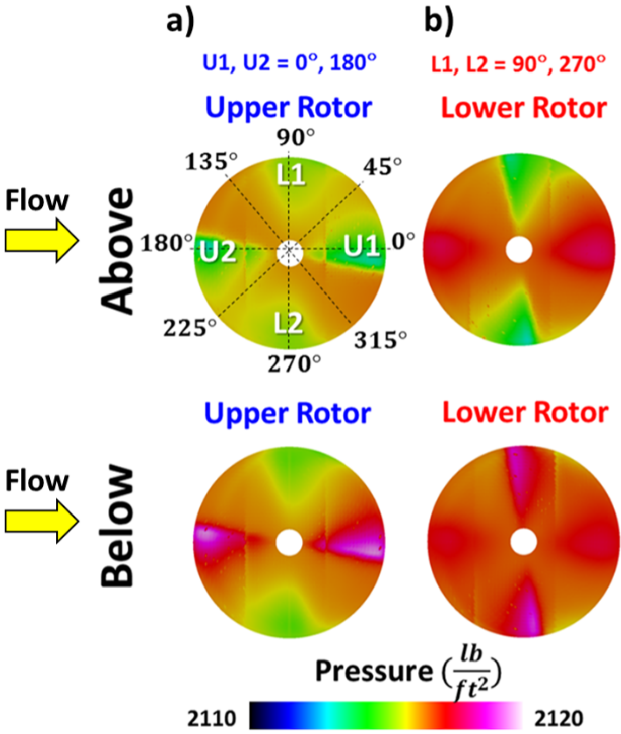
Figure 50. HC1 flow field absolute pressures below and above rotor at two instances in time when blades are not overlapped, for a) upper rotor where U1, U2 = 0^\circ, 180^\circ and b) lower rotor, where L1, L2 = 90^\circ, 270^\circ (RotUNS forward flight lifting-line (discrete blade) rotor model calculations) in forward flight ( \mu = 0.12 ).
