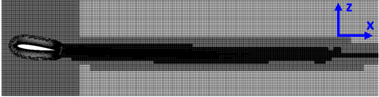
Figure 7. OVERFLOW 2.2k simulation with grid adaption for an NACA 0012 isolated airfoil at \alpha = 7^\circ .
