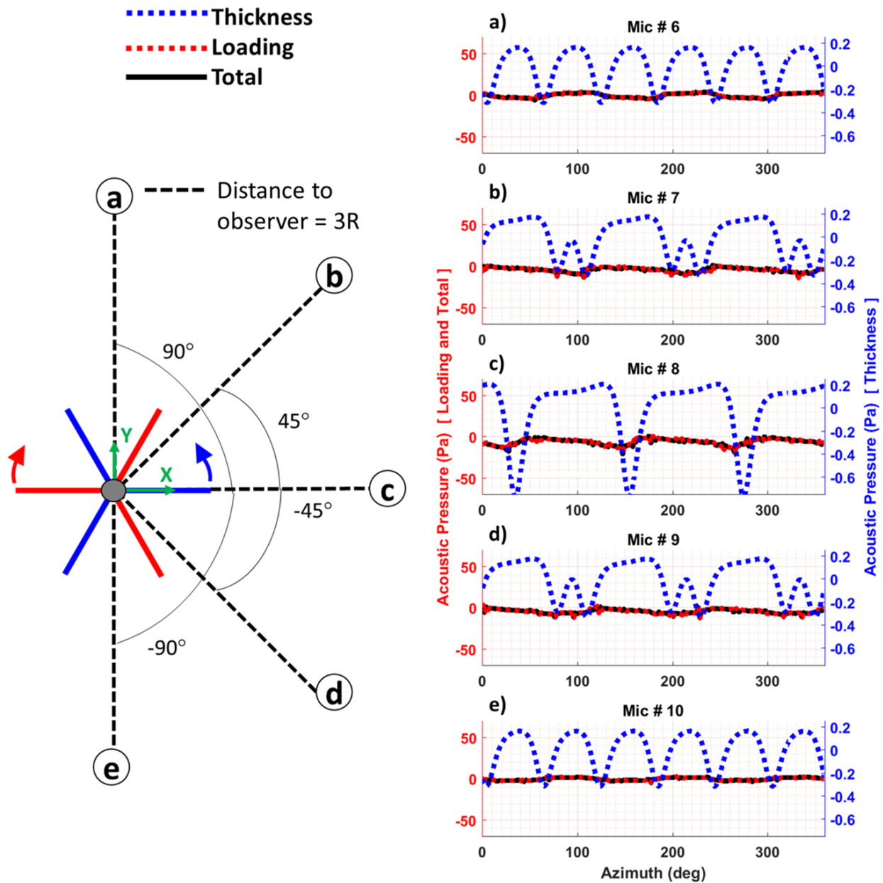
Figure 75. Azimuthal acoustic directivity in hover for coaxial modern rotor acoustic pressure time history. The left (red) y-axis corresponds to loading and total noise, and the right (blue) y-axis corresponds to thickness noise.
