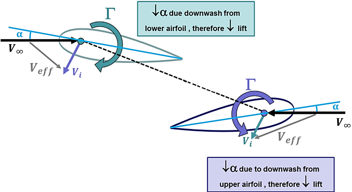
Figure 6. Change in lift of two NACA 0012 (when compressibility is not dominating) airfoils crossing: a) before and b) after.
