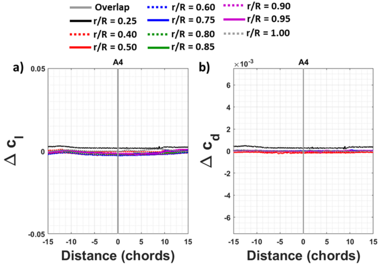
Figure 39. Modern single rotor in hover 2D representation for A4 a) \Delta c_l and b) \Delta c_d versus distance to overlap ( r/R = 0.25 through 1.00).
