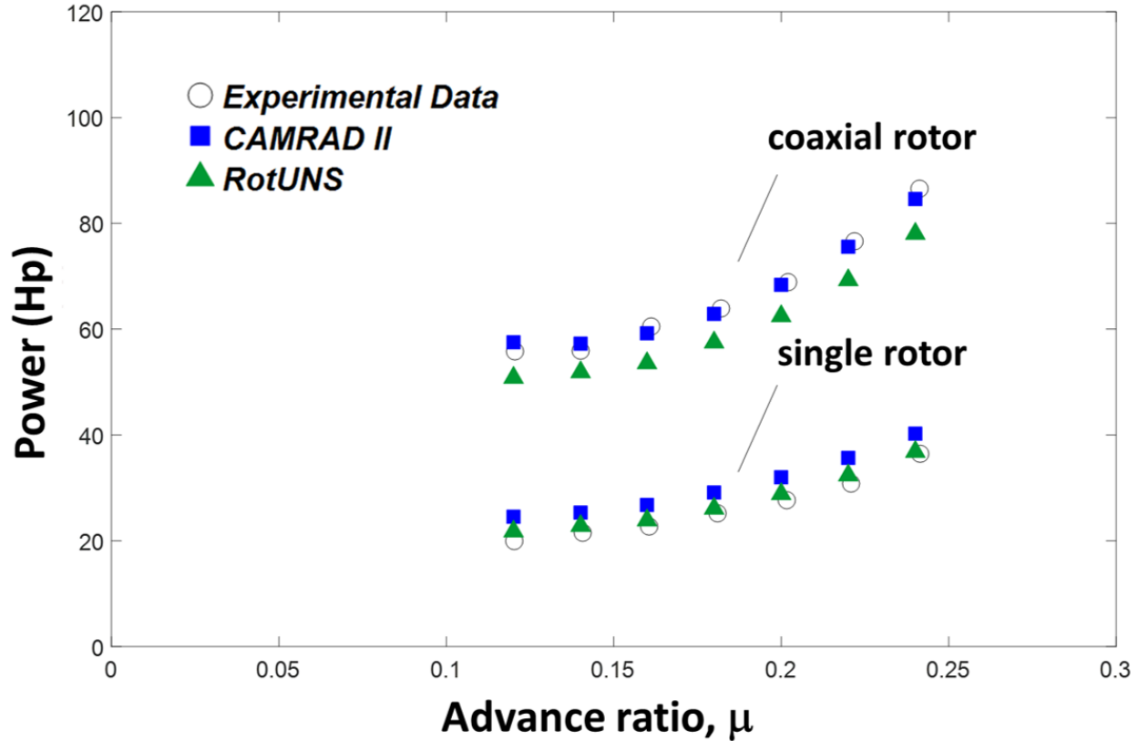
Figure 45. Measured performance of HS1 and HC1 [16] in forward flight compared with CAMRAD II and RotUNS calculations.
