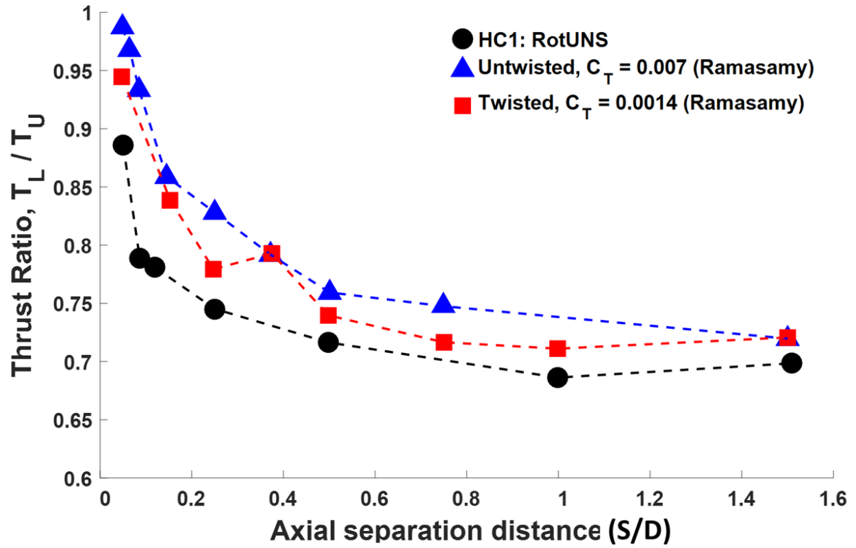
Figure 44. Thrust ratio versus rotor separation distance in hover comparing HC1 RotUNS rotor disk model calculations and Ramasamy’s [9] experimental data for untwisted blades.
