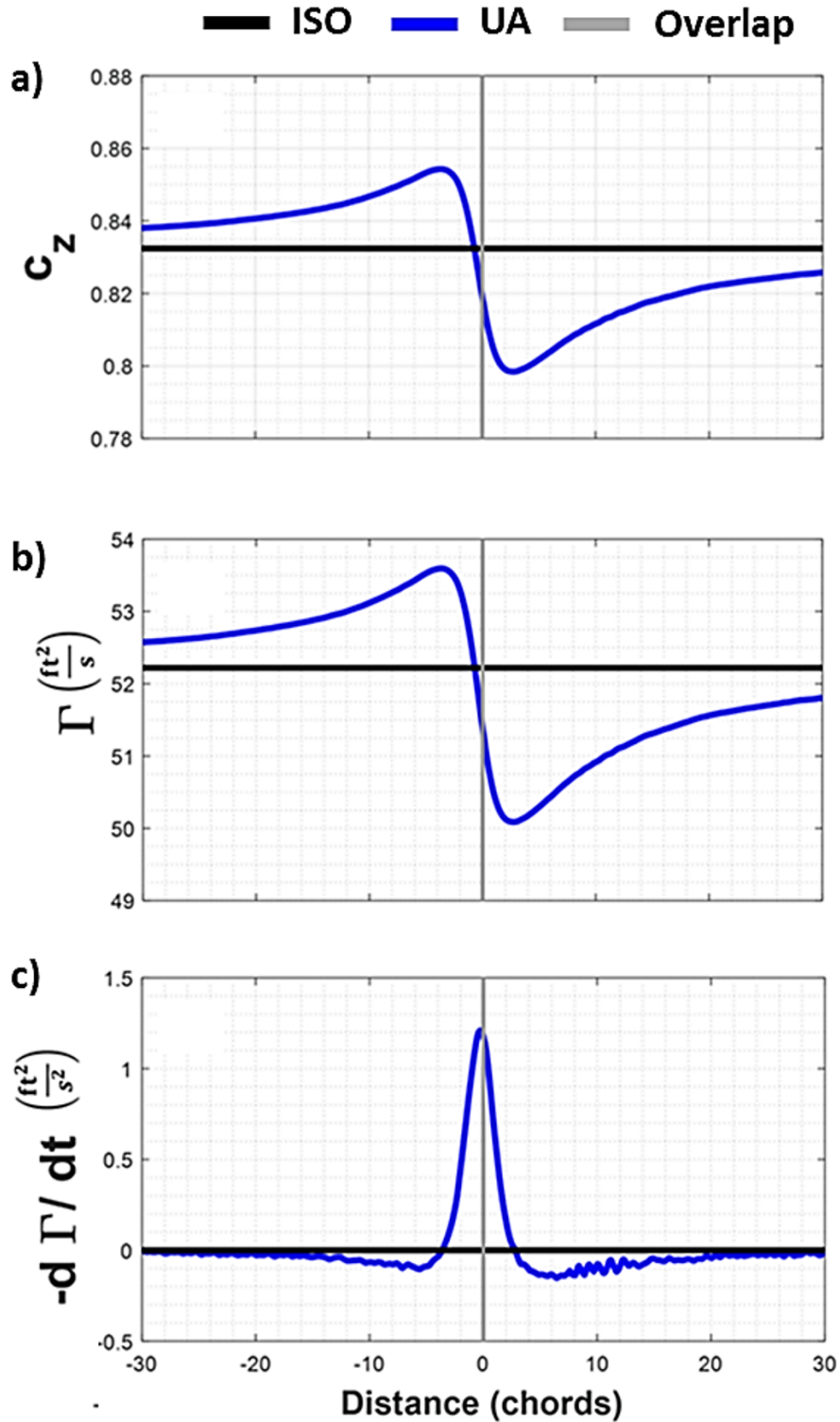
Figure 35. Results for an isolated airfoil and the upper airfoil of the two airfoils crossing case a) c_z , b) \Gamma , and c) -d\Gamma/dt . Horizontal axis is distance to overlap for the upper airfoil (UA) (HC1: M = 0.47 ( V_{tip} = 500 ft/s), \alpha = 7^\circ , and S/c = 6.21 ( S = 2.33 ft, c = 0.375 ft)).
