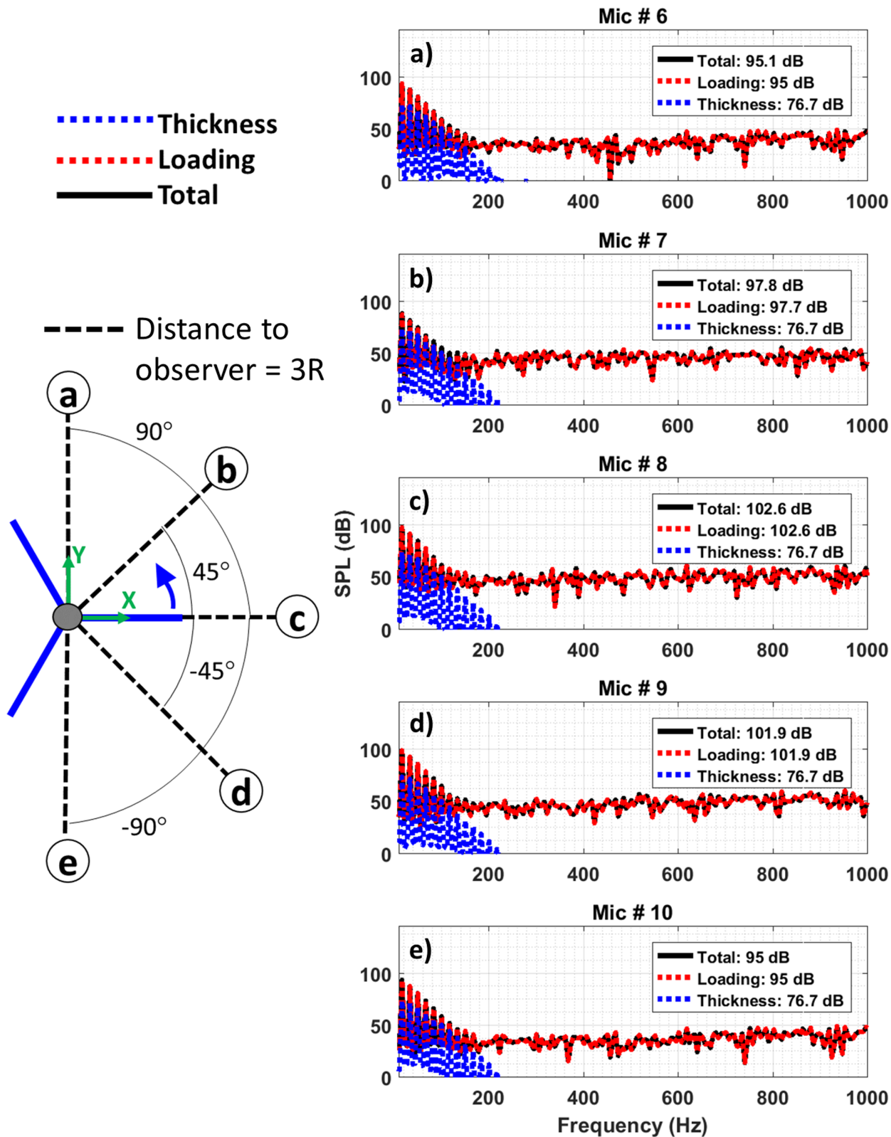
Figure 72. Azimuthal acoustic directivity in hover for single modern rotor frequency spectrum.
