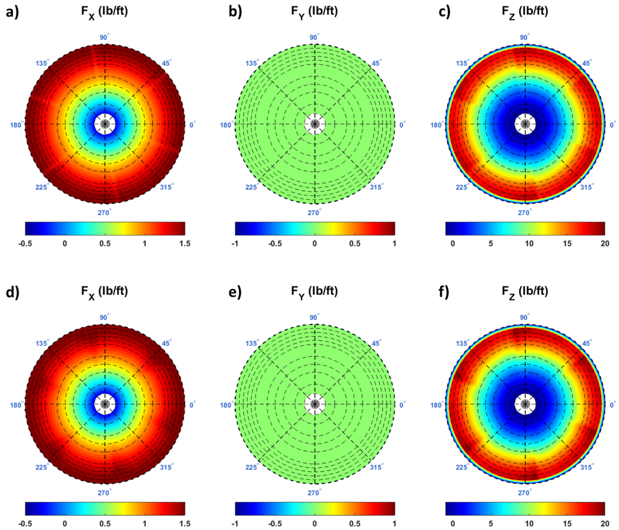
Figure 67. Stacked 2D OVERFLOW results for modern coaxial modern rotor in hover upper rotor a) F_X , b) F_Y and c) F_Z and lower rotor d) F_X , e) F_Y and f) F_Z .
