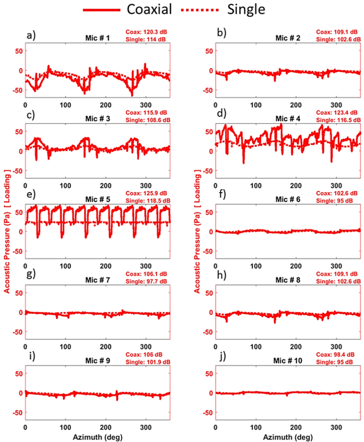
Figure 78. Single and coaxial modern rotor in hover. Loading noise time history comparison for observers 1 through 10.
