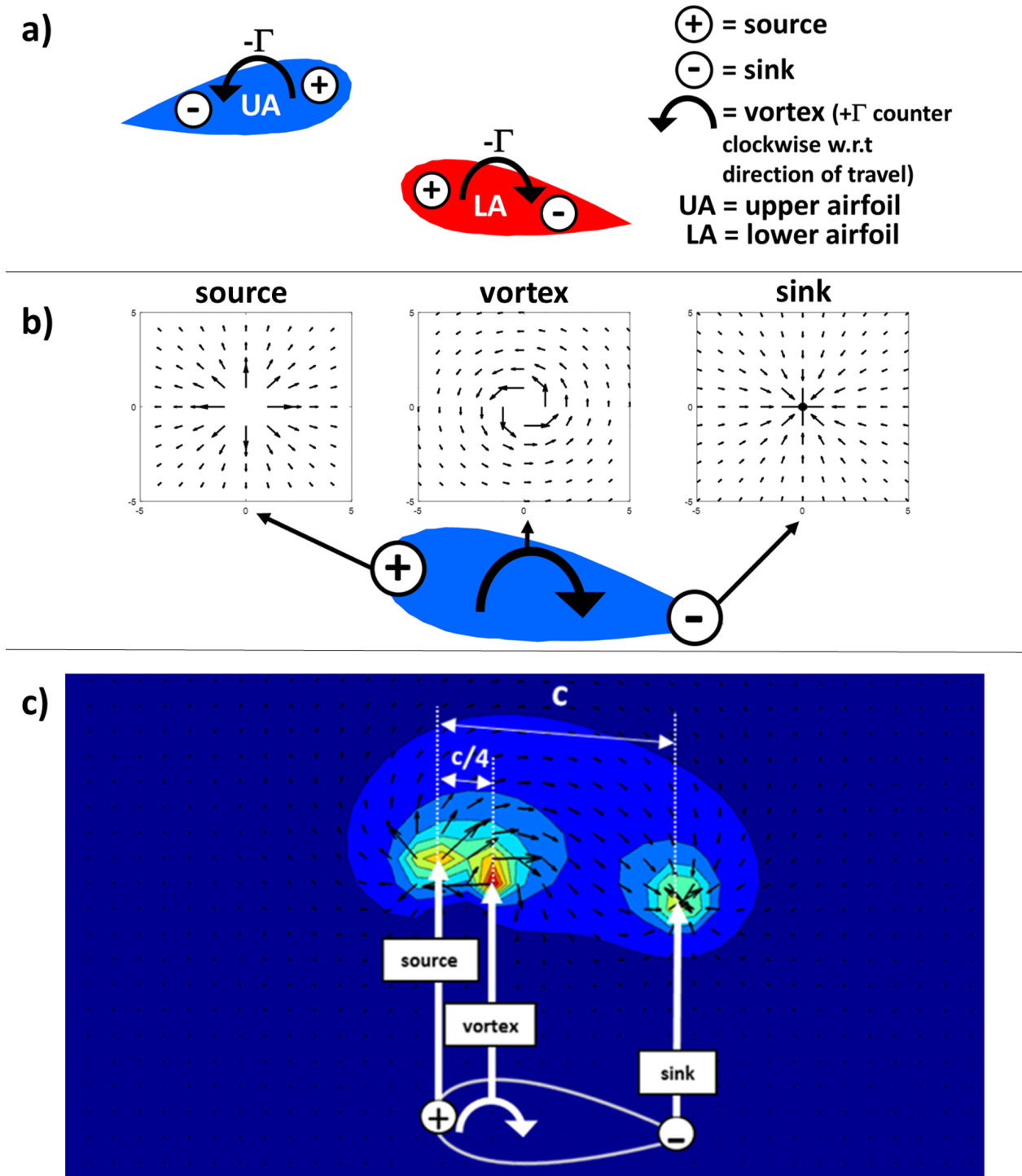
Figure 3. a) Pictorial representation of two airfoils moving past each other modeled by a source, sink, and vortex, b) mathematical model of an individual sink, vortex, and source and c) simulation of a combined sink, vortex, and source for an isolated airfoil.
