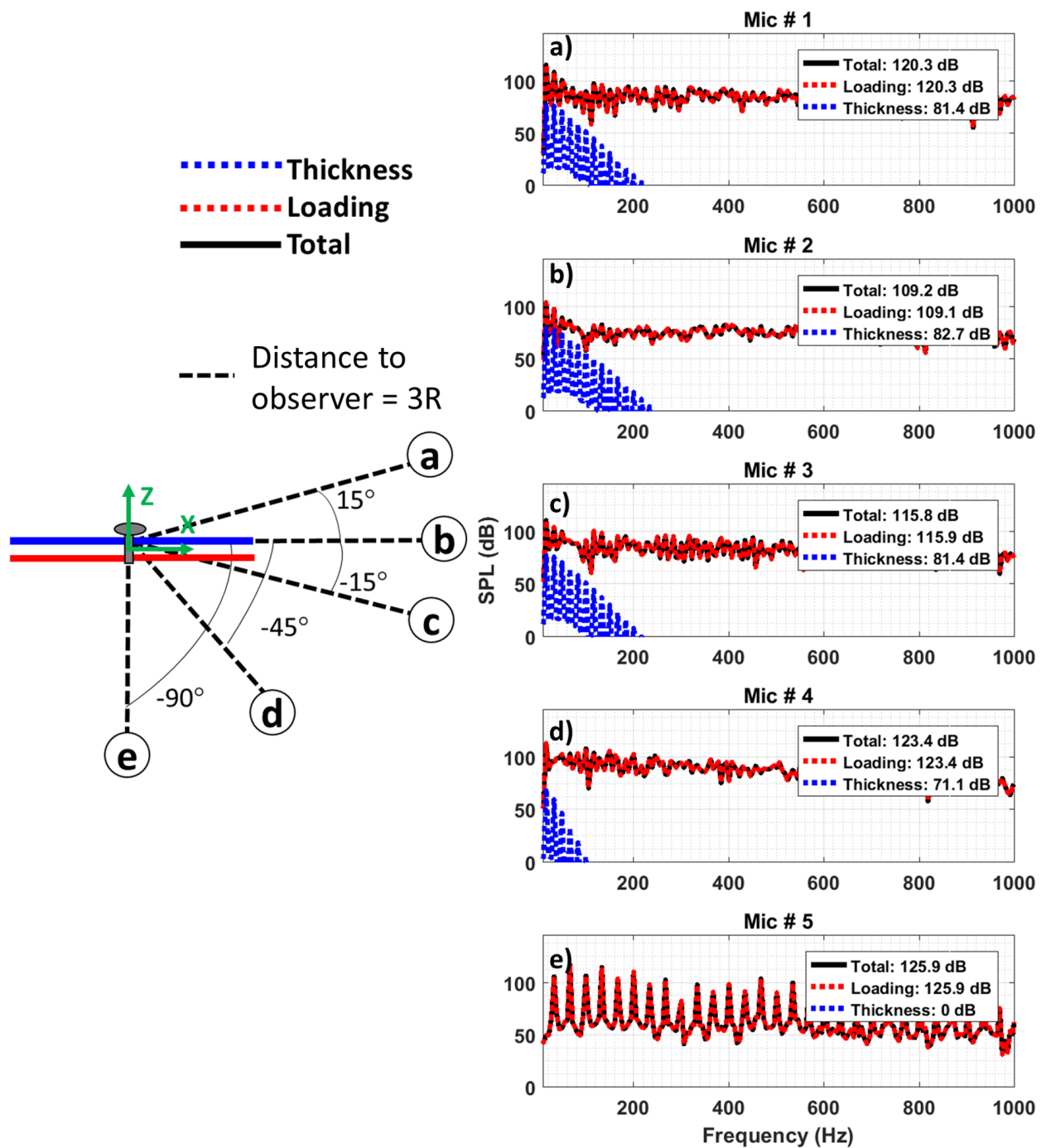
Figure 74. Elevation acoustic directivity in hover for coaxial modern rotor frequency spectrum.
