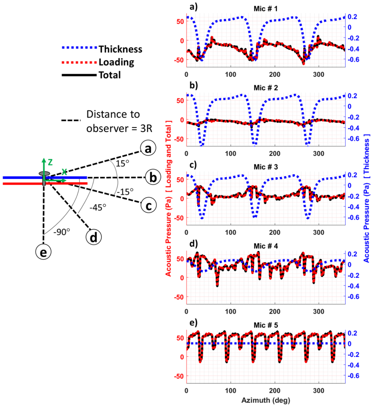
Figure 73. Elevation acoustic directivity in hover for coaxial modern rotor acoustic pressure time history. The left (red) y-axis corresponds to loading and total noise, and the right (blue) y-axis corresponds to thickness noise.
