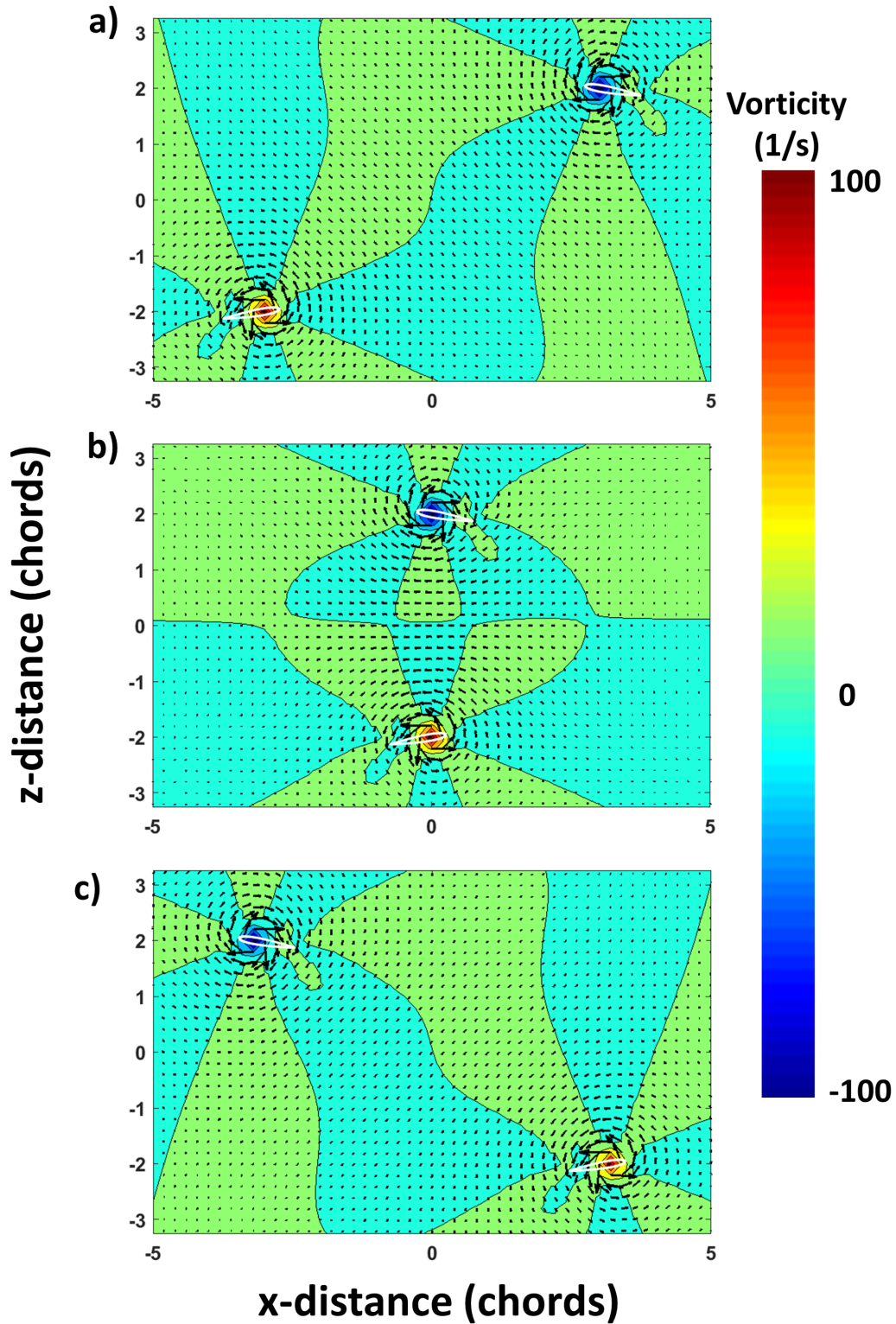
Figure 5. Simulation of two airfoils: a) before, b) at, and c) after time of crossing. Vorticity contour shown with u and v velocity vectors, downwash not simulated. ( M = 0.25 , \alpha = 9.8^\circ , and S/c = 4.0 ( S = 2.0 ft, c = 0.5 ft)).
