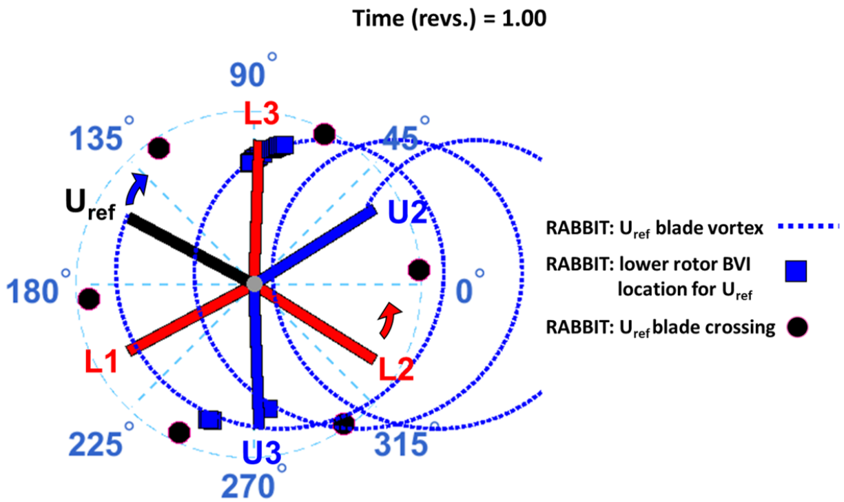
Figure 61. RABBIT blade crossing and lower rotor BVI predictions for a six-bladed (three upper/three lower) coaxial rotor ( V_{tip} = 625 ft/s, \mu = 0.0867 , and S = 2.0 ft, \chi_{TPP} = 89.6^\circ , C_T = 0.0025 , \alpha_S = 10.00^\circ ).
