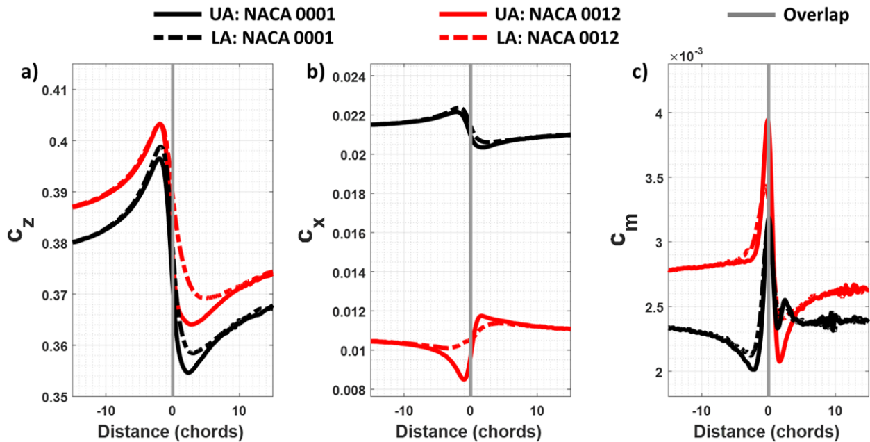
Figure 17. Comparison of two NACA 0001 and NACA 0012 airfoils crossing for a) c_z , b) c_x , and c) c_m versus distance to overlap ( M = 0.5 ( V_{tip} = 560 ft/s), \alpha = 3^\circ , and S/c = 4.0 ( S = 2.0 ft, c = 0.5 ft)).
