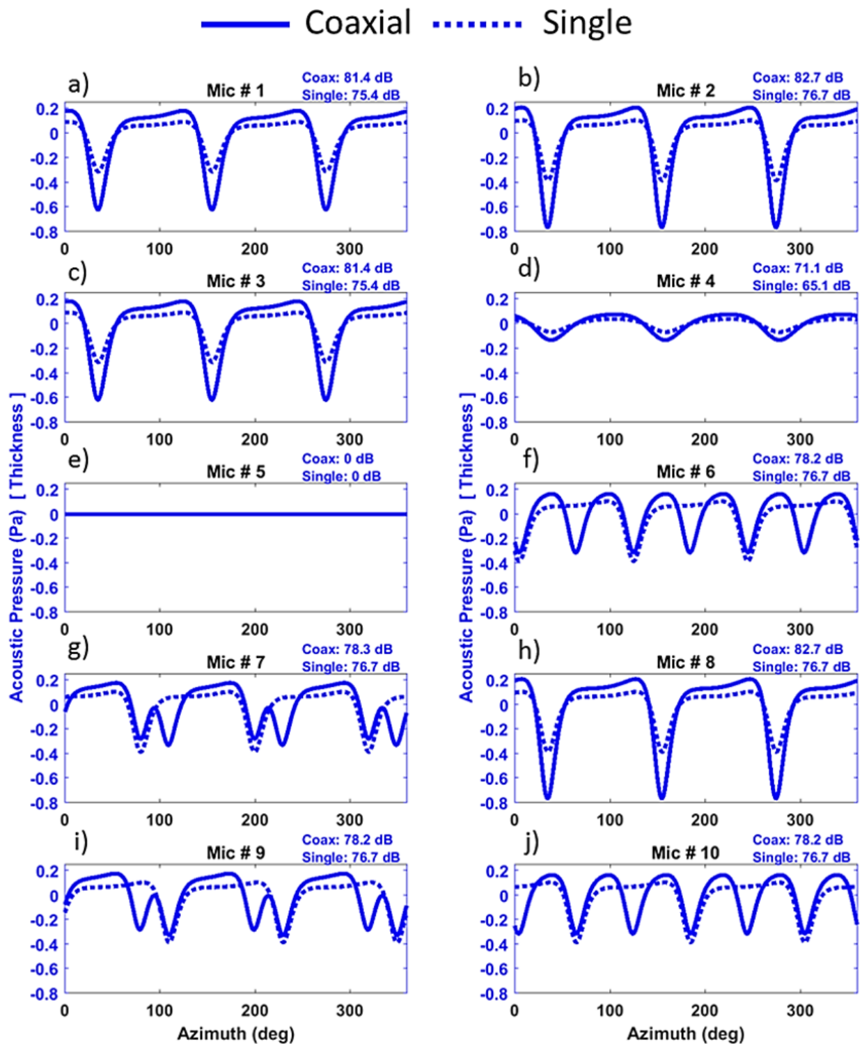
Figure 77. Single and coaxial modern rotor in hover. Thickness noise time history comparison for observers 1 through 10.
