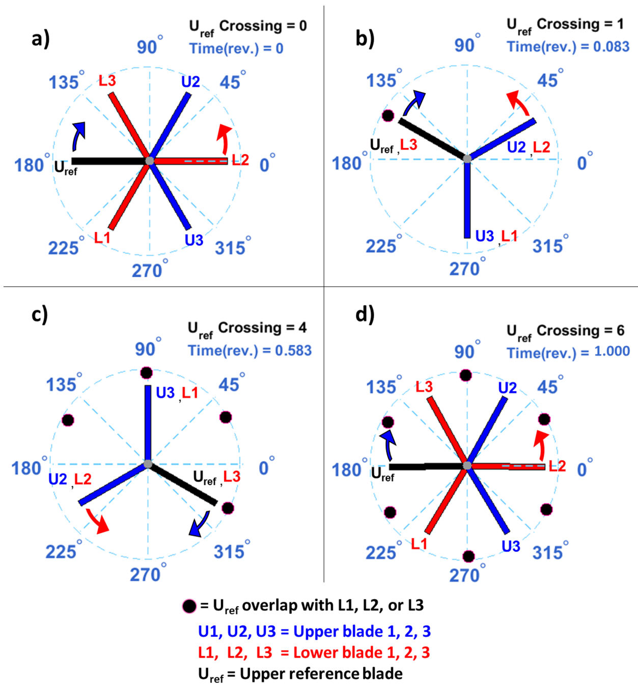
Figure 54. RABBIT's predictions for a six-bladed coaxial rotor blade crossing time and locations ( V_{tip} = 625 ft/s, \mu = 0.10 , and S = 2.0 ft, \alpha_s = 7.00^\circ ).
