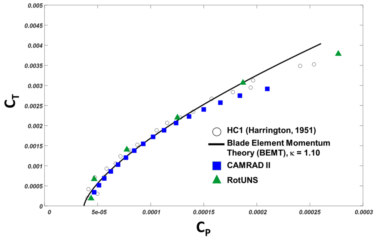
Figure 42. Measured and calculated performance of the single rotor, HS1 [13] in hover.
