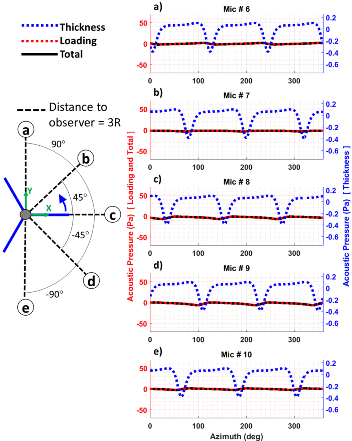
Figure 71. Azimuthal acoustic directivity in hover for single modern rotor acoustic pressure time history. The left (red) y-axis corresponds to loading and total noise, and the right (blue) y-axis corresponds to thickness noise.
