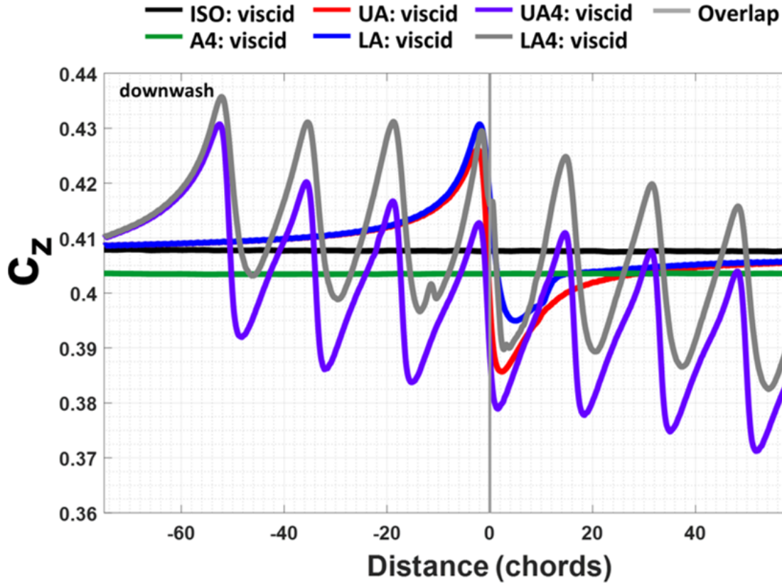
Figure 37. Viscid calculations with downwash for an isolated airfoil, two airfoils crossing, single train of eight airfoils crossing ( A4 ), and two trains of eight airfoils crossing ( UA4 and LA4 ), c_z versus distance to overlap ( M = 0.25 , \alpha = 9.8^\circ , V_i = 31 ft/s, S/c = 4.0 ( S = 2.0 ft, c = 0.5 ft), and D/c = 33.51 ).
