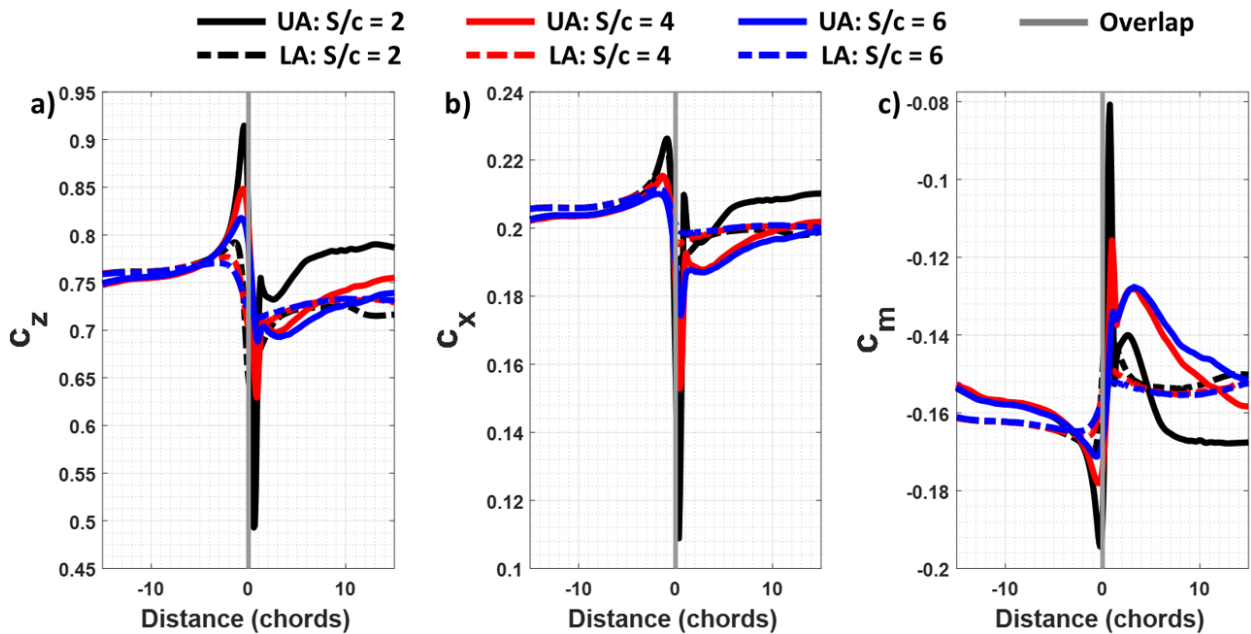
Figure 20. Two NACA 0012 airfoils crossing for a) c_z , b) c_x , and c) c_m versus distance to overlap ( M = 0.9 ( V_{tip} = 1,005 ft/s), \alpha = 7^\circ , and S/c = 2.0, 4.0 , and 6.0 ( c = 0.5 ft)).
