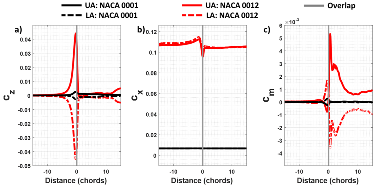
Figure 16. Comparison of two NACA 0001 and NACA 0012 airfoils crossing for a) c_z , b) c_x , and c) c_m versus distance to overlap ( M = 0.9 ( V_{tip} = 1,005 ft/s), \alpha = 0^\circ , and S/c = 4.0 ( S = 2.0 ft, c = 0.5 ft)).
