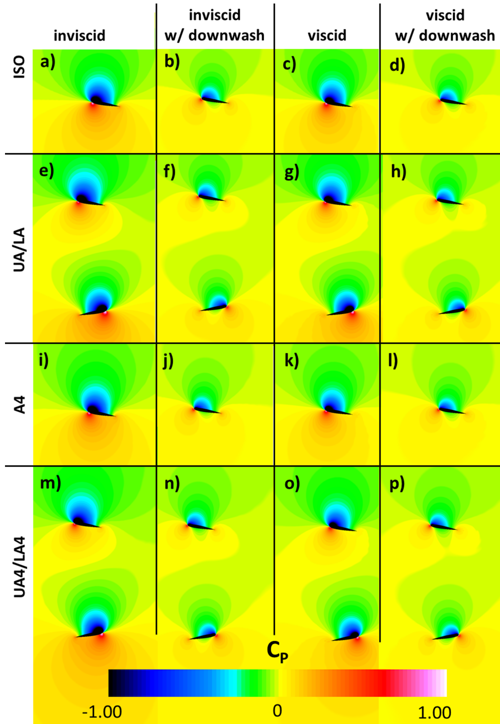
Figure 30. Isolated airfoil, two airfoils crossing at crossing ( UA/LA ), single train of eight airfoils ( A4 ), and two trains of eight airfoils at crossing ( UA4/LA4 ) for an inviscid no downwash (a), e), i), and m)), inviscid with downwash (b), f), j), and n)), viscid no downwash (c), g), k), and o)), and viscid with downwash (d), h), l), and p)), simulation C_p contour ( M = 0.25 ( V_{tip} = 280 ft/s), \alpha = 9.8^\circ , V_i = 31 ft/s, and S/c = 4.0 ( S = 2.0 ft, c = 0.5 ft)).
