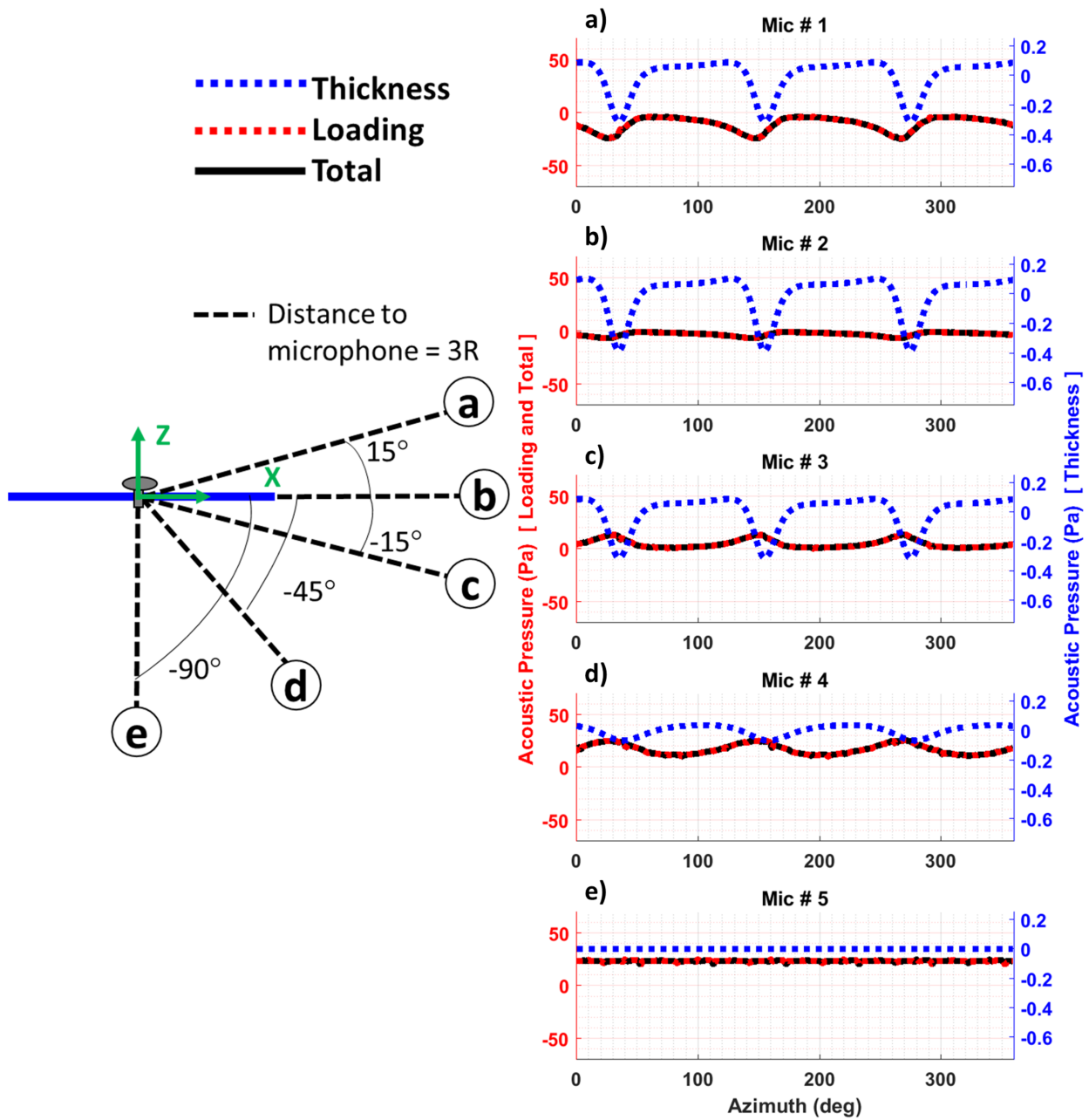
Figure 69. Elevation acoustic directivity in hover for single modern rotor acoustic pressure time history. The left (red) y-axis corresponds to loading and total noise, and the right (blue) y-axis corresponds to thickness noise.
