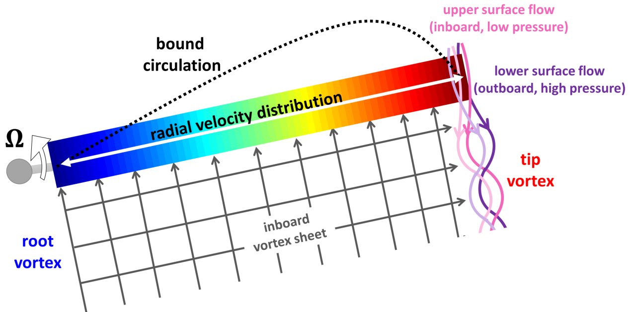
Figure 56. Pictorial representation of a blade tip vortex formation and the trailed and shed vorticity in wake.
