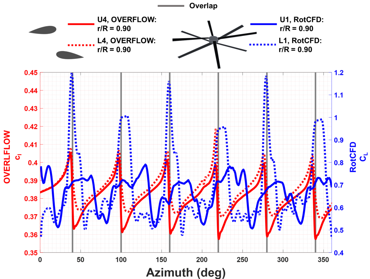
Figure 53. Comparison between OVERFLOW 2D and 3D RotCFD coaxial modern rotor in hover at r/R = 0.90 for upper rotor blade one (U1), lower rotor blade one (L1), upper airfoil four (UA4), and lower airfoil four (LA4) (OVERFLOW conditions: M = 0.564 , \alpha = 5.8^\circ , S/c = 4.0 ( S = 2.0 ft, c = 0.5 ft), and D/c = 75.4 ft, RotCFD conditions: V_{tip} = 700 ft/s), \alpha = 5^\circ , and S/c = 4.0 ( S = 2.0 ft, c = 0.5 ft), C_T = 0.004 , C_P = 0.0003 , \theta_U / \theta_L = 9^\circ ).
