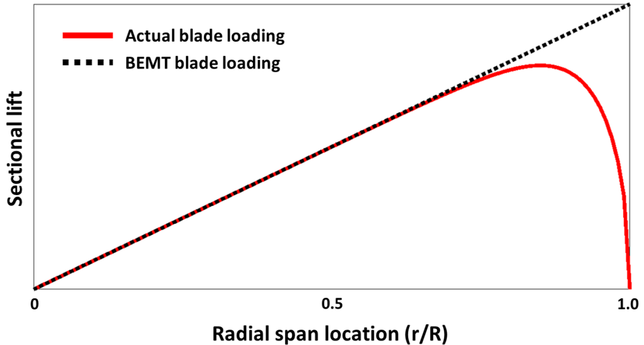
Figure 65. Rotor blade loading with and without tip loss.
