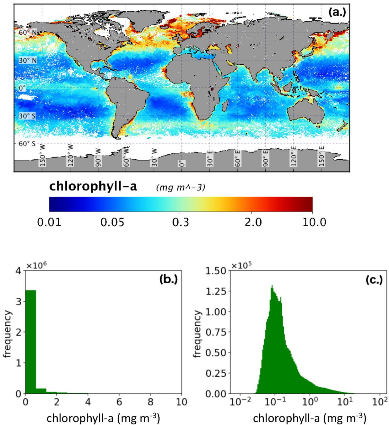
Figure 2: (a.) SeaWiFS chlorophyll-a concentration for May 1998. Subplots (b.) and (c.) show how global chlorophyll-a concentration for May 1998 is nearly log-normally distributed.
