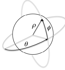
FIGURE 1. Spherical coordinates.
