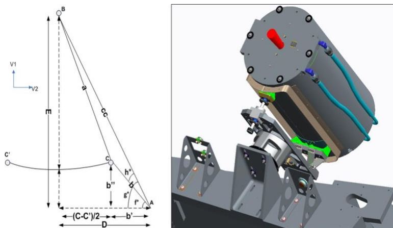
Figure 6. The PM-to-COCOA axial distance geometry and the ADMA.
