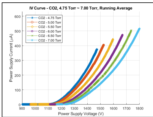
Figure 4 – IV curve data in carbon dioxide for a 7.13 cm tube 100 µm wire
