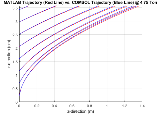
Figure 1 – Preliminary COMSOL and MATLAB analysis with estimated particle charge on a 1 μm diameter particle
