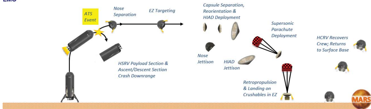
Figure 15. Concept of operation illustrating Mars ascent ATS targeting a RTEZ using the capsule aeroentry and landing systems.
