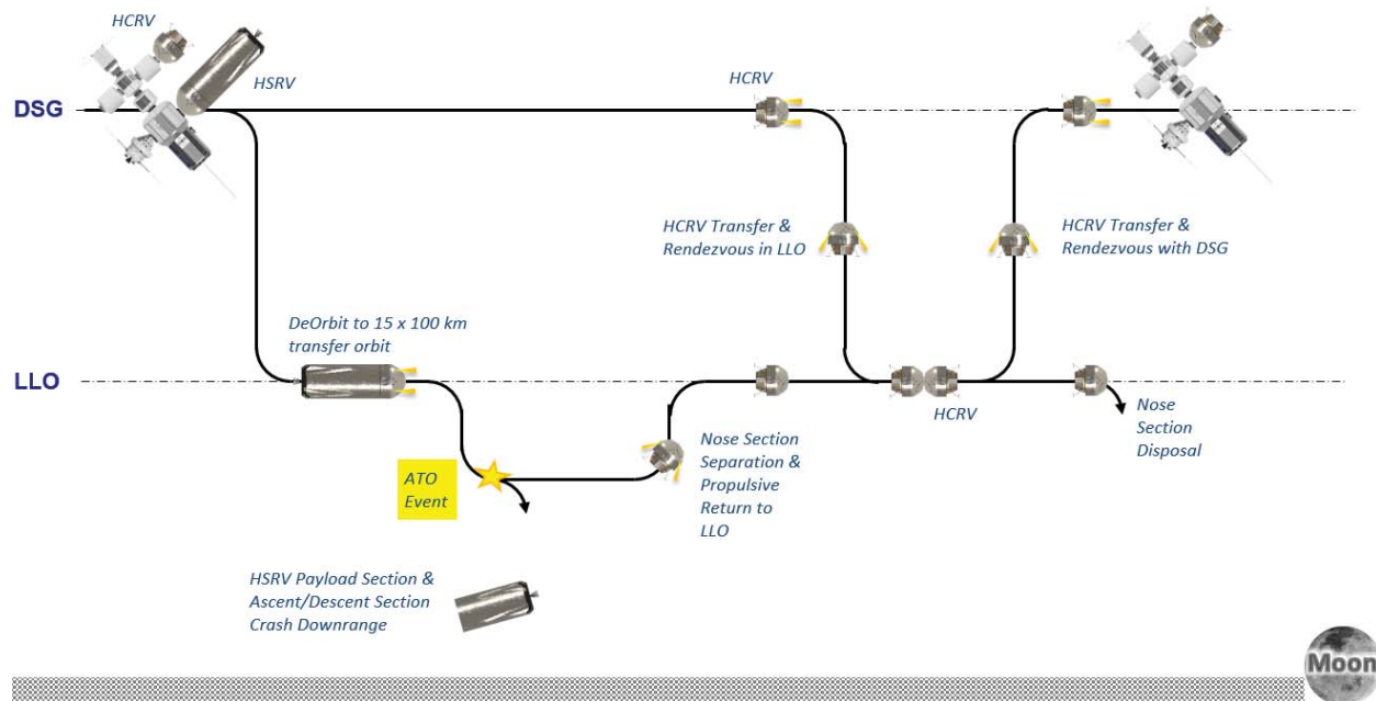
Figure 33. Concept of operation illustrating Lunar descent ATO using the ATLS propulsion capabilities only.
