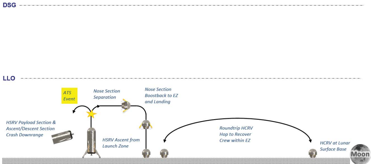
Figure 39. Concept of operation illustrating Lunar ascent ATS targeting the RTEZ using the ATLS propulsion capabilities only.
