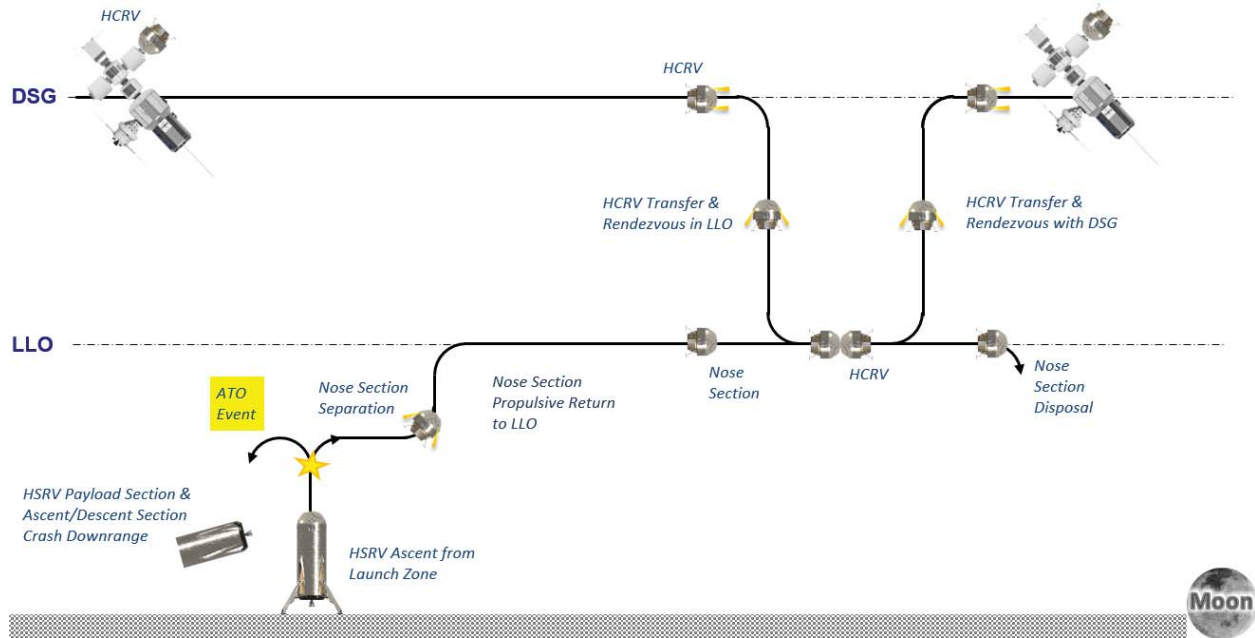
Figure 41. Concept of operation illustrating Lunar ascent ATO using the ATLS propulsion capabilities only.
