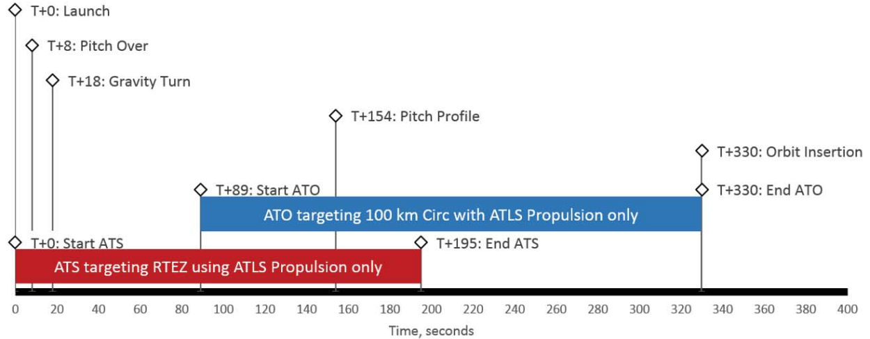
Figure 38. Lunar ascent abort options.
