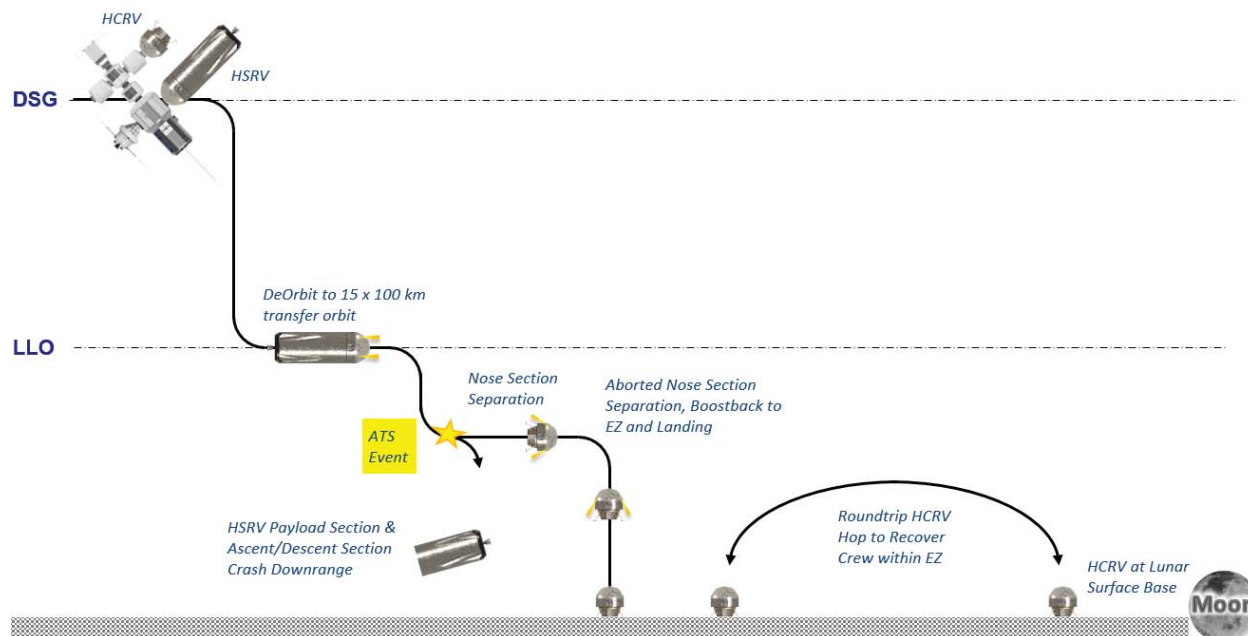
Figure 35. Concept of operation illustrating Lunar descent ATS targeting the RTEZ using the ATLS propulsion capabilities only.
