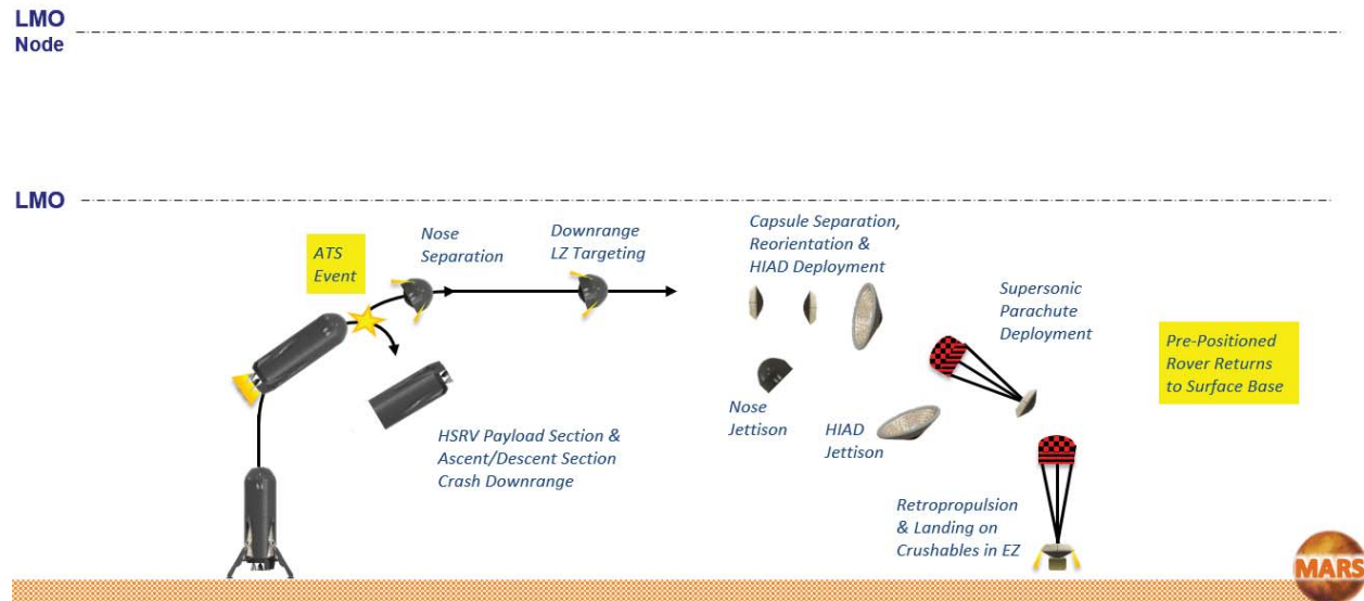
Figure 17. Concept of operation illustrating Mars ascent ATS targeting a common downrange location approximately 500 km east of the launch site using the capsule aeroentry and landing capabilities.
