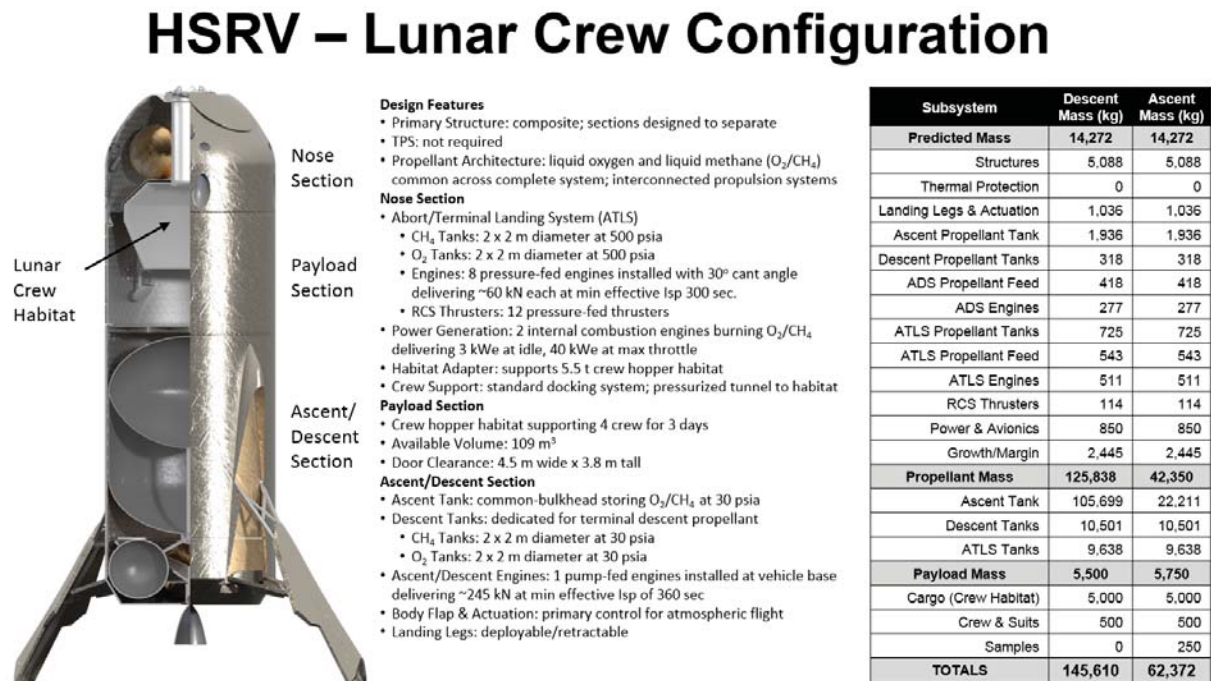
Figure 6. Summary of the HSRV configuration used for lunar crewed flights.
