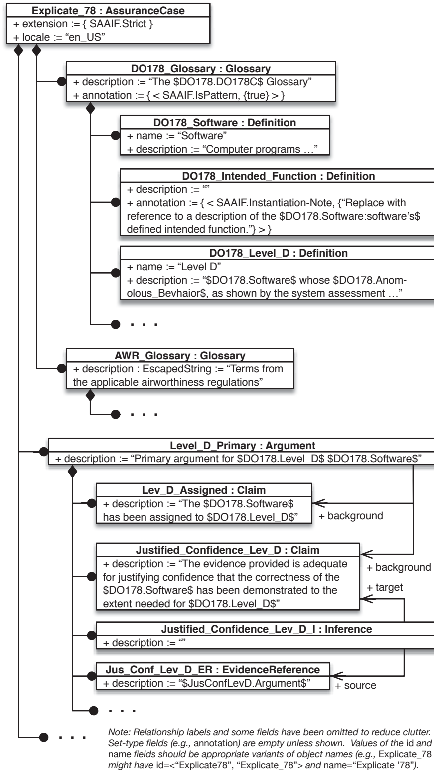
Figure D2: Adaptation of “Level D primary argument” from [23] (part 1 of 3).
