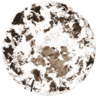
Sham (0Gy)
