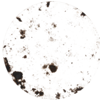
^{56}\text{Fe} (2Gy)
