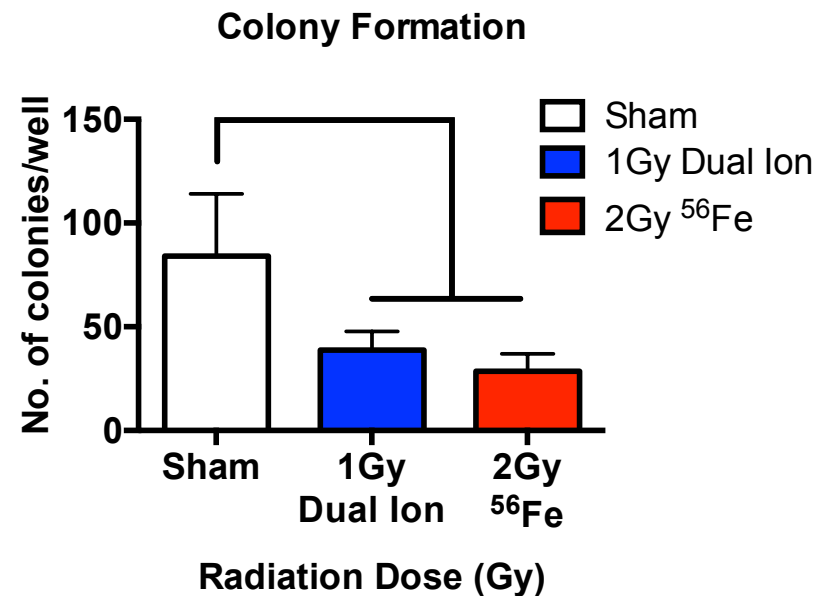
^{56}\text{Fe} (2Gy)
