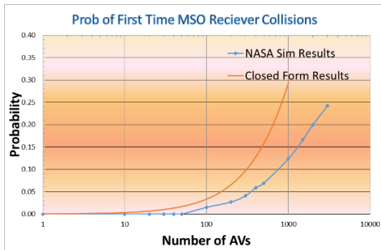
Figure 11 – Probability of First Time MSO Receiver Collisions
