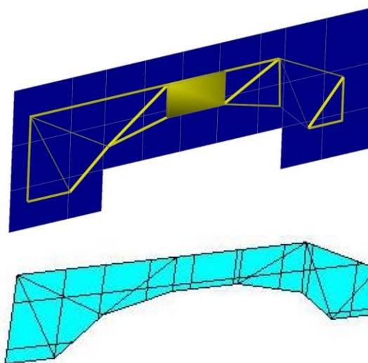
Figure 3. Avoidable Cutting Operation: The resultant shape was accomplished with 10 copies of the blue structure and 9 triangular prism and 1 box cutting operations. This would have been better accomplished using quadrilaterals and triangles if needing conversion
