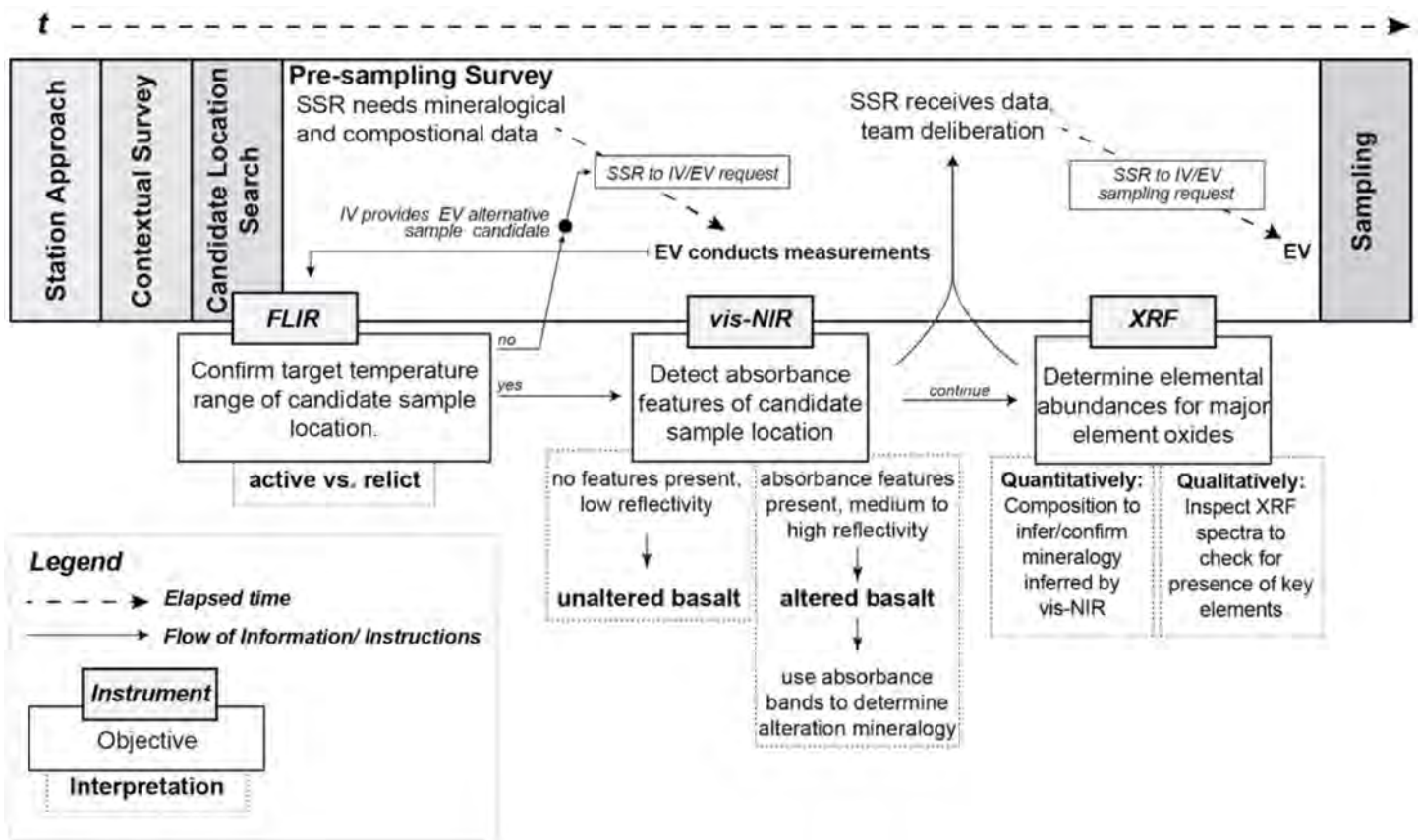
Figure 4. Integration of instruments into EVA architecture.
