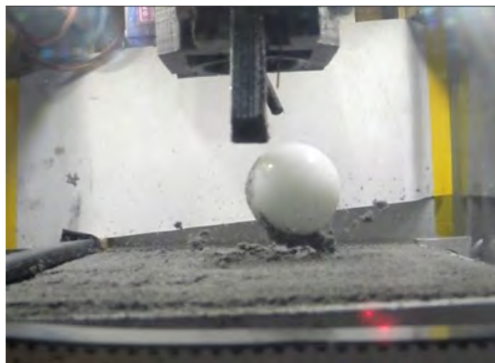
Impact clumping in microgravity showing strong cohesion in fine simulant.
