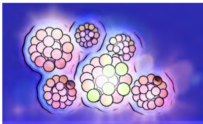
Figure 1.1. Visualization of light scattering by particles in clusters and the close packing of the clusters themselves. Mutual influence among the clusters is depicted.
