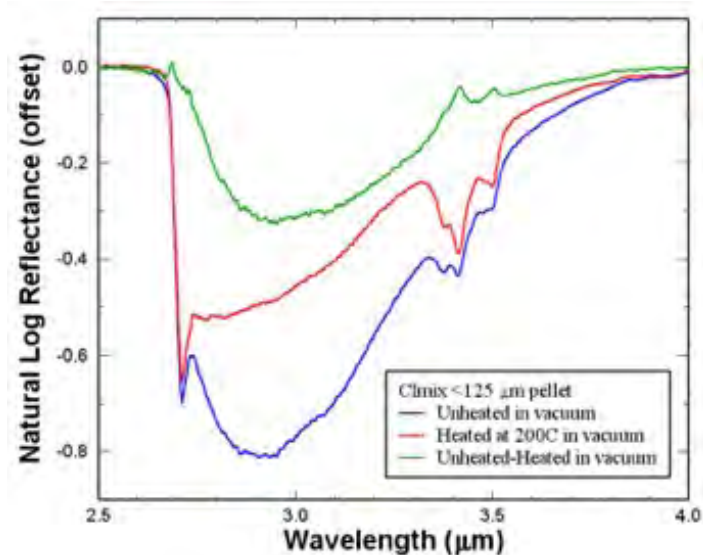
Spectra of CI meteorites (Clmix) measured in vacuum. Blue= unheated. Red= heated to 200°C. The Green spectrum is the ratio of the two and captures the character of the loosely bound adsorbed water for this sample.
