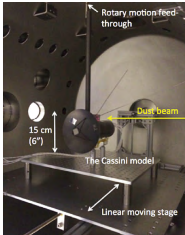
1:20 scaled model of the Cassini spacecraft exposed to dust impacts to study how sensitive antennas are to impact plasmas.
