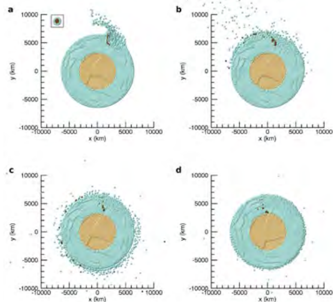
Figure 2: Projectile's core interaction during large terrestrial collisions. Panels (a)-(d) show four time steps in an SPH simulation (at 0.2, 1, 2.7 and 23 hr), with impactor mass M_i = 0.001 M_\oplus , (~1400 km diameter projectile), 45^\circ impact angle, and impact velocity of 18 km/s. Green particles represent silicate material (Earth and projectile), light brown particles indicate Earth's core, and dark brown particles indicate the projectile's core. The projectile size is shown for reference in the top-left corner of (a).
