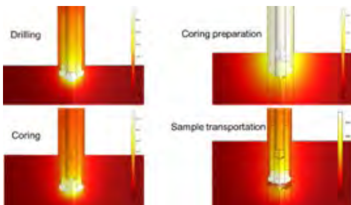
Energy Exchange Model EEM simulation results: temperature distribution during drilling in marble.
