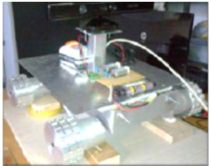
Lunar rover operating at Moon simulant facility
