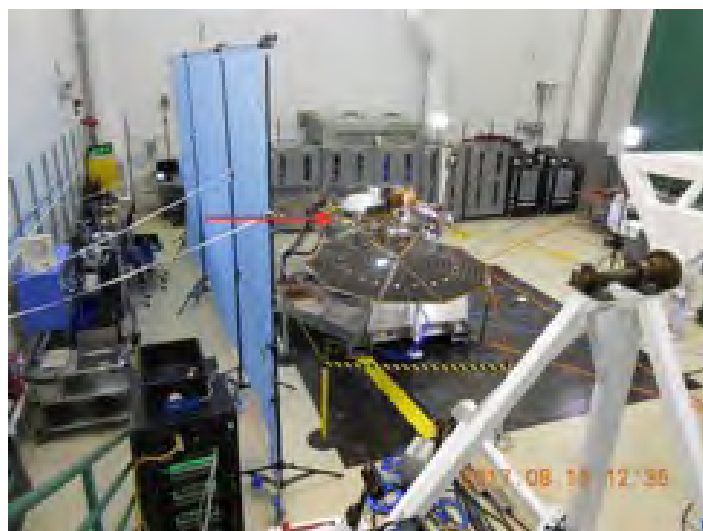
Red arrow pinpoints the position of the microreflector on board InSight probe
