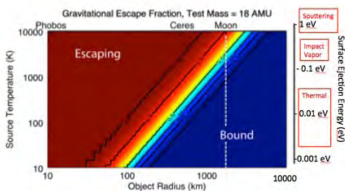
Figure 1.2.1 – Gravitational escape fraction for water as a function of airless body size [Killen et al., 2017]
