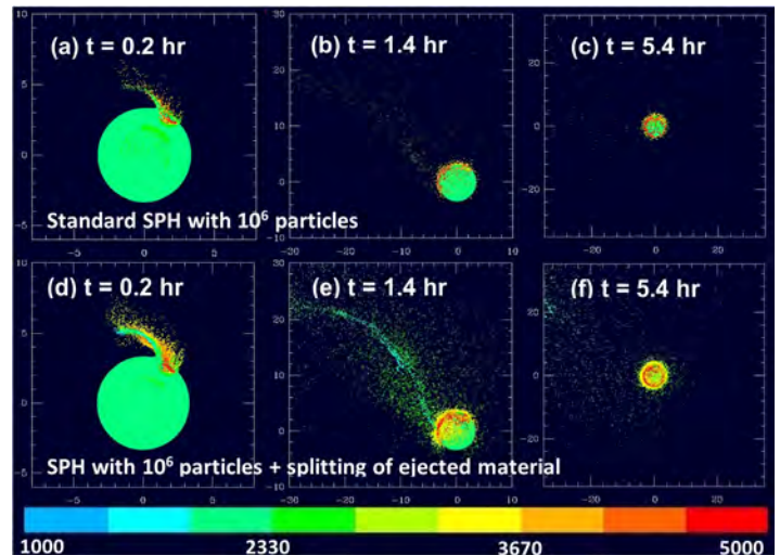
Figure 1: Simulations of the impact of a Vesta-mass body ( 5 \times 10^{-4} M_M ) with Mars. The impact velocity is 1.5 v_{esc} ( 7 \text{ km s}^{-1} ), at a 45^\circ impact angle. Color scales with temperature in Kelvin; distances shown in units of 10^3 \text{ km} . (Top row) A 10^6 -particle simulation with standard SPH. (Bottom row) The same impact modeled with SPH + particle splitting and an order-of-magnitude higher resolution of the ejected material. After 10 hr, the disk mass is 8.5 \times 10^{-6} M_M , with \sim 2 M_{pd} having equivalent circular orbits at and beyond \sim 5 R_M , consistent with subsequent accumulation of Phobos and Deimos in the 5 to 7 R_M region. Outer disk material is 85% martian in origin. From Canup & Salmon (2018).
