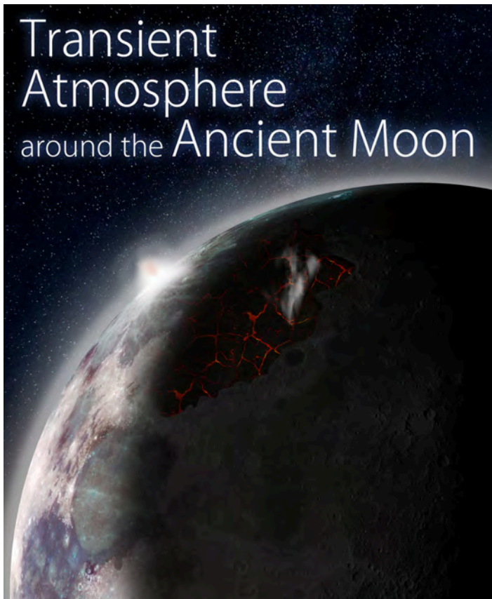
Figure 1. Volcanic eruptions long ago created a transient atmosphere around the Moon that may have been an important source of volatiles suspected to be trapped within polar deposits. Illustration credit: MSFC and LPI.
