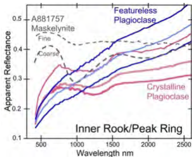
M 3 spectra of crystalline and 'featureless' plagioclase found along the Orientale Inner Rook mountains. Shown for comparison are offset laboratory spectra of a maskelynite separate from the gabbroic lunar meteorite A881757.
