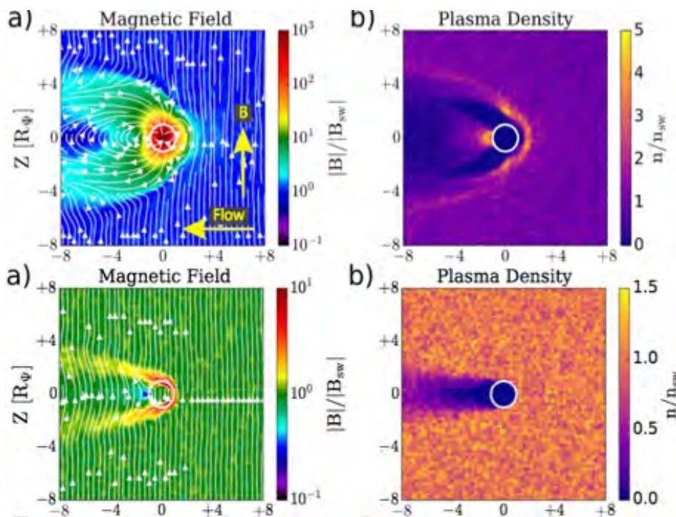
Figure 1.1.1 Predicted magnetic field and plasma density at 16 Psyche for magnetized (top) and unmagnetized (bottom) cases.
