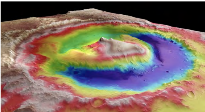
Digital Terrain Model of Gale Crater by the High Resolution Stereo Camera (HRSC) on the ESA Mission Mars Express. ESA/DLR/FU Berlin.
