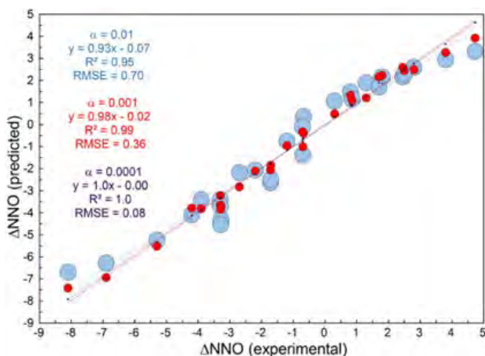
Figure 1.6. Predicted vs. experimental oxygen fugacity using XAS data.
