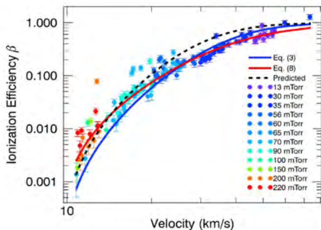
Ionization efficiency for aluminum and air extended to the full velocity range of interest. From [SSSERVI-2017-098].
