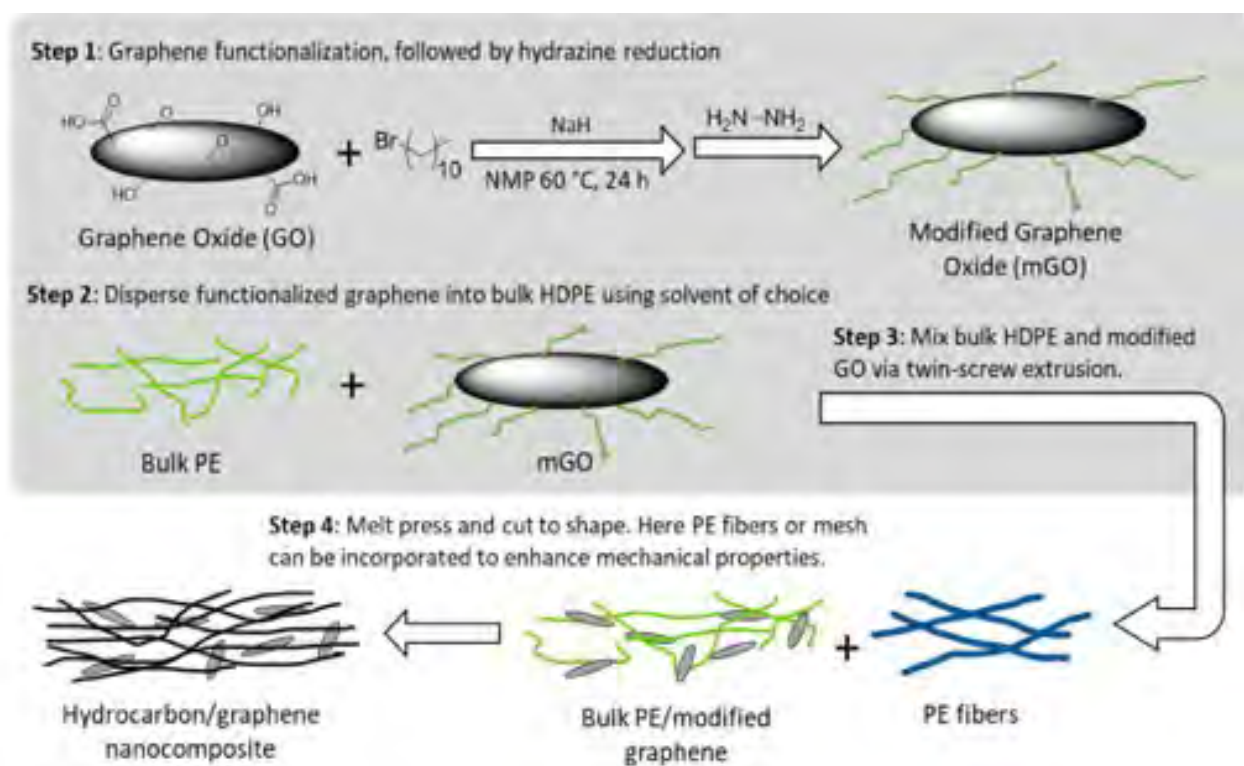
Figure 7: Process for forming and testing polyethylene fiber reinforced graphene: polymer nanocomposites as spacesuit patches with electrical conductivity, thermal conductivity, and radiation hardness.
