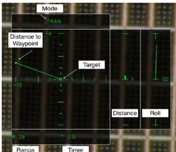
Figure 9. Proposed in-helmet display for EVA navigation and real-time radiation exposure monitoring.
