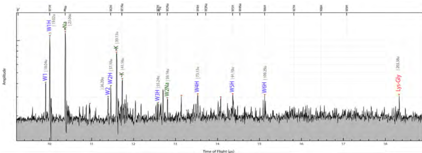
Time-of-flight mass spectrum produced by a single 4.8 km/s iron impactor into a flash-frozen Lysine-Glycine mixture.
