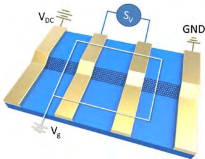
Figure 8: Nanoribbon graphene FET device. (O. Vail et al., manuscript in preparation)
