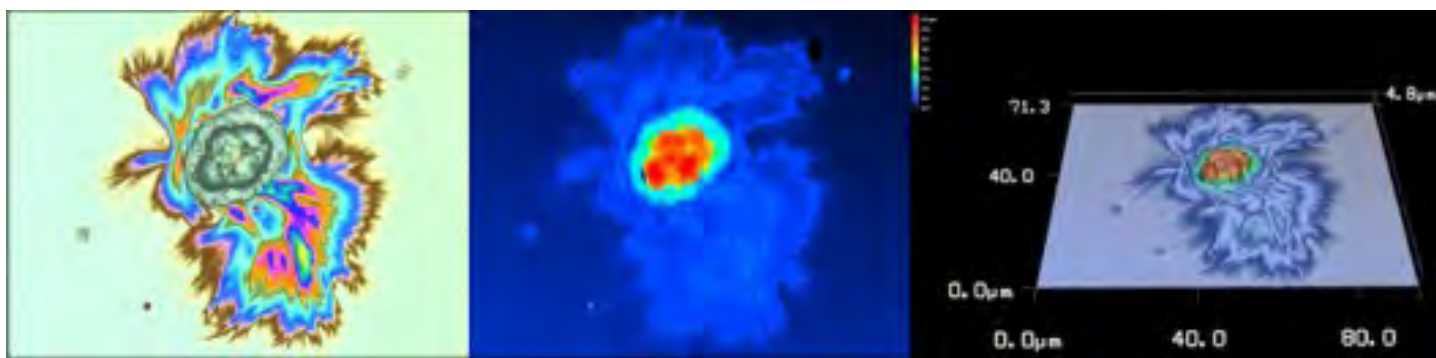
Figure 5: Combination of optical and laser contrast images of bombarded samples. Height image; tilted 3D view. A spherical Cu-particle embedded in an olivine with San-Carlos-like composition. Note the shape and extent of the lateral damage induced upon impact around the particle which also reflects in an uplifted surface area of a few nanometers. (Figure: K. Fiege, et al., submitted to J. Geophys. Res. and Guglielmino (Ph.D. thesis 2017)).
