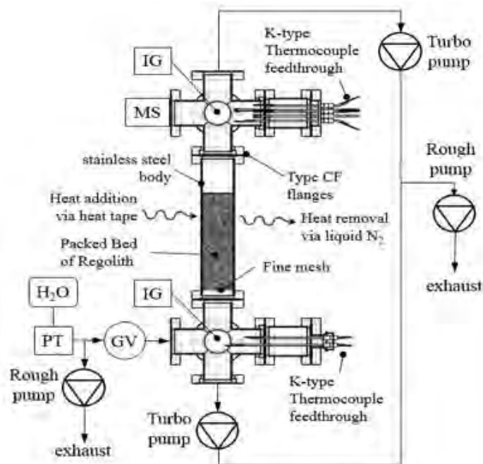
Figure 6: Instrumentation schematic of the packed bed vacuum chamber. PT refers to pressure transducer, GV to gate valve, IG to ion gauge, and MS to mass spectrometer.
