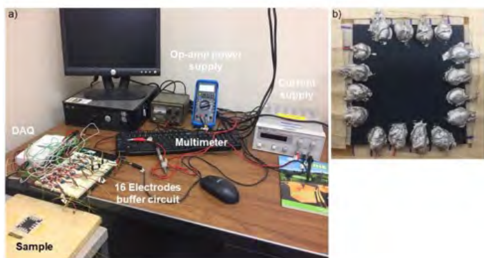
Figure 10: a) Experimental setup for electrical resistance tomography tests on b) samples produced at Sapienza University, and tested at UC Davis.
