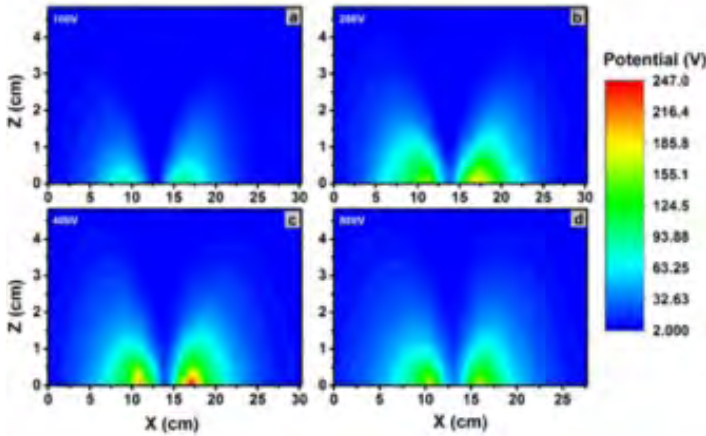
Measured potential contours above an insulating surface embedded in a vertical magnetic dipole field with the impact of the 100, 200, 400 and 800 eV plasma flow generated in CSWE.
