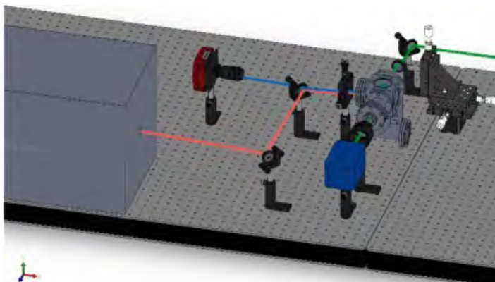
Figure 4: Schematic of laser induced micro-particle accelerator to simulate hypervelocity impacts.
