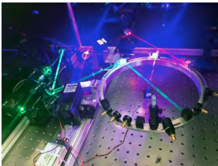
Fig. 2: First illumination of GraVeTAS aperture in full three beam mode. Each beam is encoded with an orthogonal array of fringes generated by novel miniaturized laser interferometers.
