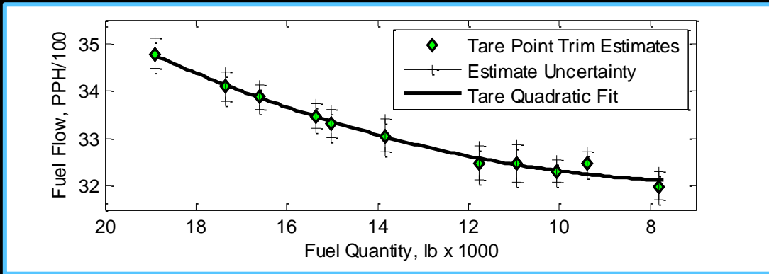
tare fuel flow vs. fuel quantity
