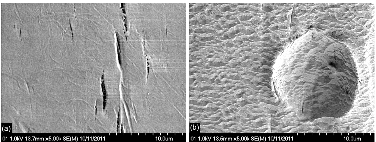
Figure 9.—FESEM images of MISSE-7 Orthofabric at 5000 \times showing (a) the lack of texture in the protected area and (b) the texture in the exposed area. The 10 \mu\text{m} crater shown in (b) was the result of a debris strike prior to erosion texturing.
