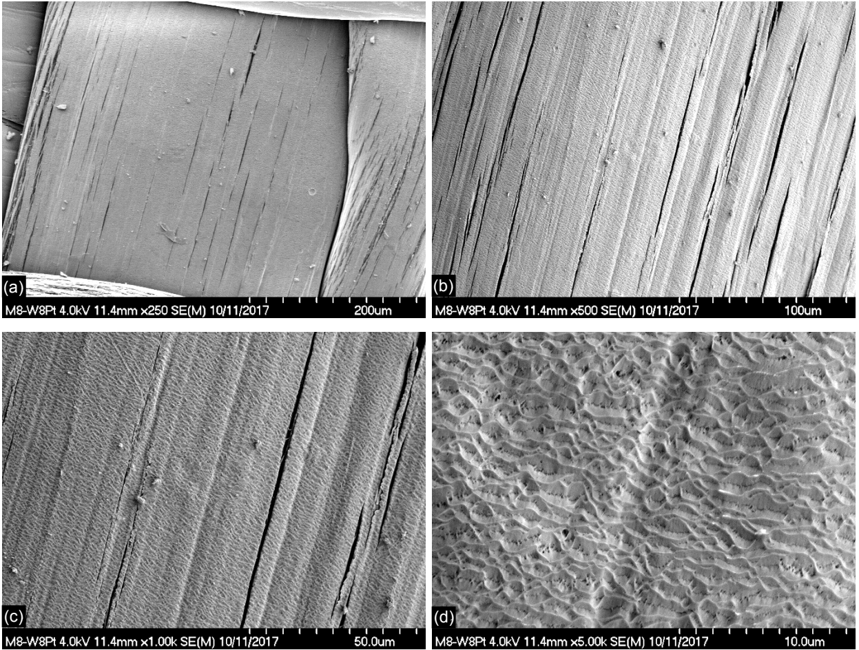
Figure 8.—FESEM images of exposed Orthofabric at (a) 250 \times , (b) 500 \times , (c) 1000 \times , and (d) 5000 \times .
