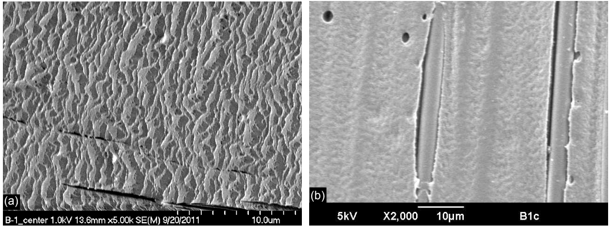
Figure 6.—FESEM images of exposed MISSE-7 Apollo FEP spacesuit fabric at (a) 5000×, and ORU β-cloth at (b) 2000× show texture similar to that observed in the ORMate-III samples.
