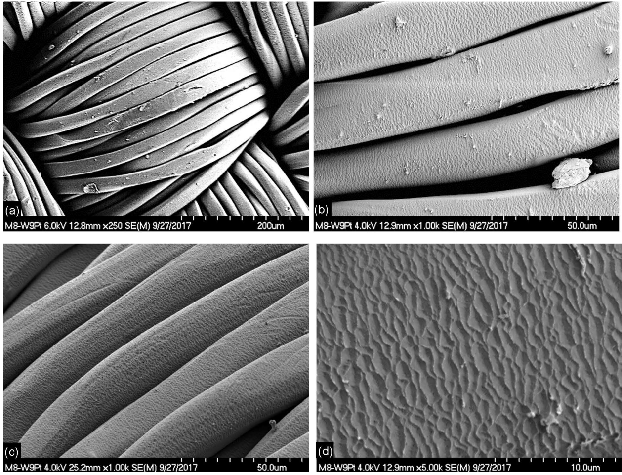
Figure 5.—FESEM images of exposed ORMate-III Apollo FEP fabric at (a) 250×, (b, c) 1000×, and (d) 5000×.
