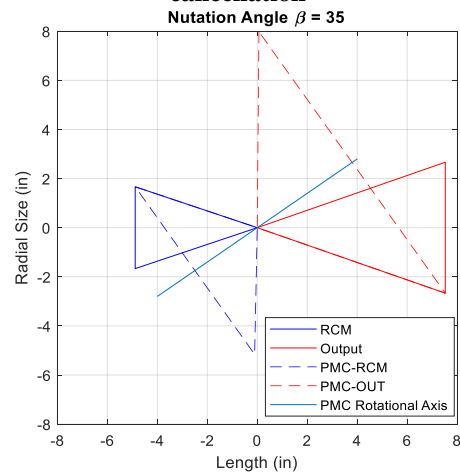
Figure 9. Example PMC geometry at high nutation angle and high difference in meshing gear tooth numbers
