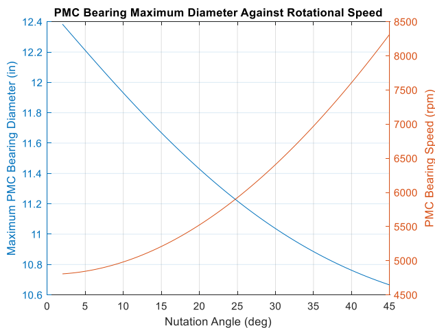
Figure 18. PMC bearing maximum diameter possible for given geometry along with bearing speed
