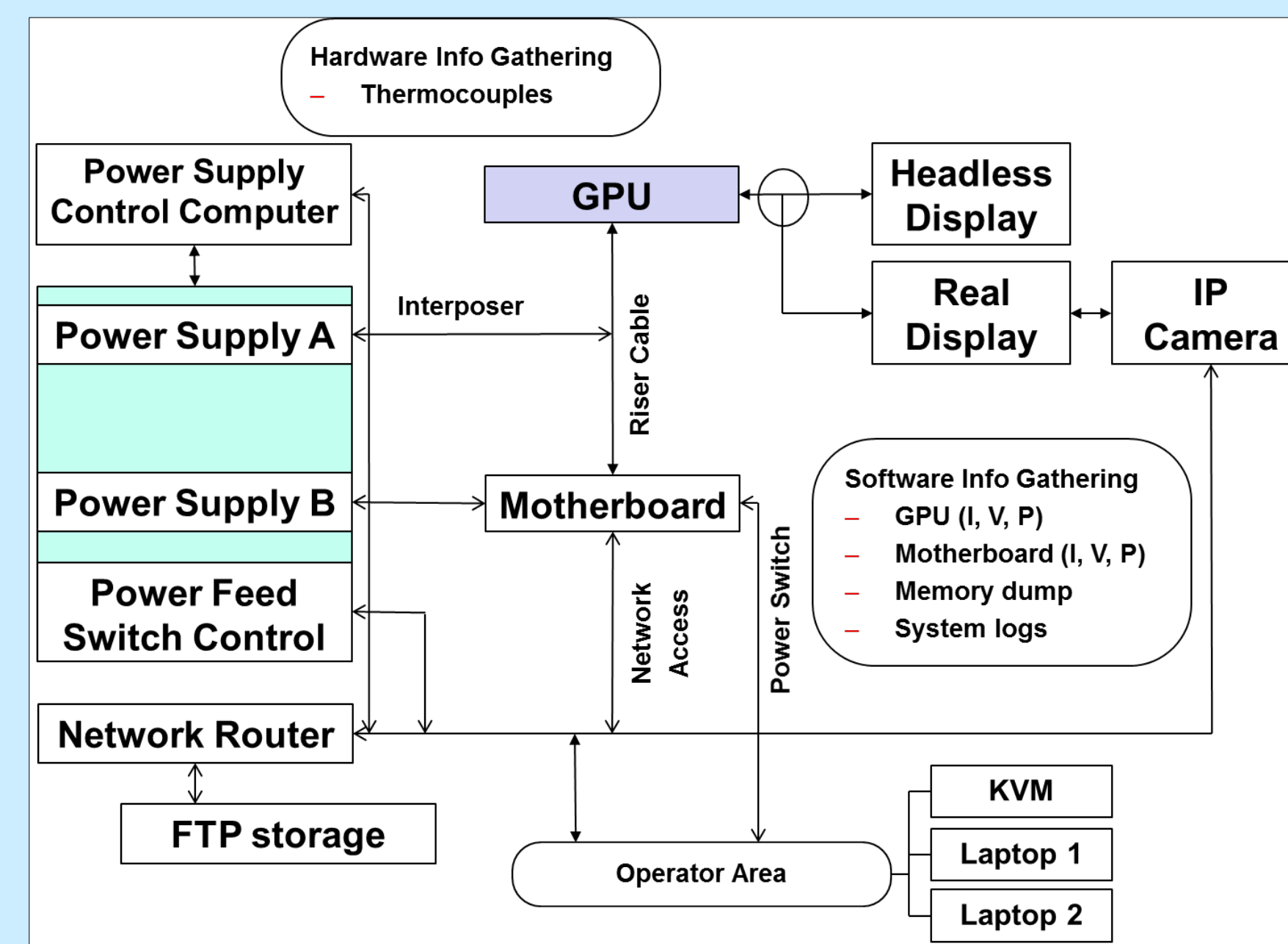
Figure 6: System-Level Organization
