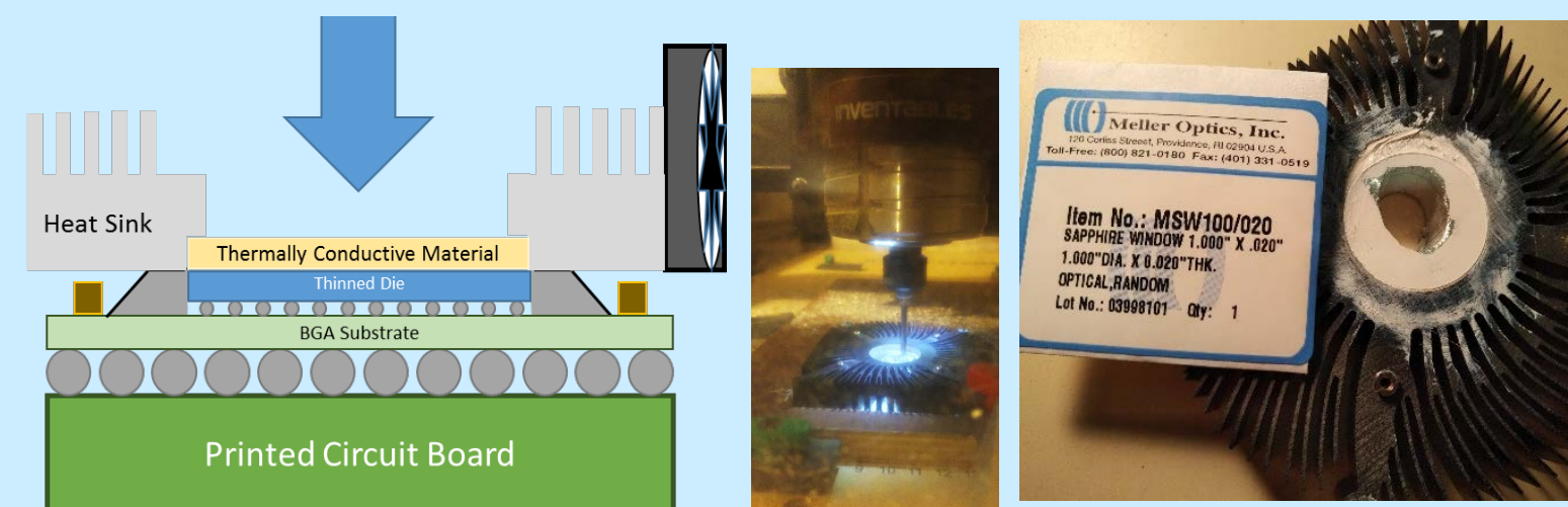
Figure 2: Obverse Side Modifications Sapphire window design (left); Milling COTs heatsink (center); Final product (right)
