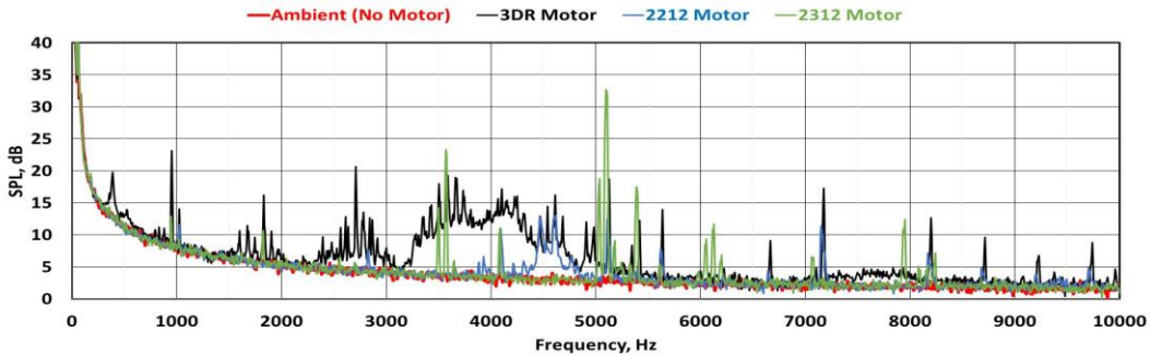
Figure 6. Background noise and motor only SPL comparisons for three motors, microphone 9 on medium array, 4380 RPM.
