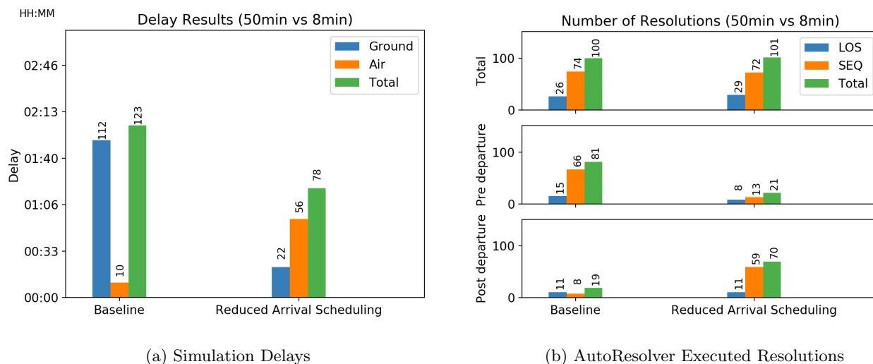
Figure 12: AutoResolver Simulation Detection and Resolution Results: Baseline (0.3nmi H, 100ft V, 60s, 50min) vs Reduced Arrival Scheduling Horizon (0.3nmi H, 100ft V, 60s, 8min)
