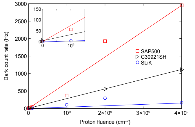
FIG. 12: Dark count rates of three different APD models at various radiation fluences at -86^\circ\text{C} [52]. Each data point is an average between the two samples tested. Linear fit lines pass through the first and last data points. The dark count rate increase appears to be linearly proportional to the proton fluence. Inset is a close-up of the first points.
