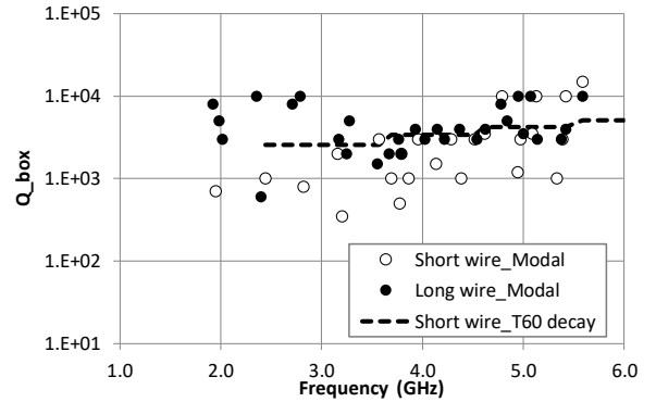
Fig. 9 Modal Q of the closed box, measured with short and long wire antenna; compared with T60 time decay result.
