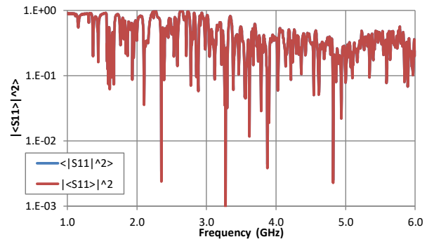
Fig. 8 S_{11} of the long wire antenna, measured in the box enclosure with aperture AP2.
