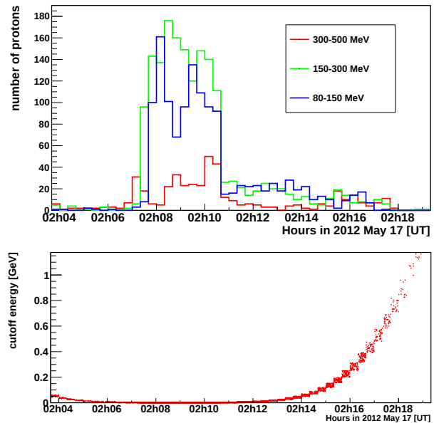
Fig. 1: In the top figure an increase in number of protons detected by PAMELA during 2012 May 17 GLE: three intervals of kinetic energies are reported. From the bottom figure it is evident that cut-off energies were always below considered kinetic energies for protons.
