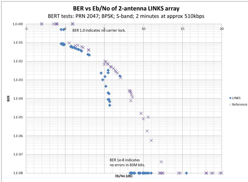
Figure 6 BER vs Eb/No chart of ATLAS LINKS for S-band Coded Downlink
